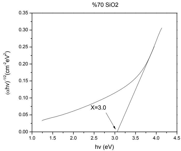
Figure 9.22: Indirect band gap calculation of PS coatings with %70 SiO 2 content using Tauc method.
