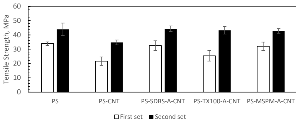
Figure 4.5. Tensile strength values of the binary composites.
