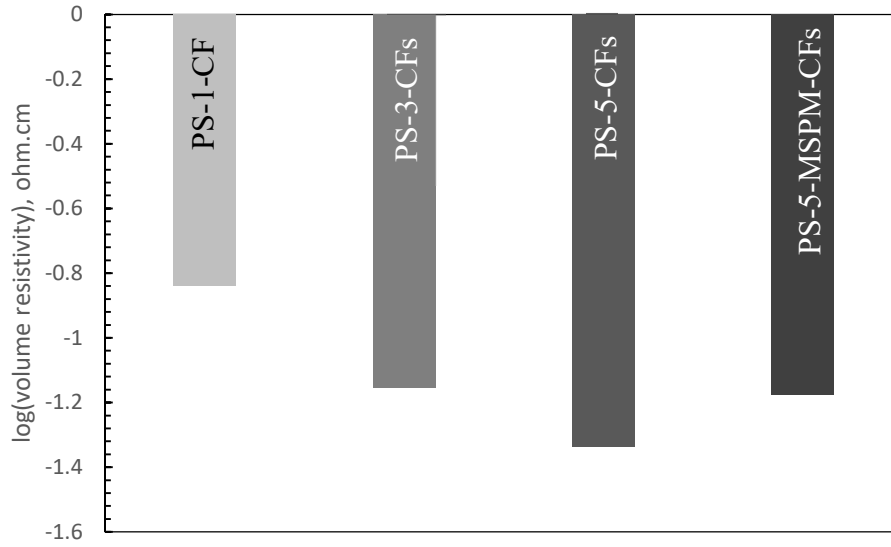
Figure 4.47. Electrical resistivities of the multilayer composites.
