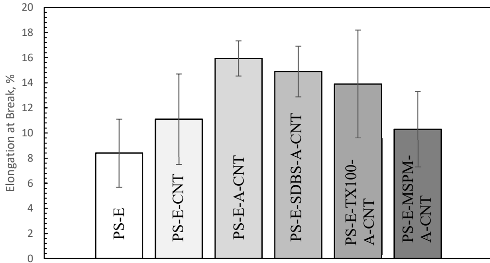
Figure 4.18. Elongation at breaks of the ternary composites.
