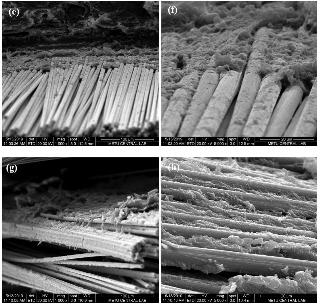
Figure 4.42. (cont'd) SEM images of the fracture surfaces of the multilayer composites; (a), (b) PS-1-CF, (c), (d) PS-3-CFs, (e), (f) PS-5-CFs and (g), (h) PS-5-MSPM-CFs at 1000x and at 5000x magnification, respectively.
