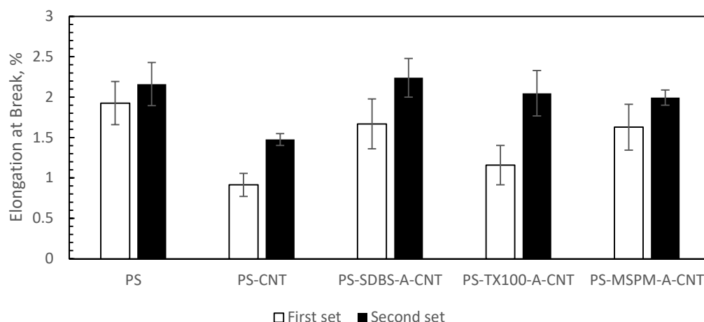
Figure 4.7. Elongation at break values of the binary composites.
