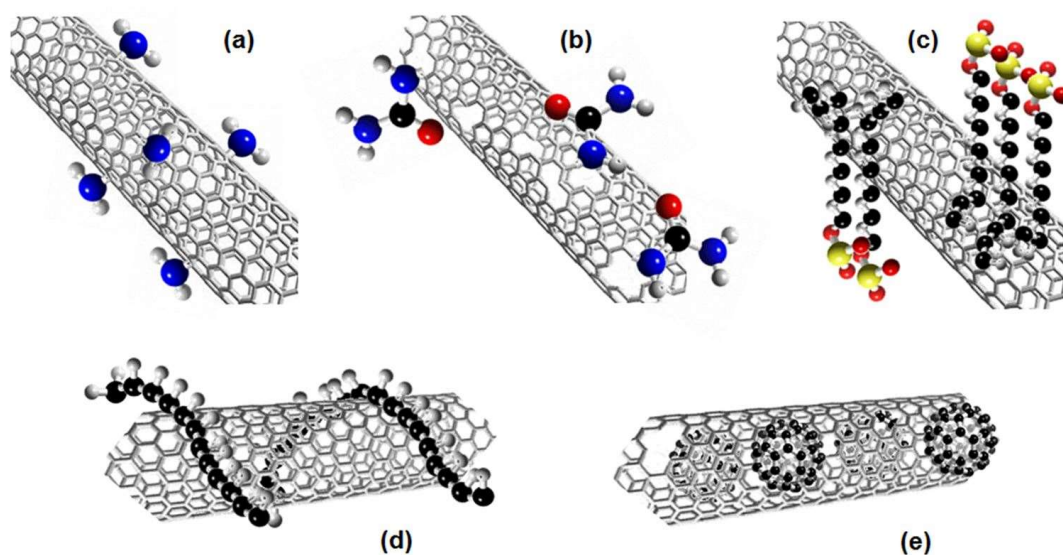
Figure 2.1. Surface modification methods of CNTs (a) covalent sidewall functionalization, (b) covalent defect sidewall functionalization, (c) non-covalent adsorption of surfactants, (d) polymer wrapping, (e) endohedral functionalization with C60 (Ávila-Orta et al., 2013).
