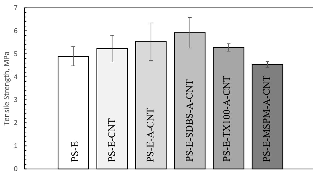
Figure 4.16. Tensile strengths of the ternary composites.
