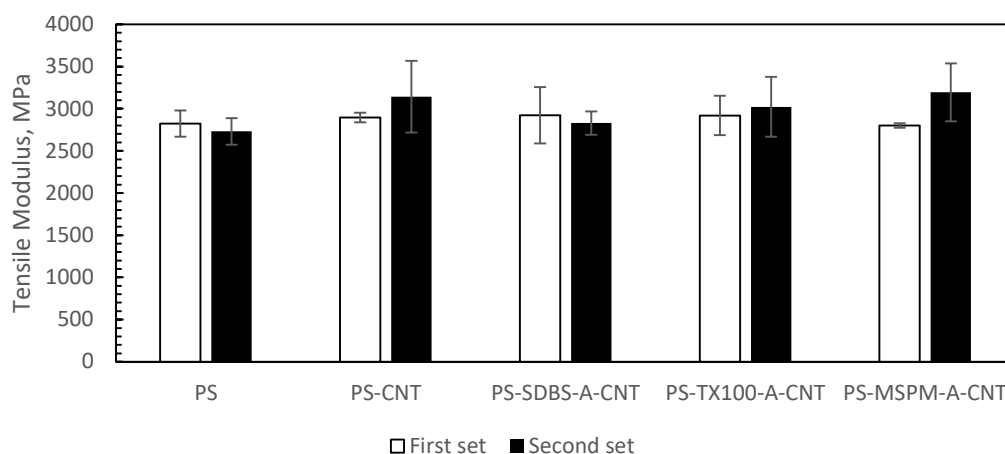
Figure 4.6. Tensile moduli of the binary composites.
