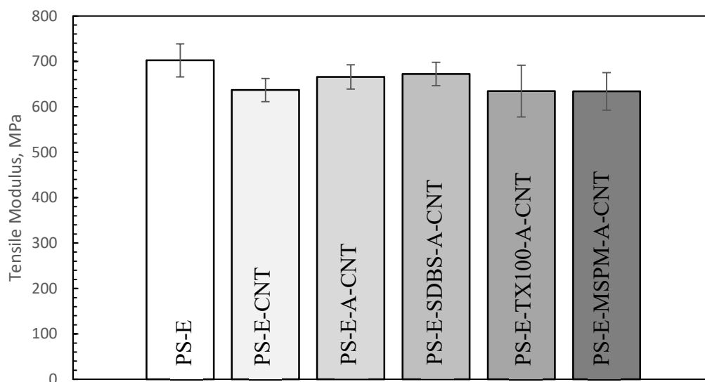
Figure 4.17. Tensile moduli of the ternary composites.
