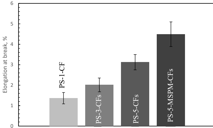
Figure 4.46. Elongation at breaks of the multilayer composites.
