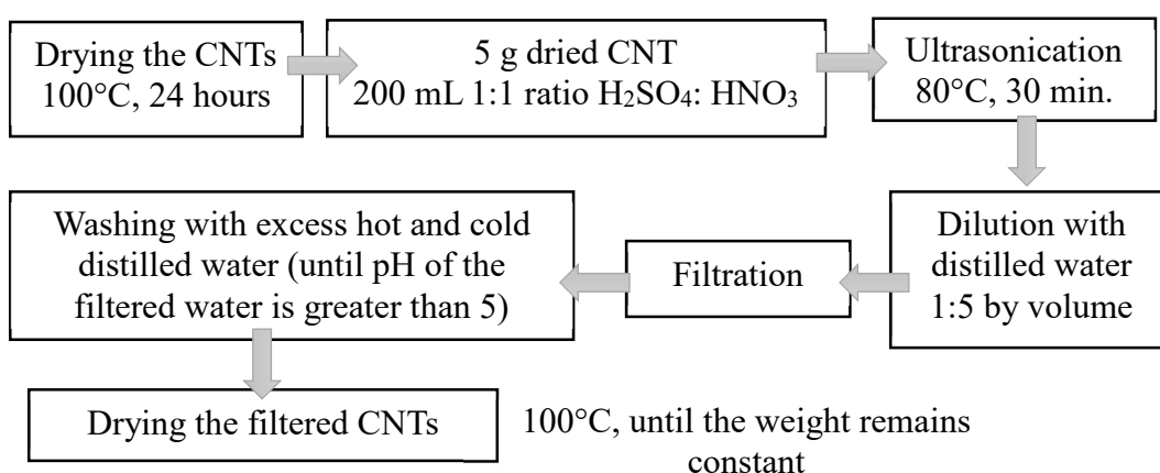
Figure 3.5. Flow chart of preparation steps of A-CNT sample.
