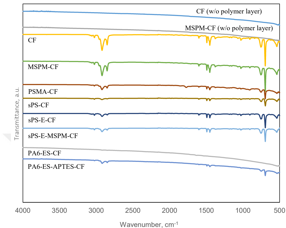
Figure 4.38. FTIR spectra of CF side of the peeled surfaces after T-peel test.
