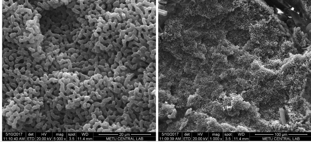
Figure 4.11. PS-E sample from fracture surface at 5000x and 1000x (etched with n-heptane).
