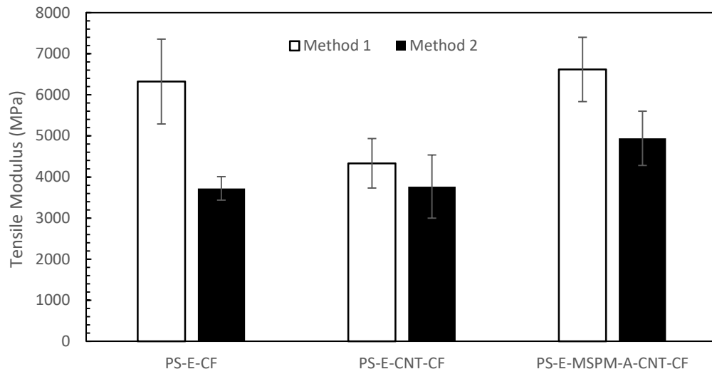
Figure 4.28. Tensile moduli of the multilayer composites.
