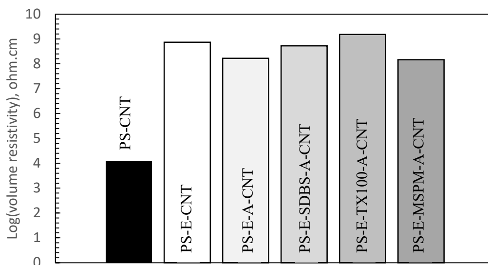
Figure 4.15. Electrical resistivities of the ternary composites.
