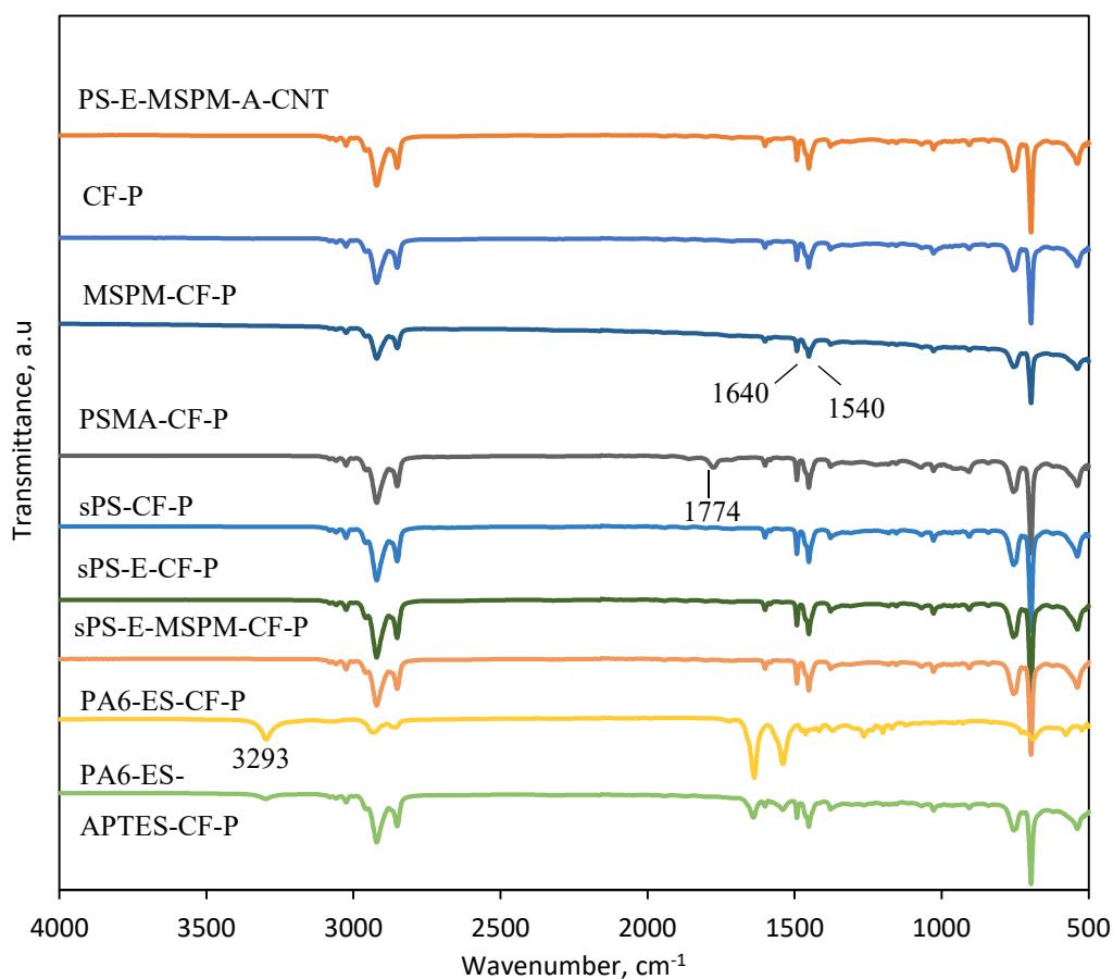
Figure 4.37. FTIR spectra of the polymer side of peeled surfaces after T-peel test.
