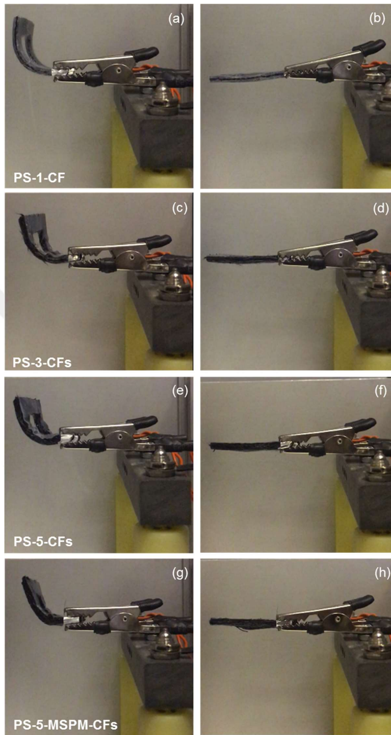
Figure 4.48. Electrically bending test images of the multilayer composites at the beginning of the test and after the recovery; (a), (b) PS-1-CF, (c), (d) PS-3-CFs, (e), (f) PS-5-CFs and (g),(h) PS-5-MSPM-CFs.
