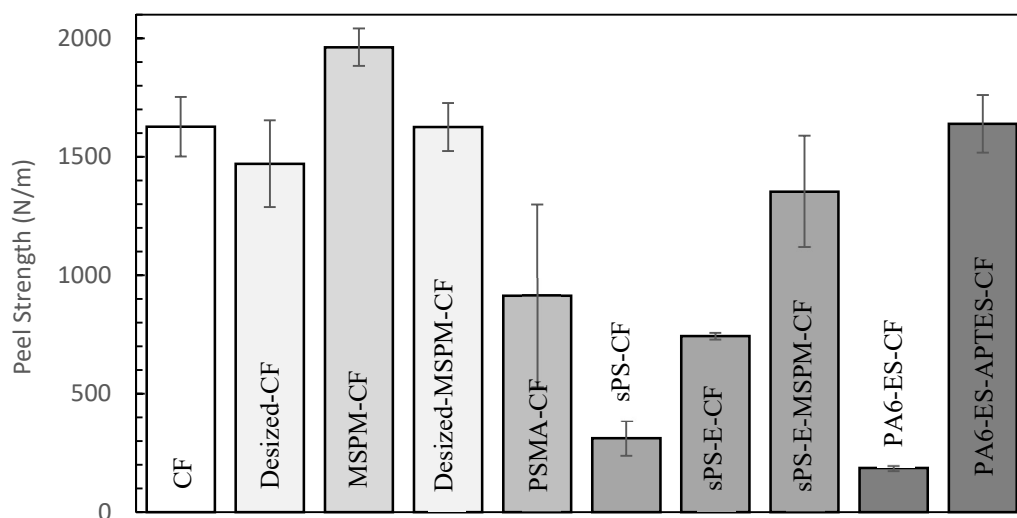
Figure 4.41. Peel strength dependence on different surface modifications applied to CF.
