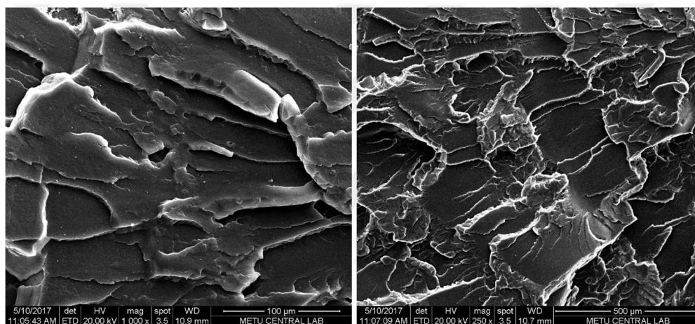
Figure 4.10. Neat PS sample from fracture surface at 1000x and 250x (etched with n-heptane).
