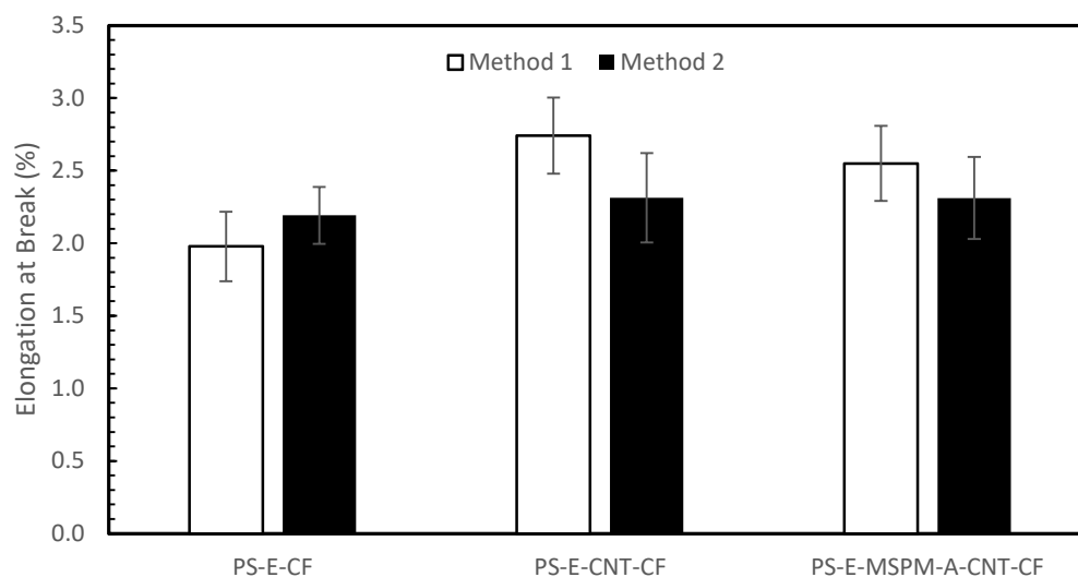
Figure 4.29. Elongation at breaks of the multilayer composites.
