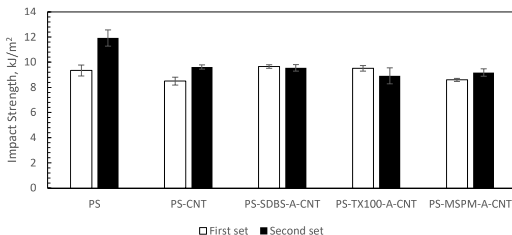
Figure 4.8. Impact strength values of the binary composites for surface modifier selection.
