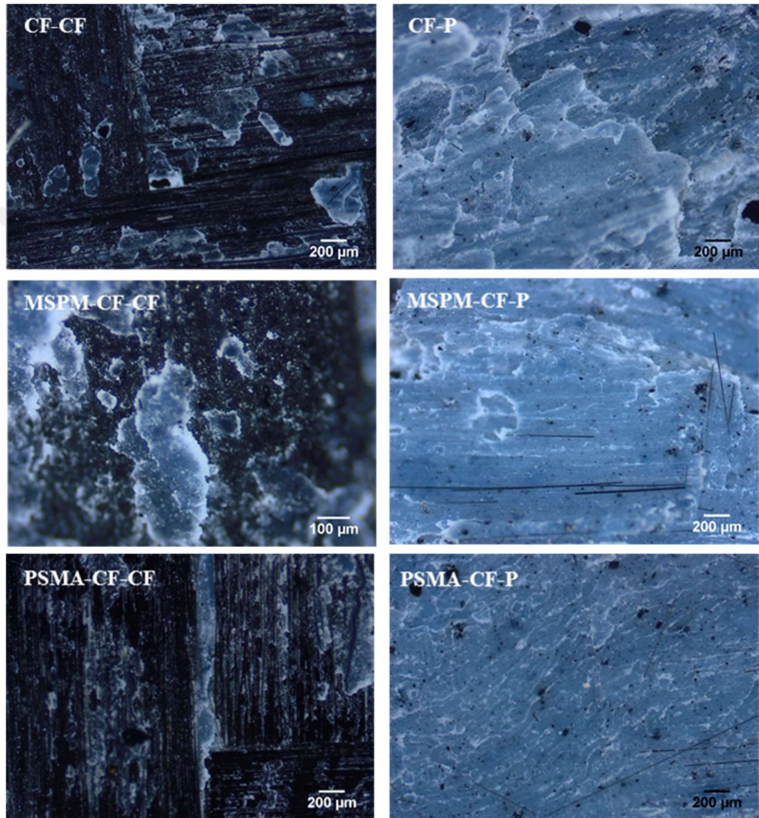
Figure 4.34. Micrographs of peeled surfaces of T-peel test specimens.
