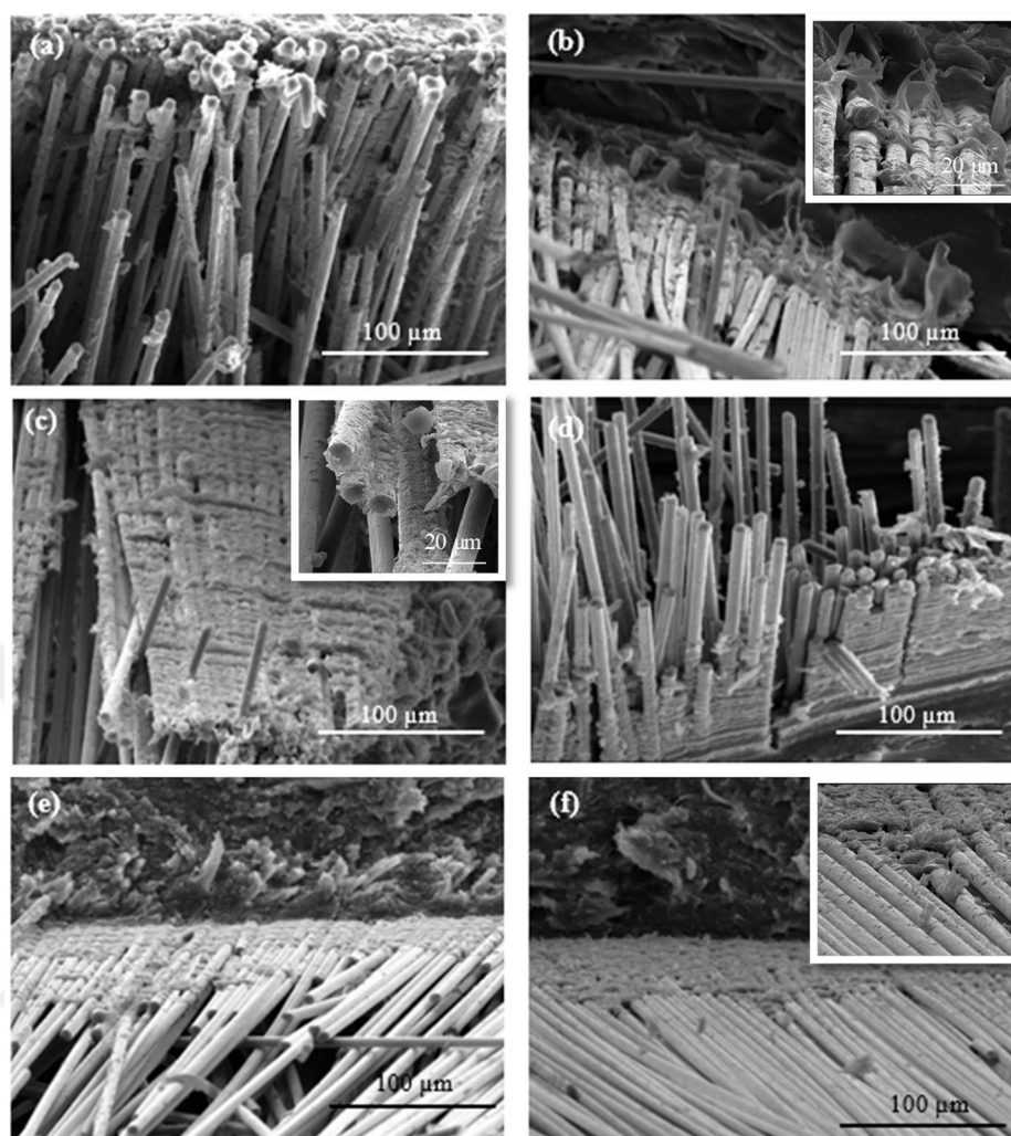
Figure 4.25. SEM images of the fractured surfaces of (a) PS-E-CF, (b) PS-E-CNT-CF and (c) PS-E-MSPM-A-CNT-CF multilayer composites prepared with method 1 and (d) PS-E-CF, (e) PS-E-CNT-CF, and (f) PS-E-MSPM-A-CNT-CF multilayer composites prepared with method 2 at 1000x.
