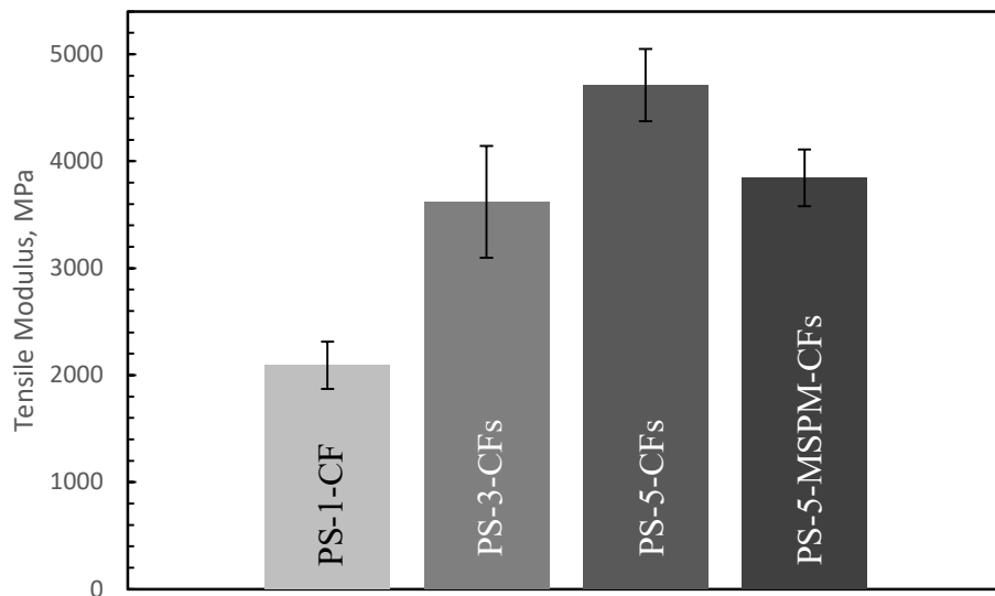
Figure 4.45. Tensile moduli of the multilayer composites.
