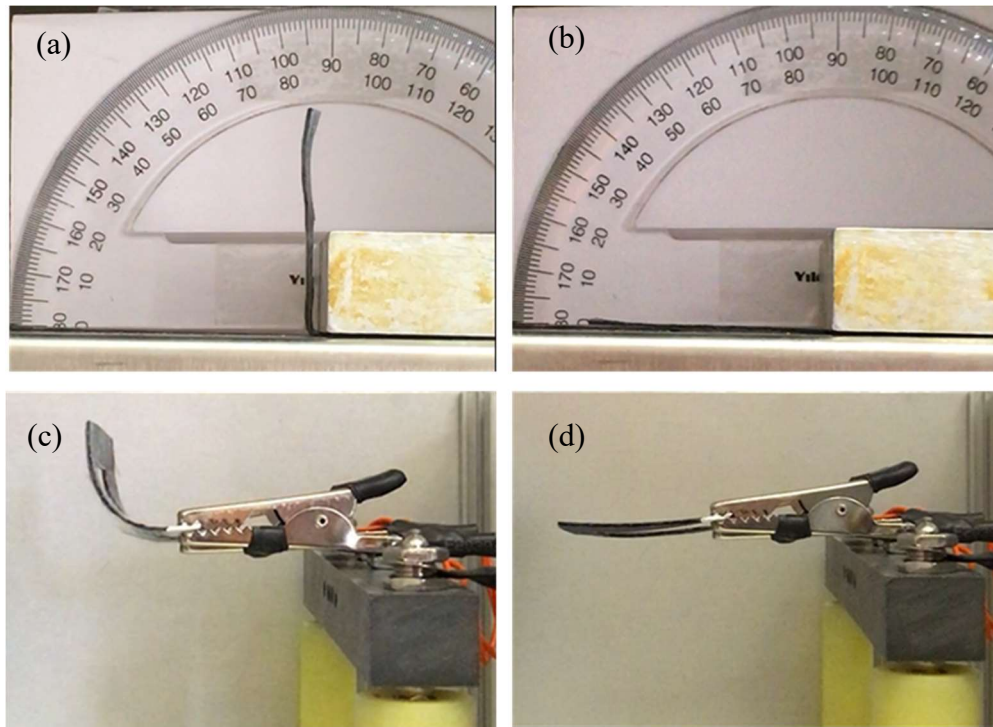
Figure 4.30. Thermally bending test images for masterbatch diluted PS-E-MSPM-A-CNT-CF samples (a) t=0 , (b) t=25 s, electrically bending test images for masterbatch diluted PS-E-MSPM-A-CNT-CF samples (c) t=0 , (d) t=20 s.
