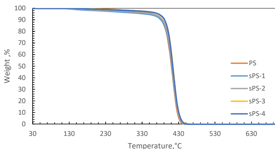
Figure 4.22. TGA plots of commercial PS and sPS samples prepared with different initiator concentrations.
