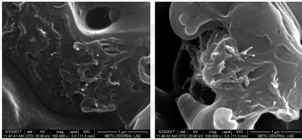
Figure 4.13. PS-E-CNT sample from fracture surface at 100000x (un-etched).
