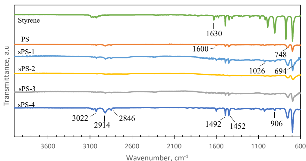
Figure 4.21. FTIR spectra of commercial PS and synthesized PS with different initiator concentrations.
