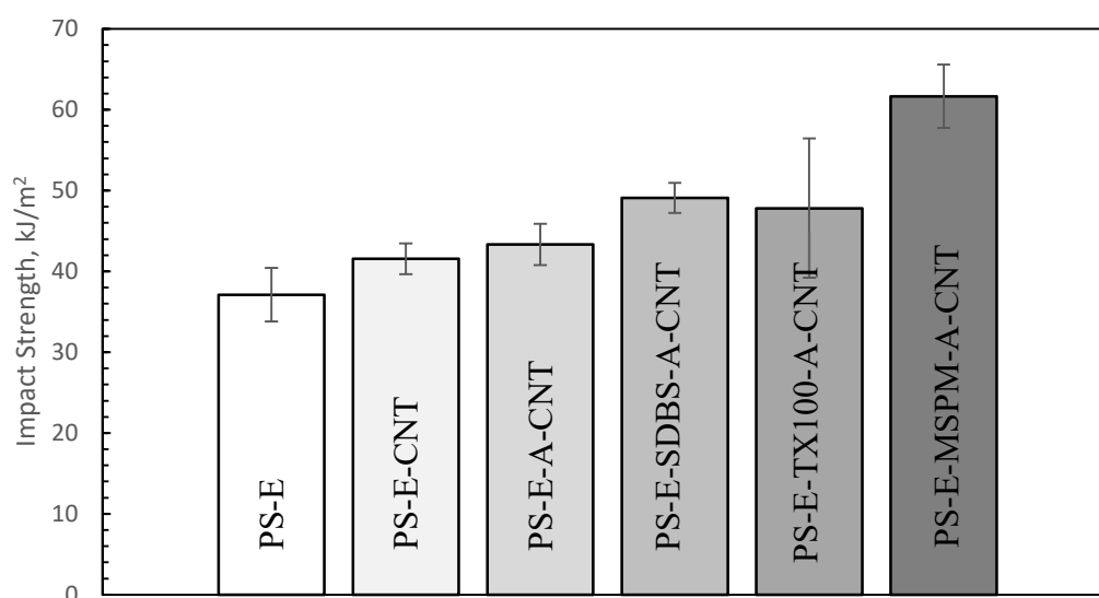
Figure 4.19. Impact strengths of the ternary composites.
