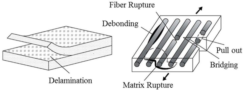
Figure 2.4. Failure mechanisms of laminated composites (Noels, 2018).
