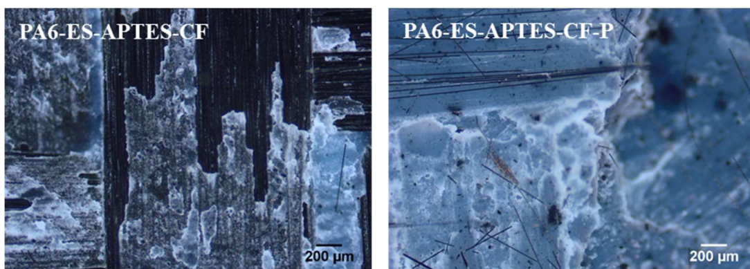
Figure 4.34 (cont'd). Micrographs of peeled surfaces of T-peel test specimens.
