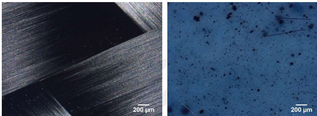
Figure 4.32. Micrographs of CF and PS-E-MSPM-A-CNT surfaces before multilayer composite preparation.
