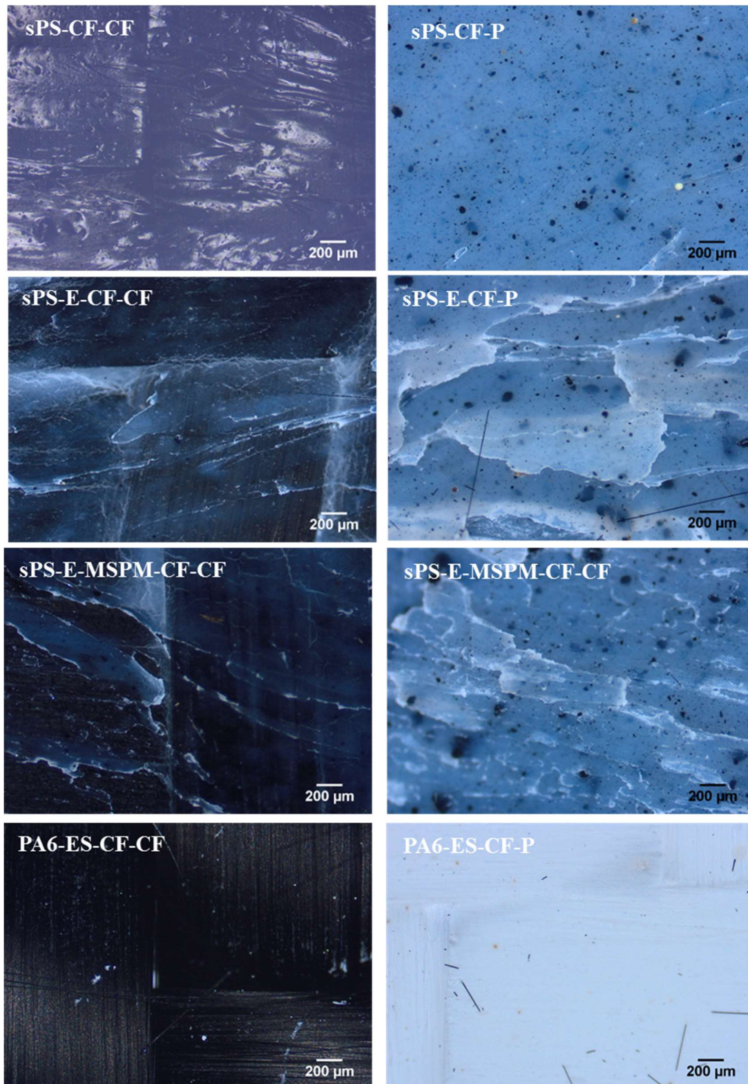
Figure 4.34 (cont'd). Micrographs of peeled surfaces of T-peel test specimens.
