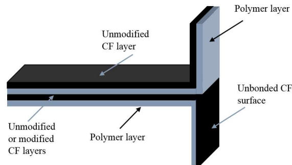
Figure 3.12. T-peel test specimen.
