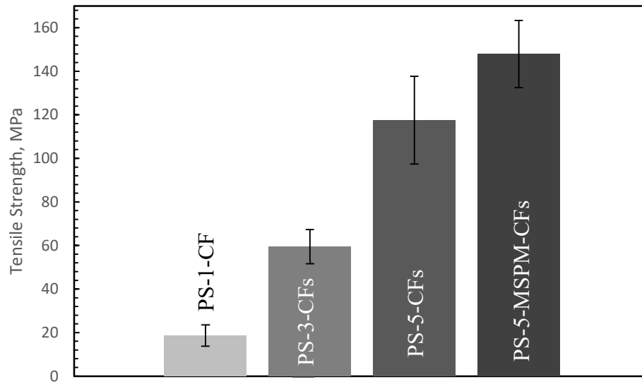
Figure 4.44. Tensile strengths of the multilayer composites.
