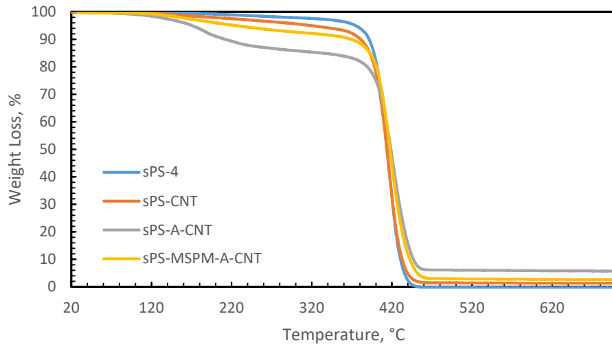
Figure 4.24. TGA plots of PS-CNT masterbatches.
