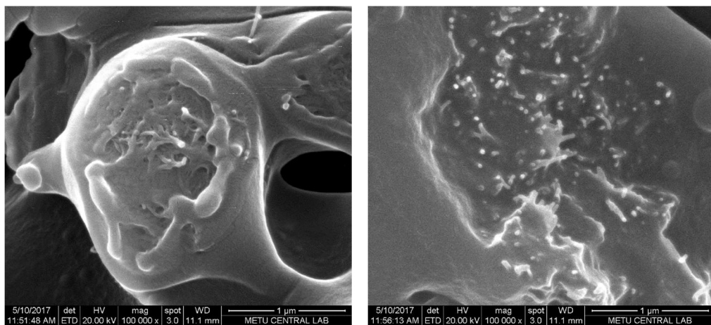
Figure 4.14. PS-E-MSPM-A-CNT sample from fracture surface at 100000x (un-etched).
