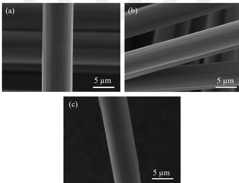
Figure 4.39. SEM images of (a) CF, (b) Desized-CF and (c) Desized-MSPM-CF samples.
