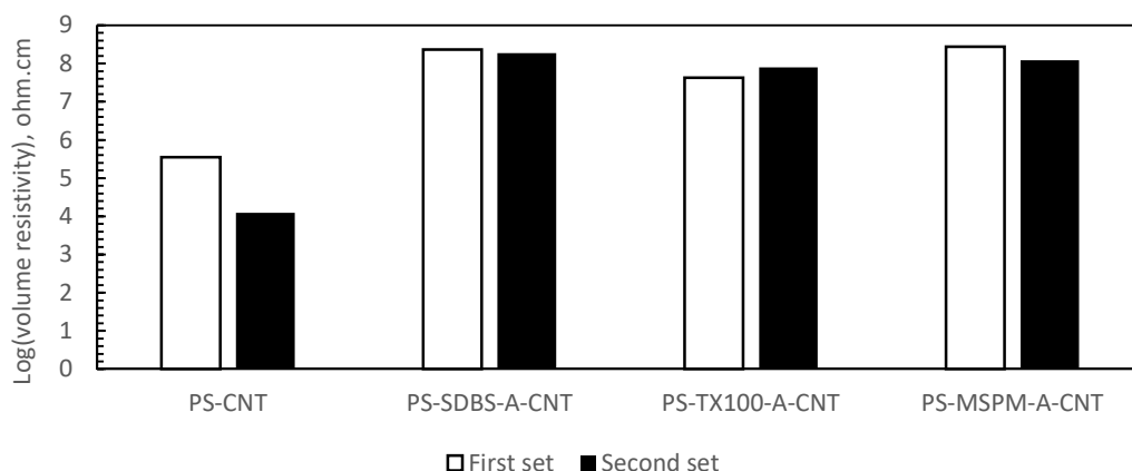
Figure 4.4. Electrical resistivity values of the binary composites.
