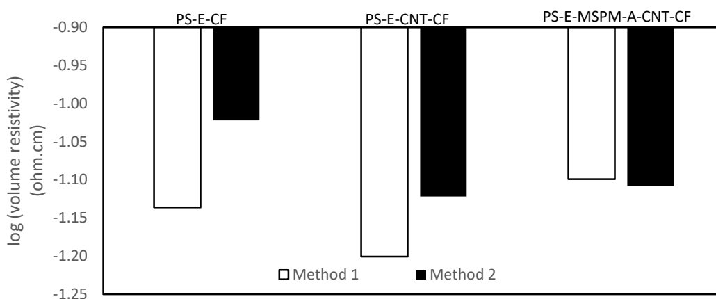
Figure 4.26. Electrical resistivities of the multilayer composites.
