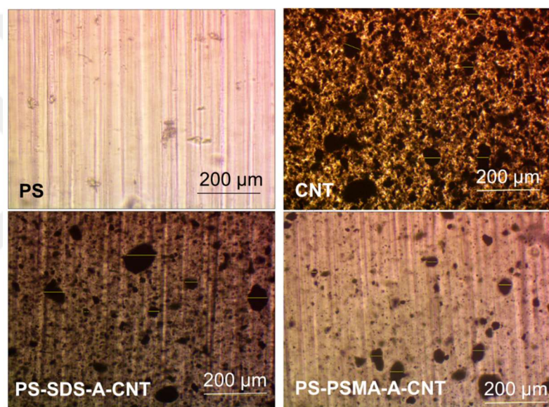
Figure 4.3. Optical Microscope images of PS-CNT binary composites prepared with different surface modifiers.
