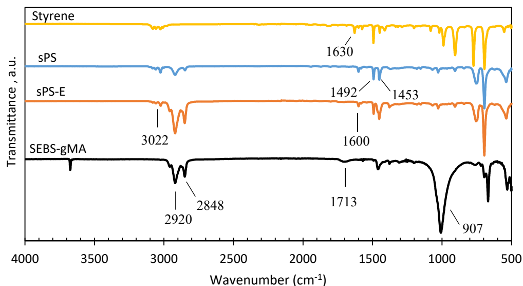
Figure 4.35. FTIR spectra of in-situ polymerized PS (sPS), in-situ polymerized PS-E (sPS-E) and SEBS-gMA.
