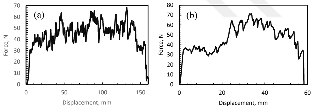
Figure 4.40. Force vs. displacement plot of the multilayer composite with (a) CF and (b) MSPM-CF.
