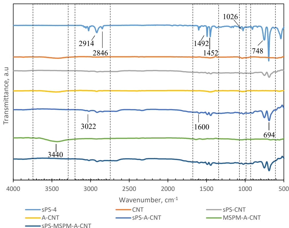
Figure 4.23. FTIR spectra of in-situ polymerized PS-CNT masterbatches and CNT samples.
