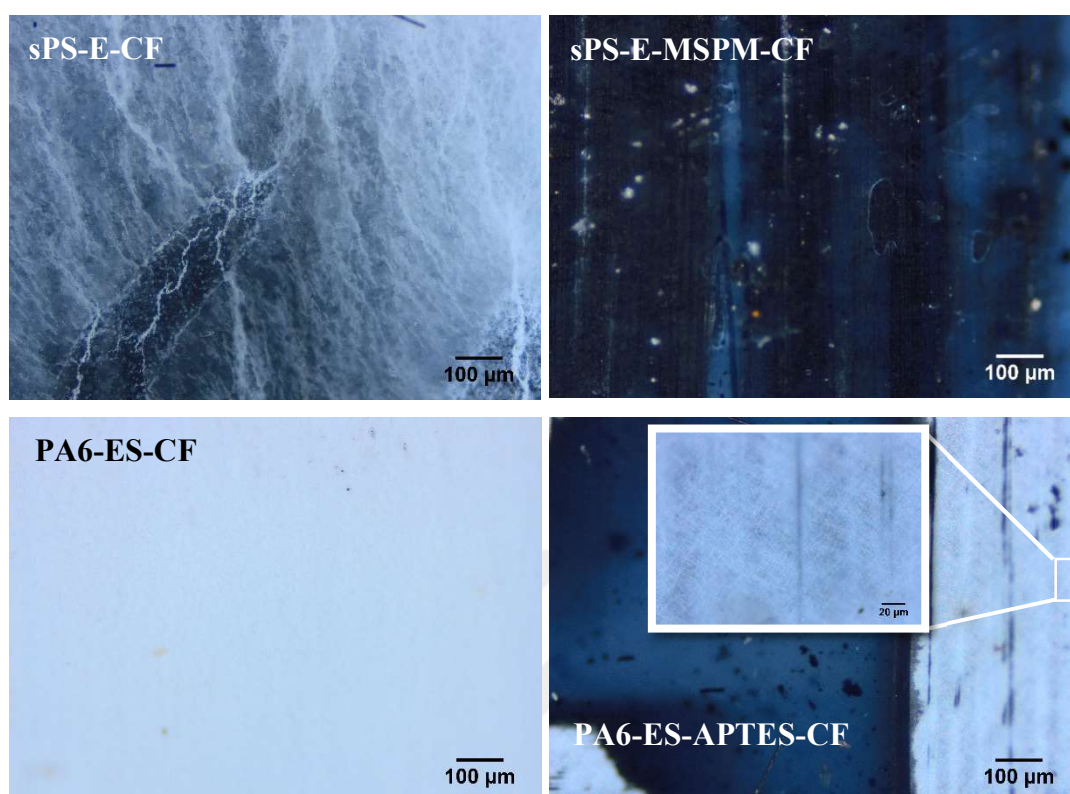
Figure 4.33. (cont'd) Micrographs of unbonded surfaces of T-peel test specimens.
