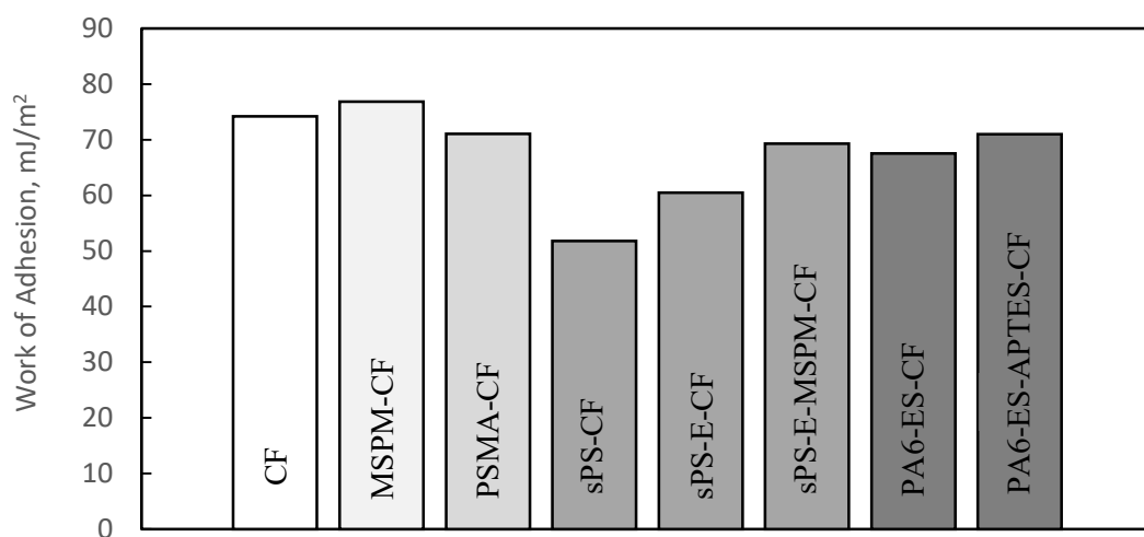
Figure 4.31. Work of adhesion between polymer layer and CF surfaces.
