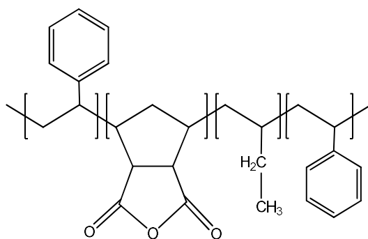
Figure 3.1. Chemical structure of SEBS-gMA (“Technical Data Sheet of Kraton FG 1924 G,” 2017; Yeniova et al., 2010).
