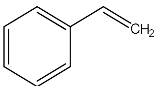
Figure 3.2. Chemical structure of styrene.
