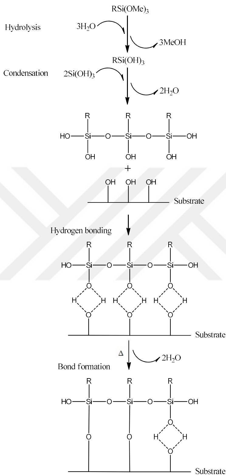
Figure 2.5. Reaction steps of hydrolytic deposition of silanes (Arkles, 2014).
