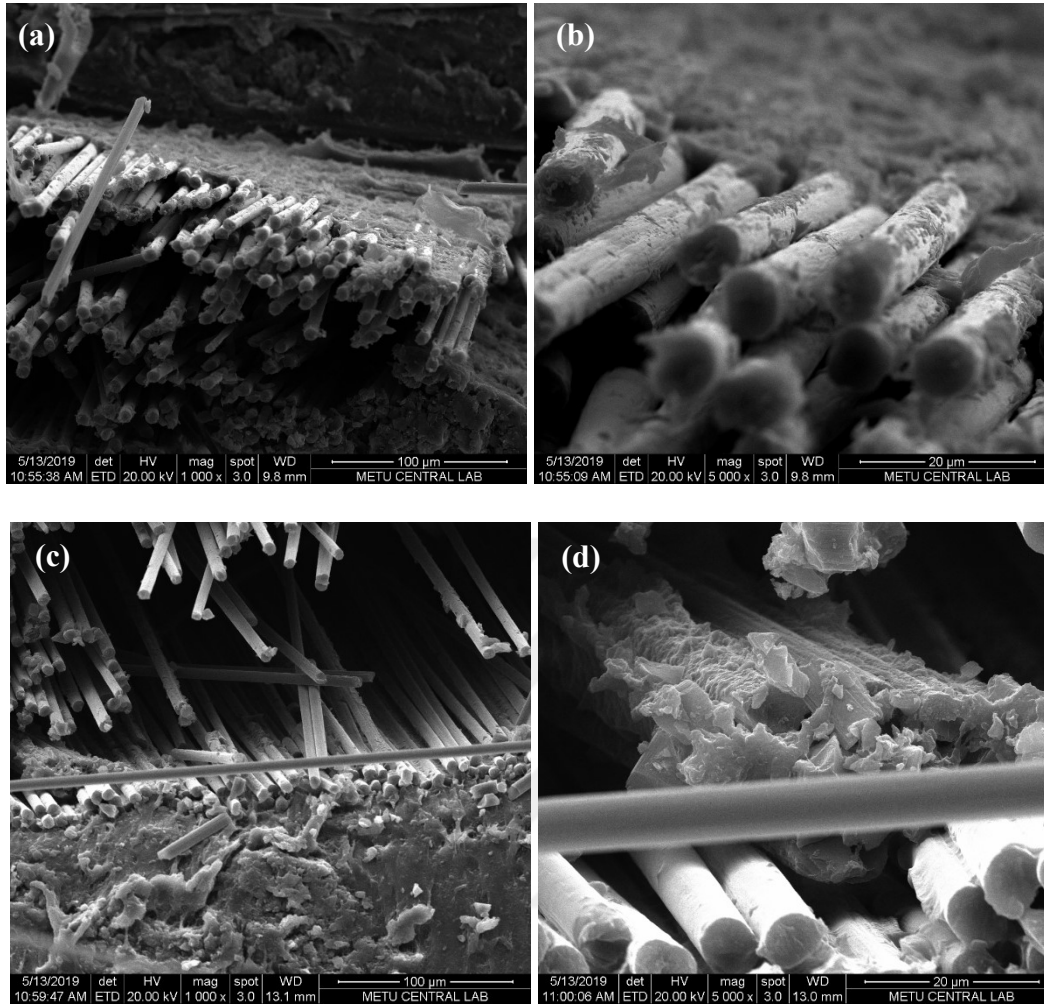
Figure 4.42. SEM images of the fracture surfaces of the multilayer composites; (a), (b) PS-1-CF, (c), (d) PS-3-CFs, (e), (f) PS-5-CFs and (g), (h) PS-5-MSPM-CFs at 1000x and at 5000x magnification, respectively.
