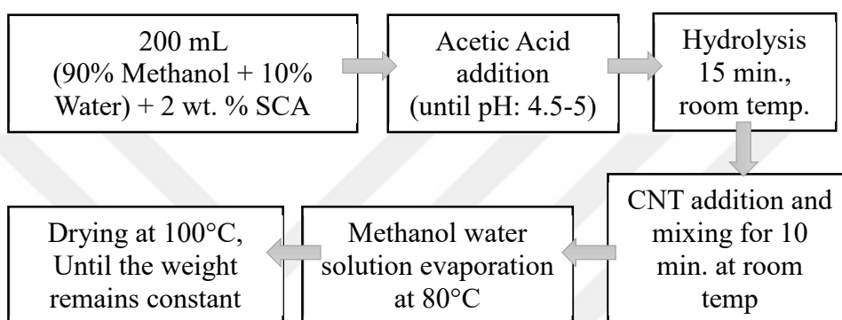
Figure 3.7. Flow chart of preparation steps of MSPM-A-CNT and GLYMO-A-CNT samples.
