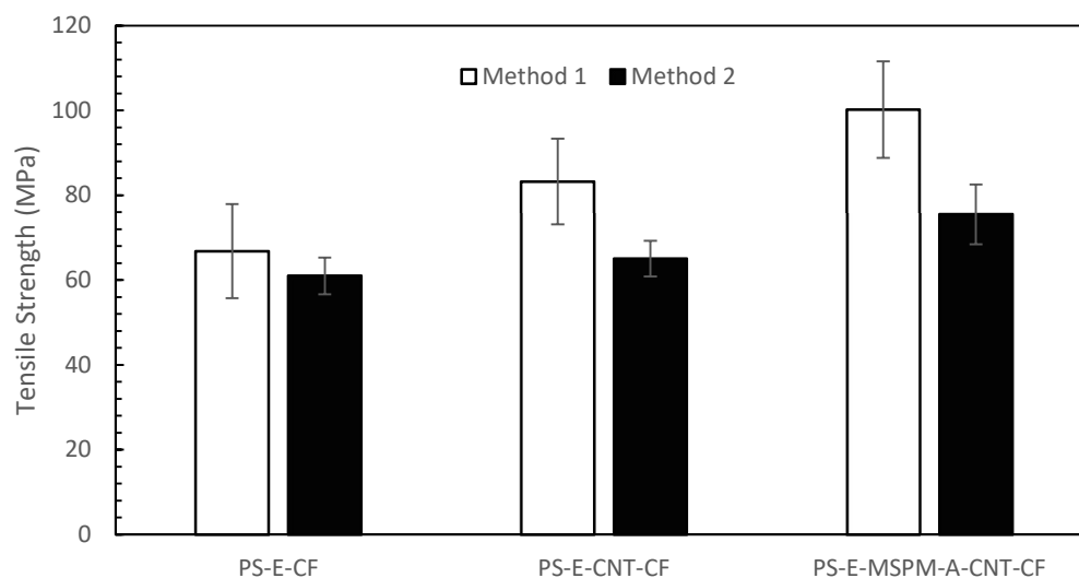
Figure 4.27. Tensile strengths of the multilayer composites.
