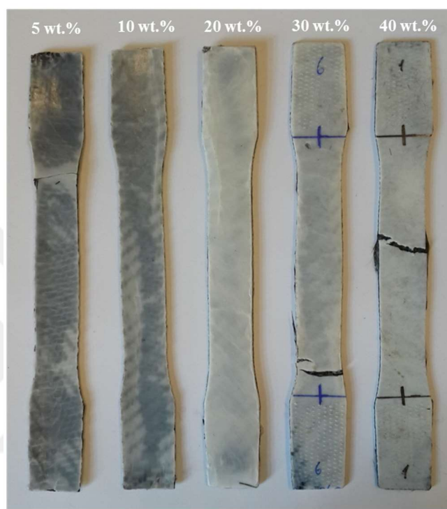
Figure 4.9. PS-E-CF samples prepared with different amount of elastomer (SEBS gMA) addition.
