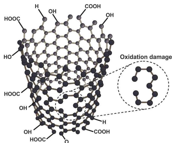
Figure 2.2. Schematic representation of oxidative functional groups and structural damages formed after oxidation treatment (adopted from Avilés et al., 2018 with permission).
