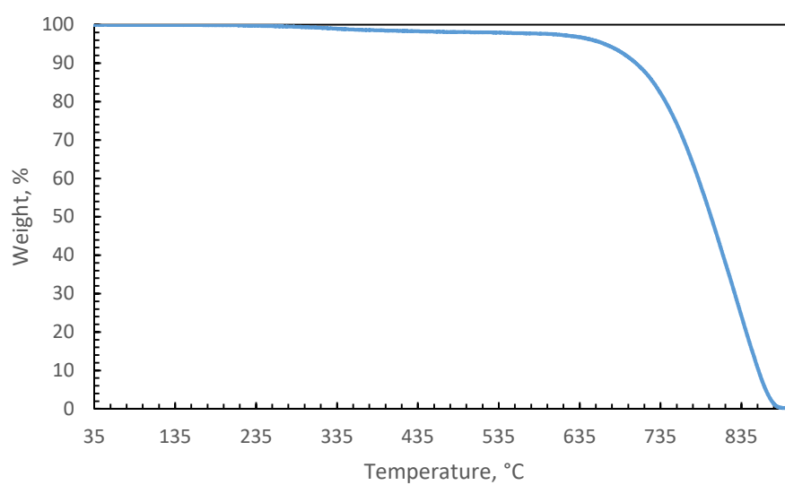
Figure A.1. TGA curve of as-received CF sample in air atmosphere.
