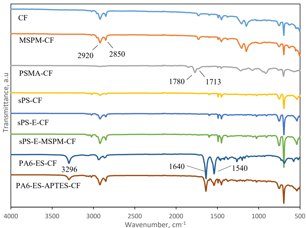
Figure 4.36. FTIR spectra of un-bonded surfaces of T-peel test specimens.
