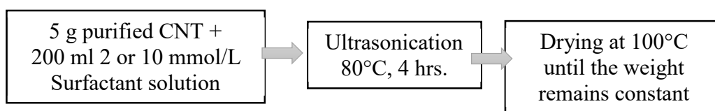
Figure 3.6. Flow chart of preparation steps of SDBS-A-CNT and TX100-A-CNT samples.
