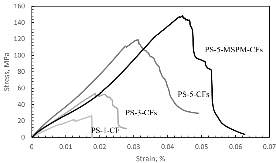
Figure 4.43. Stress-strain plots of the multilayer composites.
