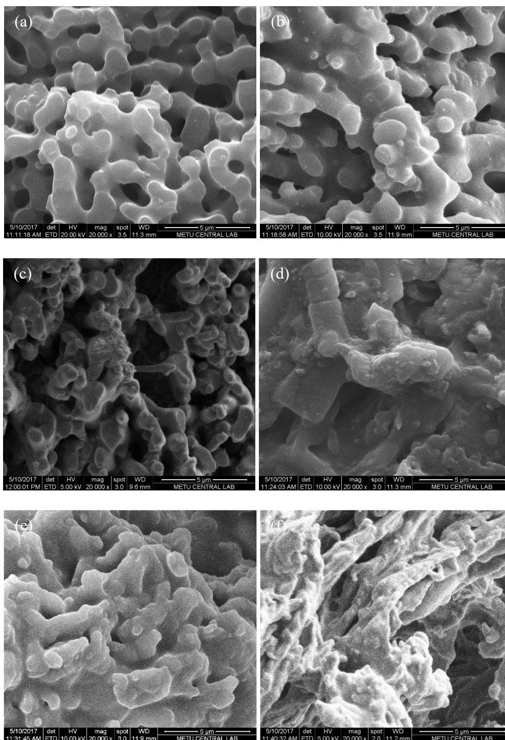
Figure 4.12. SEM images of (a) PS-E, (b) PS-E-CNT, (c) PS-E-A-CNT, (d) PS-E-SDBS-A-CNT, (e) PS-E-TX100-A-CNT, (f) PS-E-MSPM-A-CNT at 20000x magnification (etched with n-heptane).
