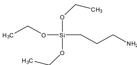
Figure 3.4. Chemical structure of APTES (“Properties of (3-Aminopropyl)triethoxysilane.” 2017).
