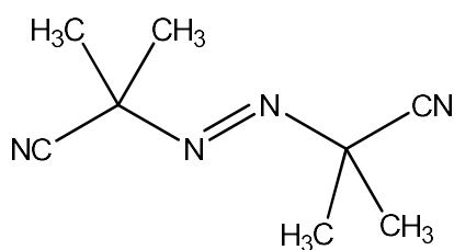
Figure 3.3. Chemical structure of AIBN (“Properties of AIBN,” 2017).
