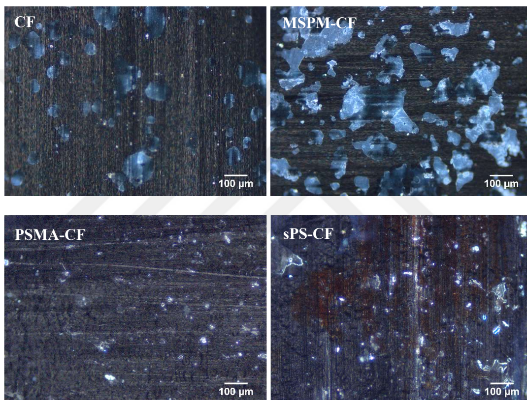
Figure 4.33. Micrographs of unbonded surfaces of T-peel test specimens.
