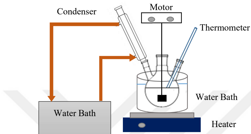
Figure 3.9. Schematic representation of bulk polymerization experimental set-up.
