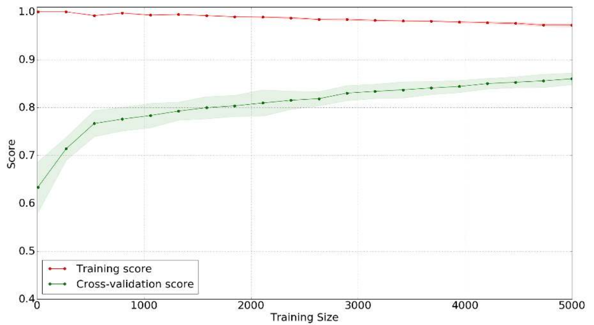
Figure 4. LinearSVC Learning Curve with Best Unigram Features
