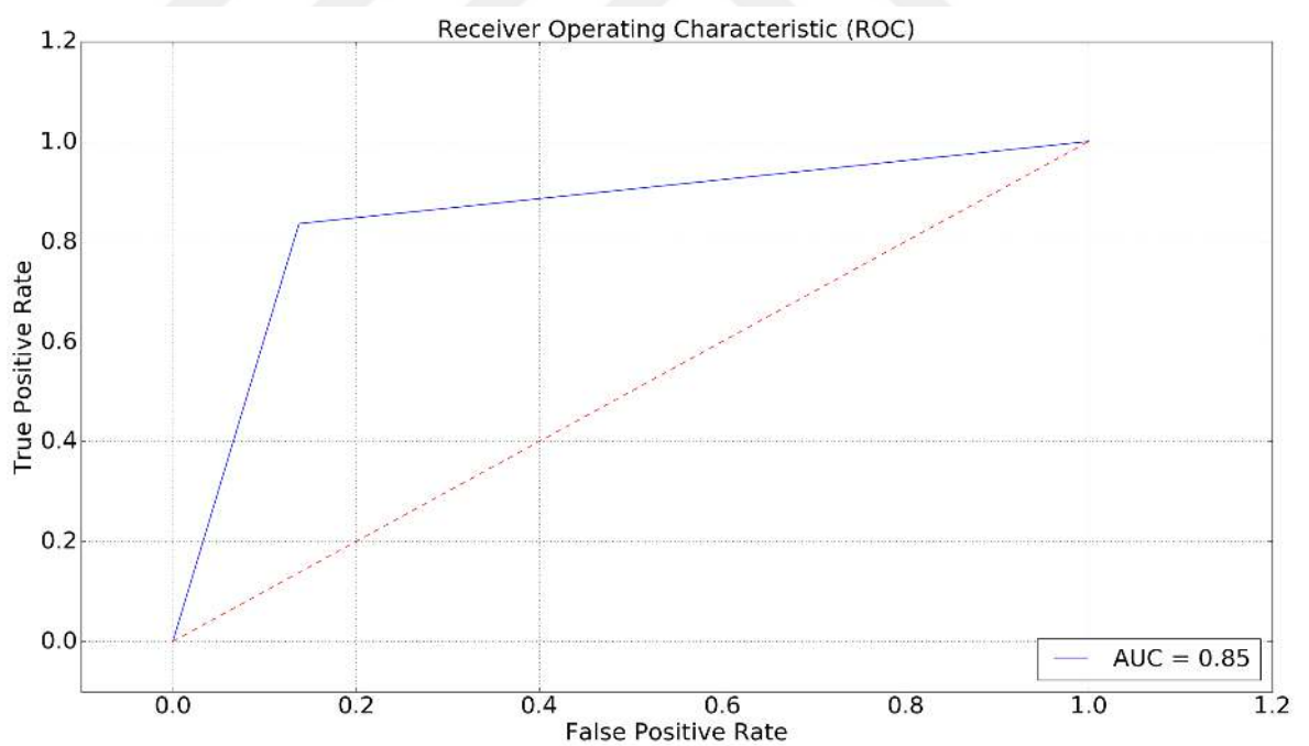
Figure 5. LinearSVC ROC Curve with Best Unigram Features
