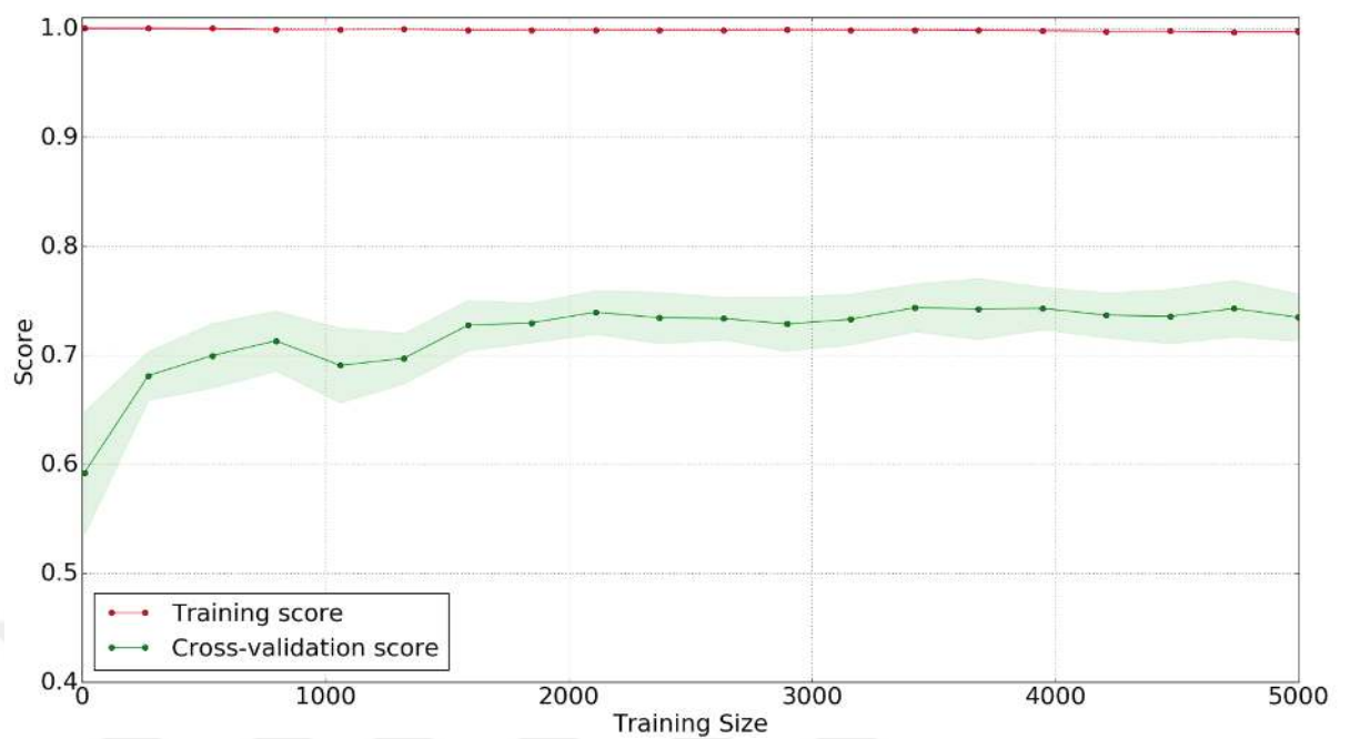
Figure 8. Decision Trees Learning Curve with Best Unigram Features
