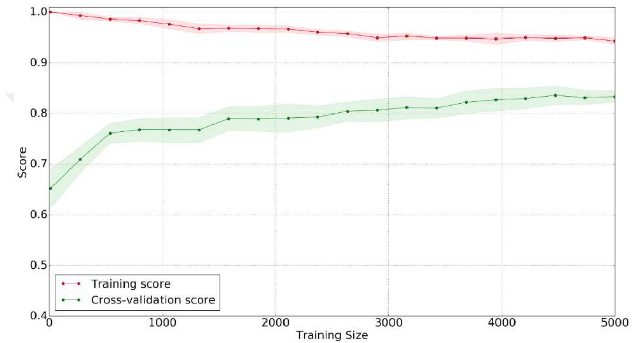
Figure 10. SGD Learning Curve with Best Unigram Features
