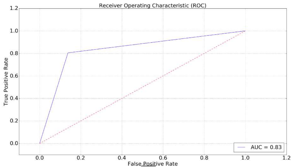
Figure 11. SGD ROC Curve with Best Unigram Features
