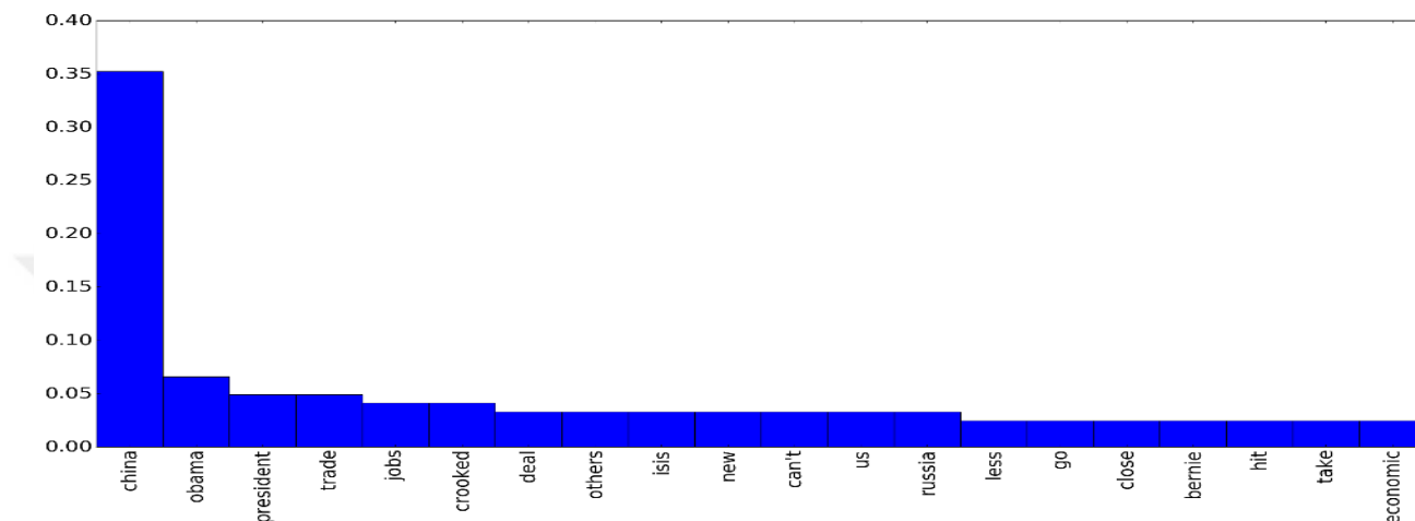
Figure 26. China Tweets Token Distribution
