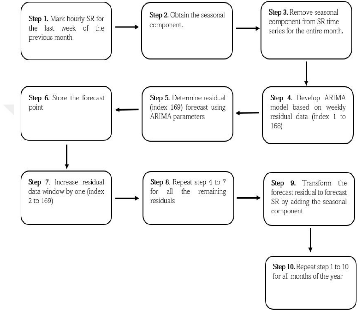
Figure 5.2: Scenario generation flow diagram.
