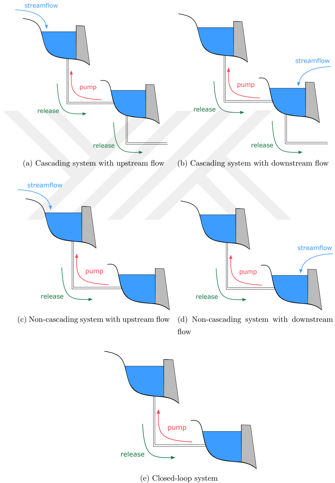
Figure 4.1: Illustration of various PHES configurations.
