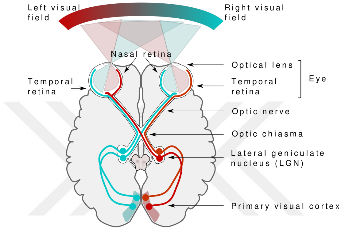
Figure 1.1: Contralateral processing in visual system. Drawn by Miquel Perello Nieto, under shareable license [CC BY-SA 4.0 ( https://creativecommons.org/licenses/by-sa/4.0 )]
