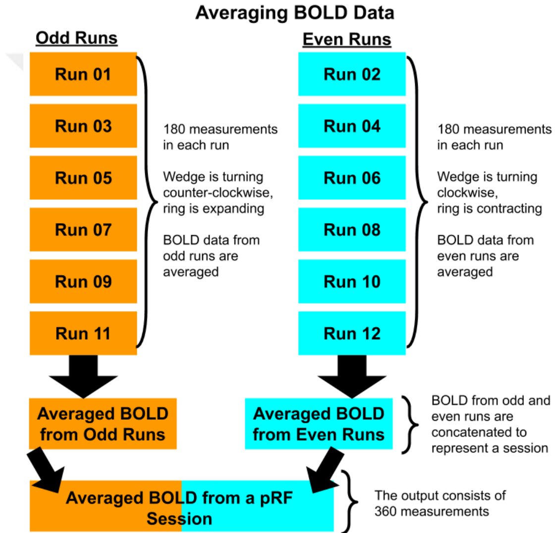
Figure 2.2: BOLD Averaging
