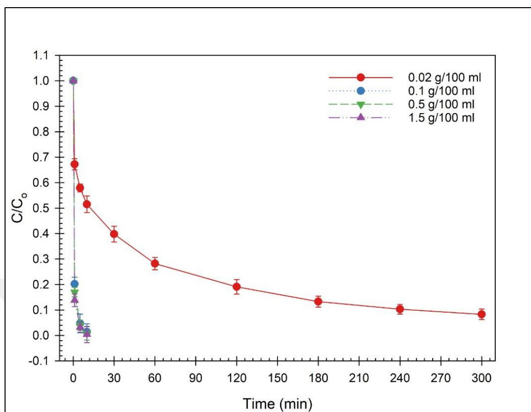
Figure 4.43. Effect of various U10HC210BC700KOH1 biochar dose on the phorate removal at 25 °C
