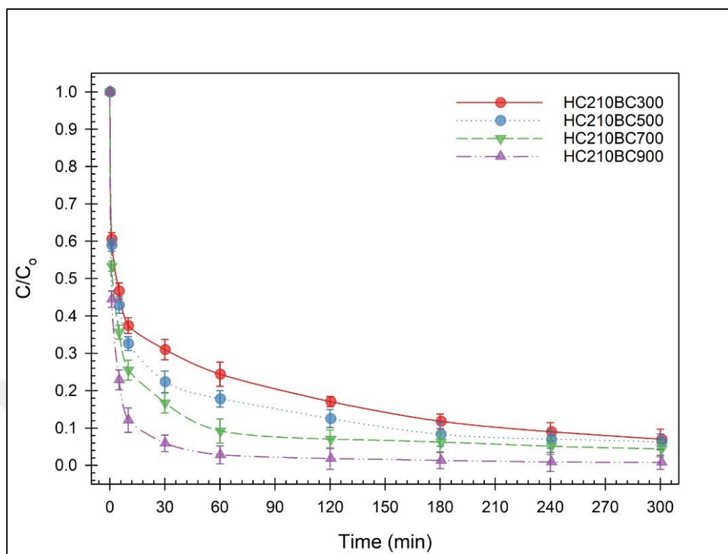
Figure 4.33. Phorate removal ratios of 1 g/L hydrothermally treated biochars at 25 °C
