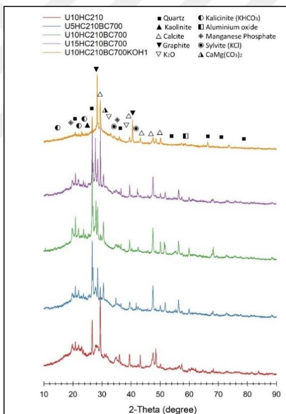
Figure 4.12. XRD diffraction pattern of urea pre-modified hydrothermally treated biochars
