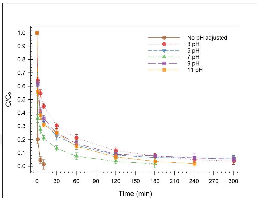
Figure 4.46. Effect of 1 g/L U10HC210BC700KOH1 on the phorate removal in pH varied solutions at 25 °C
