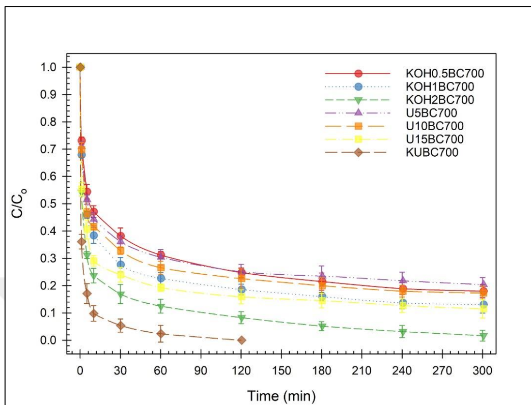
Figure 4.32. Phorate removal ratios of 1 g/L KOH and urea modified biochars at 25 °C
