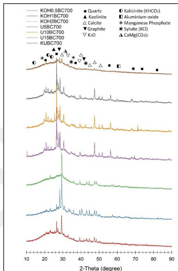
Figure 4.9. XRD diffraction pattern of pre-modified biochars
