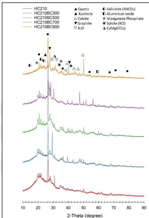
Figure 4.10. XRD diffraction pattern of hydrothermally treated biochars
