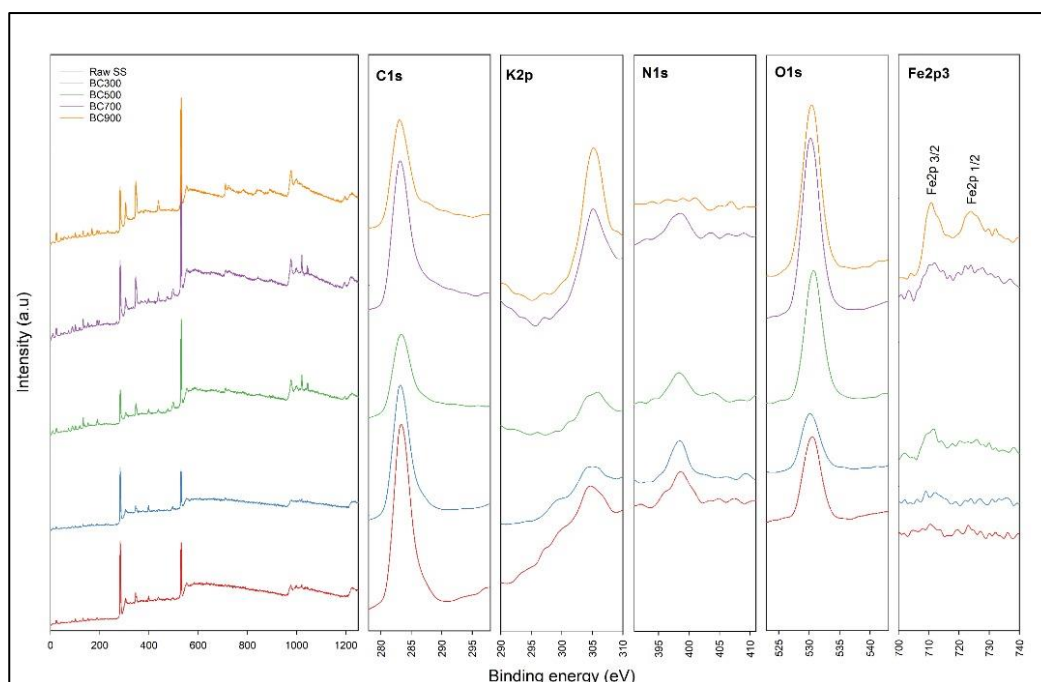
Figure 4.25. XPS spectra of Raw SS and pristine biochars
