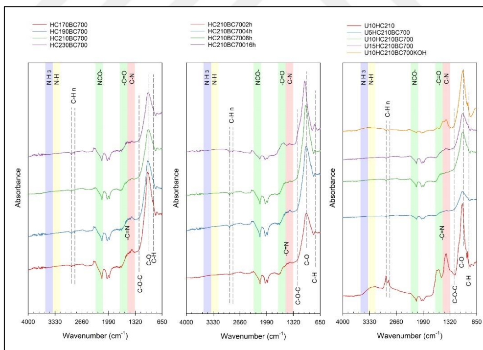
Figure 4.17. FTIR spectra of time- and temperature-varied hydrothermal biochars and urea pre-modified hydrothermal biochars
