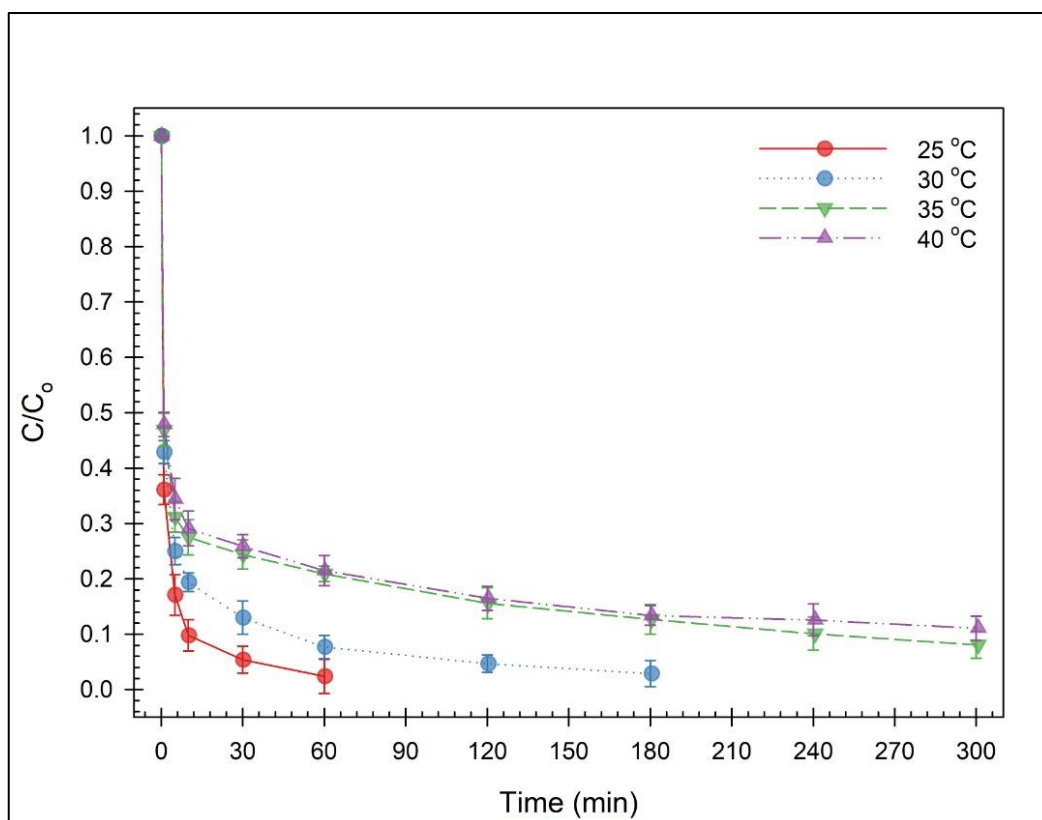
Figure 4.38. Effect of 1 g/L KUBC700 on the phorate removal under varied temperatures
