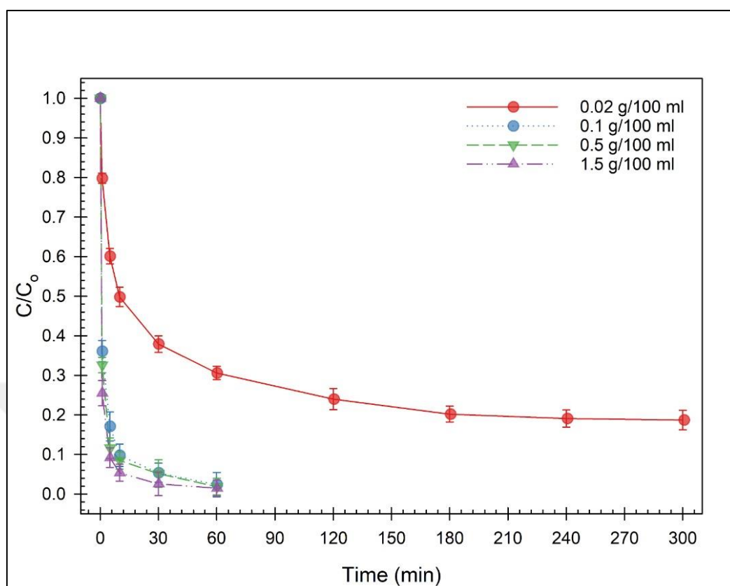
Figure 4.41. Effect of various KUBC700 biochar dose on the phorate removal at 25 °C
