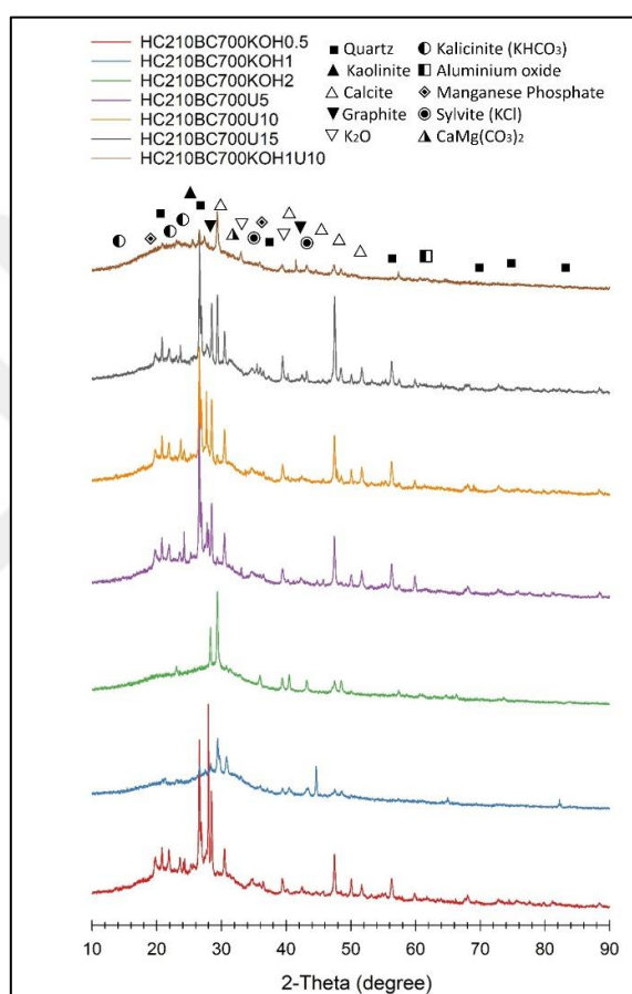
Figure 4.11. XRD diffraction pattern of post-modified hydrothermally treated biochars
