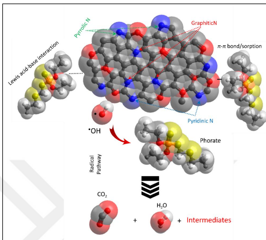
Figure 4.51. Biochar based free-radical-assisted degradation mechanism of phorate into intermediate degradation products
