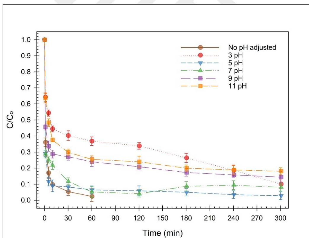
Figure 4.44. Effect of 1 g/L KUBC700 on the phorate removal in pH varied solutions at 25 °C
