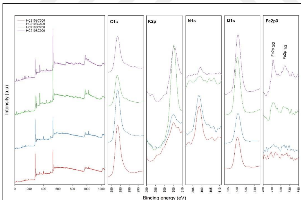
Figure 4.27. XPS spectra of hydrothermally produced biochars
