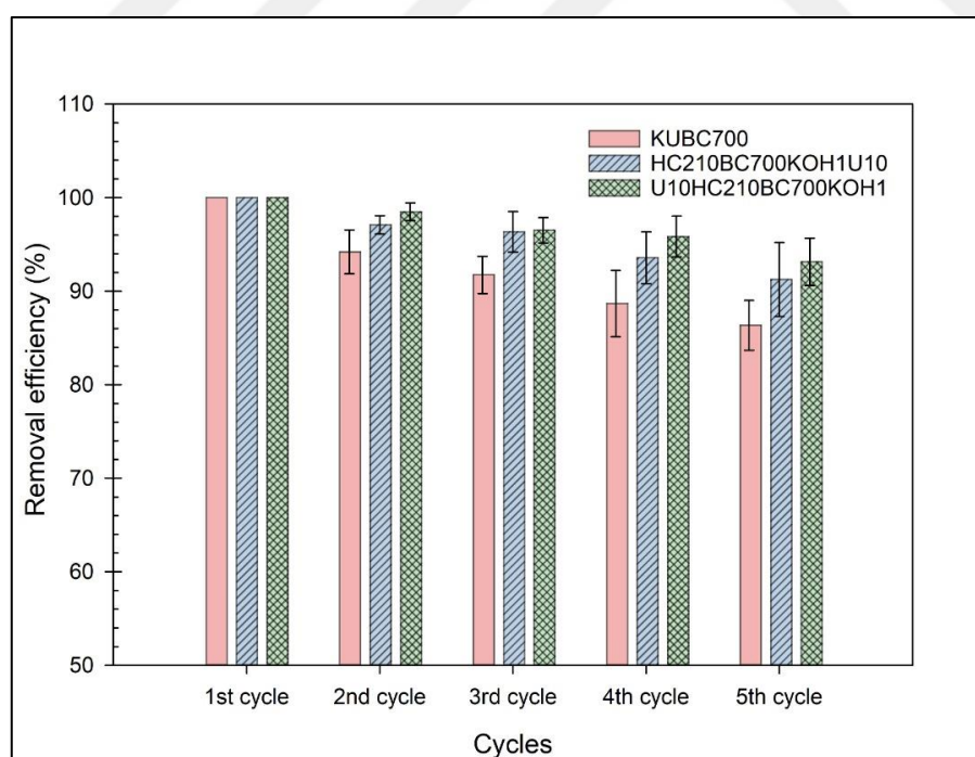
Figure 4.47. Phorate removal efficiencies of 1 g/L biochars for each reusability experiment at 25 °C
