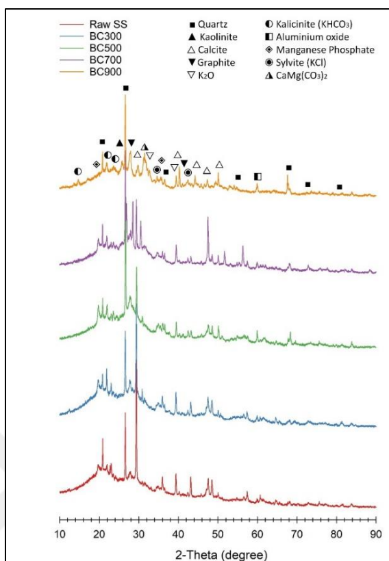
Figure 4.8. XRD diffraction pattern of the Raw SS and pristine biochars
