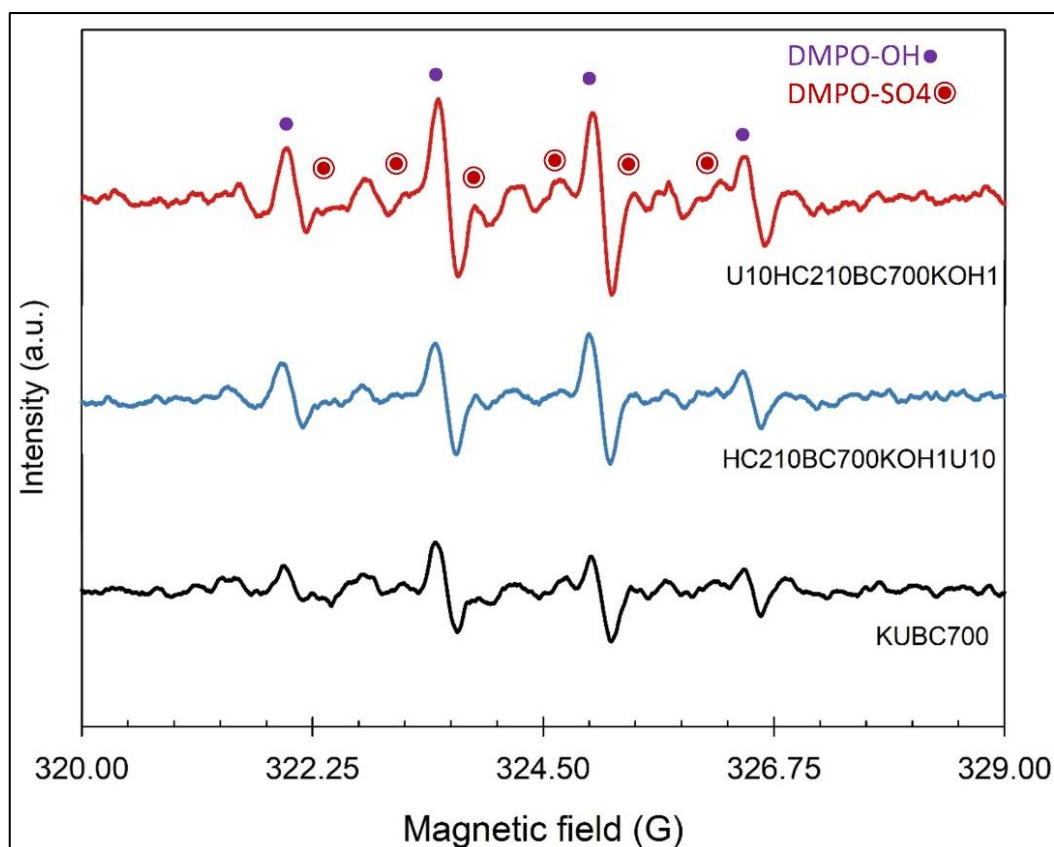
Figure 4.30. EPR spectra of generated oxygen focused free-radicals for three selected biochar samples
