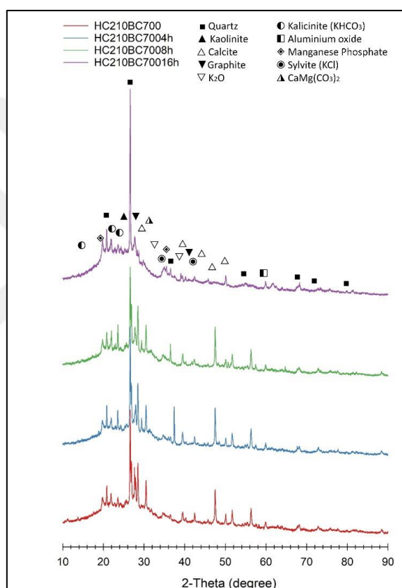
Figure 4.13. XRD diffraction pattern of hydrothermally treated biochars with various residence times
