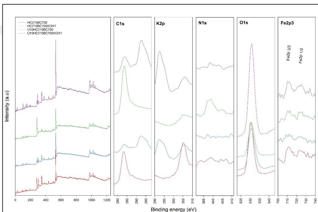
Figure 4.29. XPS spectra of pre- and post-modified hydrothermally produced biochars
