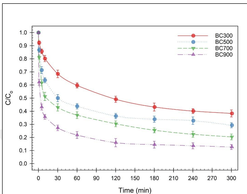
Figure 4.31. Phorate removal ratios of 1 g/L pristine biochars at 25 °C
