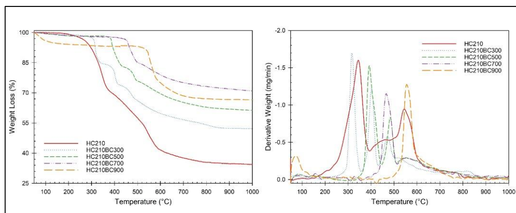
Figure 4.20. Thermochemical properties of hydrothermally treated biochars
