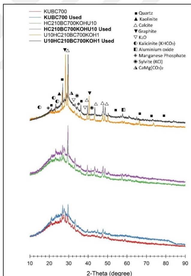
Figure 4.48. XRD diffraction pattern of used and unused modified biochars
