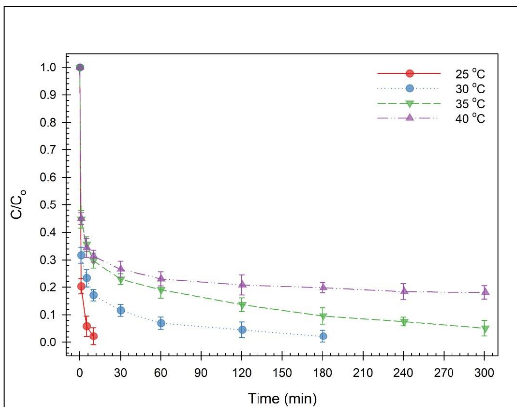
Figure 4.39. Effect of 1 g/L HC210BC700KOH1U10 on the phorate removal under varied temperatures
