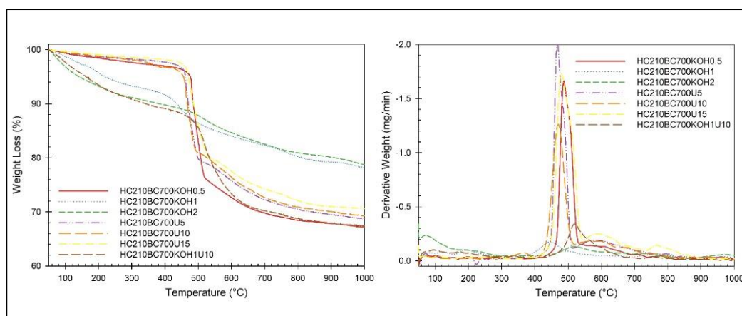
Figure 4.21. Thermochemical properties of post-modified hydrothermally treated biochars
