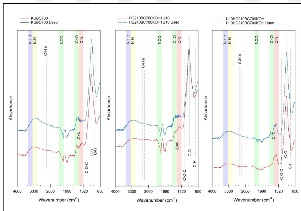
Figure 4.49. FTIR spectra of used and unused modified biochars
