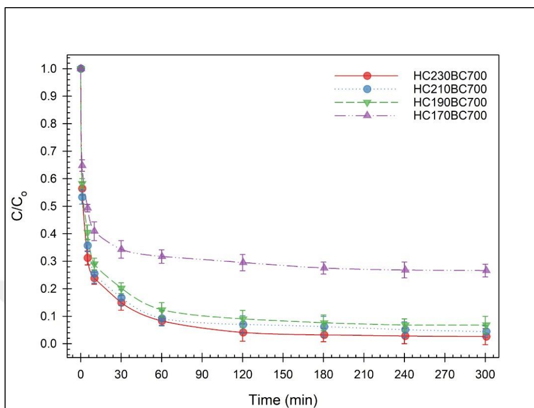
Figure 4.37. Phorate removal ratios of 1 g/L temperature varied hydrothermally treated biochars at 25 °C
