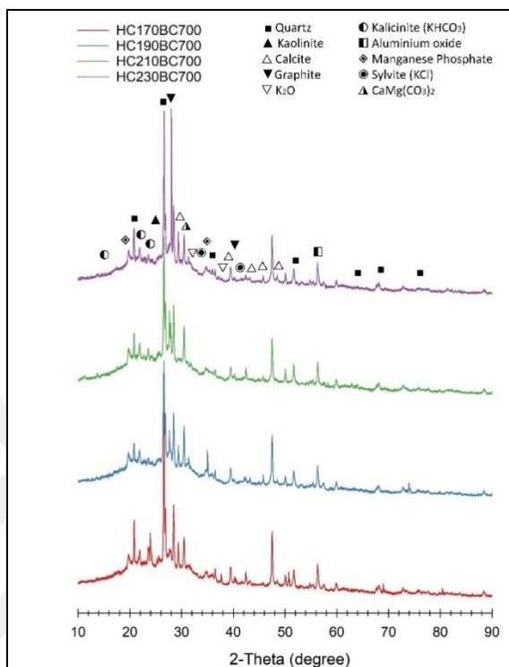
Figure 4.14. XRD diffraction pattern of hydrothermally treated biochars with various temperatures
