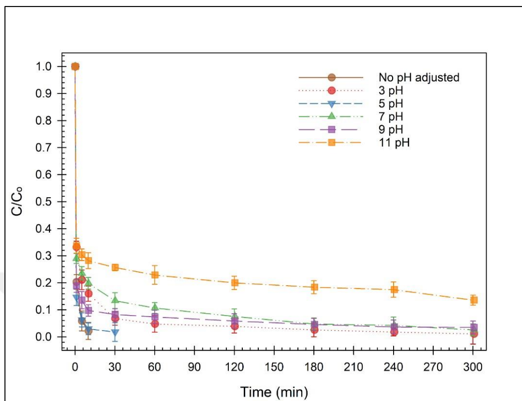
Figure 4.45. Effect of 1 g/L HC210BC700KOH1U10 on the phorate removal in pH varied solutions at 25 °C
