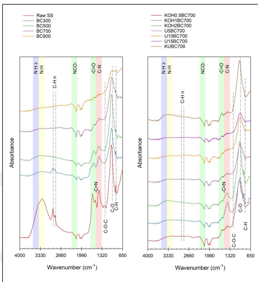
Figure 4.15. FTIR spectra of pristine and modified biochars
