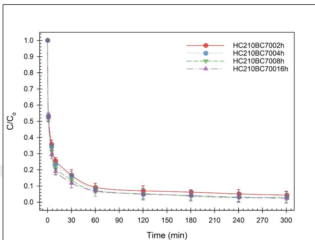
Figure 4.36. Phorate removal ratios of 1 g/L residence time varied hydrothermally treated biochars at 25 °C
