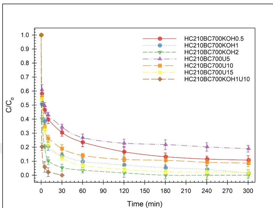
Figure 4.34. Phorate removal ratios of 1 g/L KOH and urea modified hydrothermally treated biochars at 25 °C
