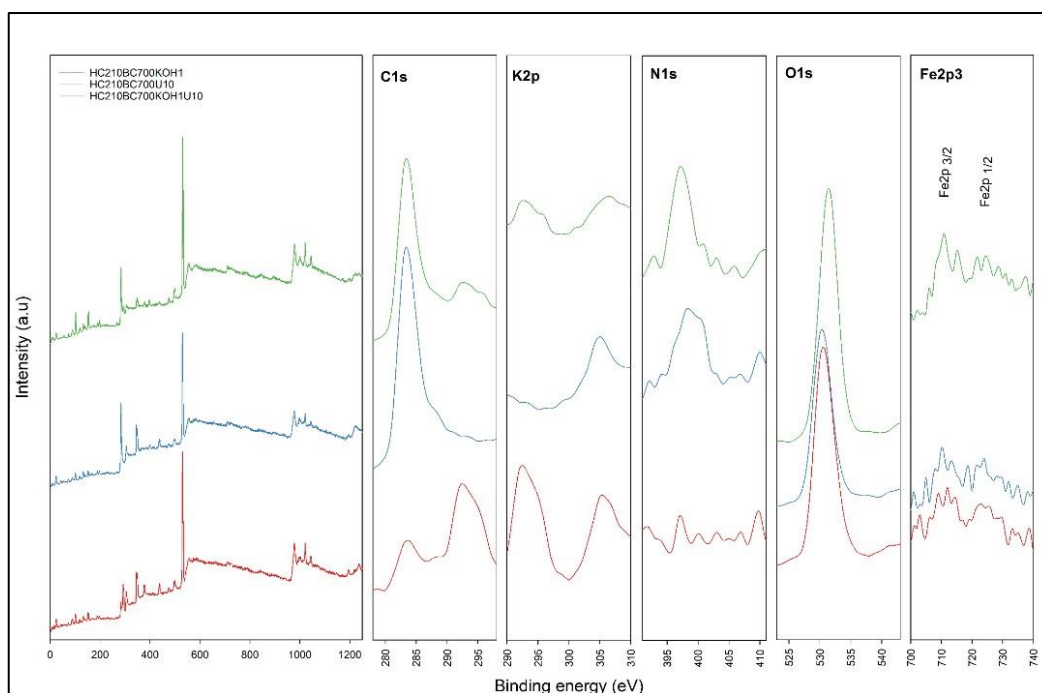
Figure 4.28. XPS spectra of post-modified hydrothermally treated biochars
