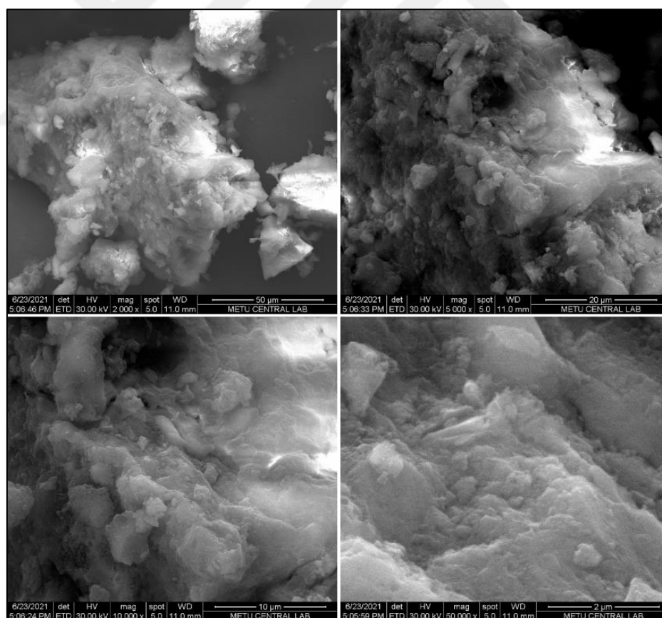
Figure 4.1. SEM image of raw sewage sludge (Raw SS)
