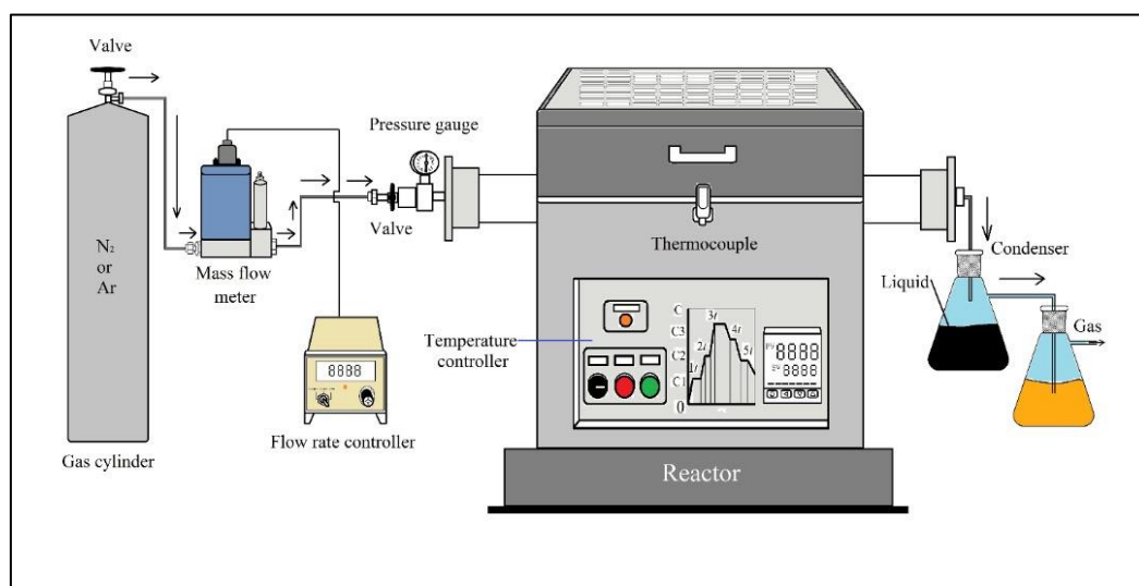
Figure 3.1. Split type tube furnace used in the pyrolysis experiments
