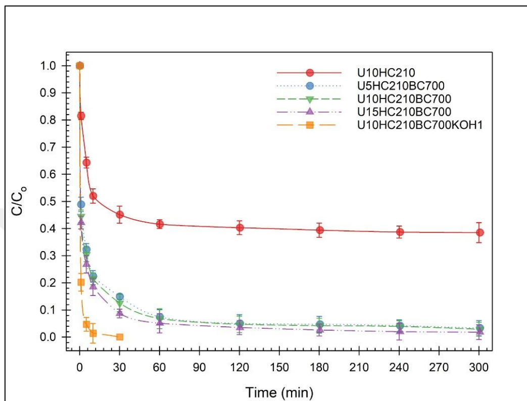
Figure 4.35. Phorate removal ratios of 1 g/L urea pre-modified hydrothermally treated biochars at 25 °C
