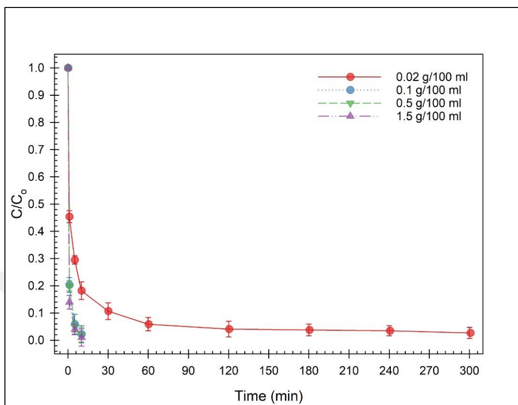
Figure 4.42. Effect of various HC210BC700KOH1U10 biochar dose on the phorate removal at 25 °C
