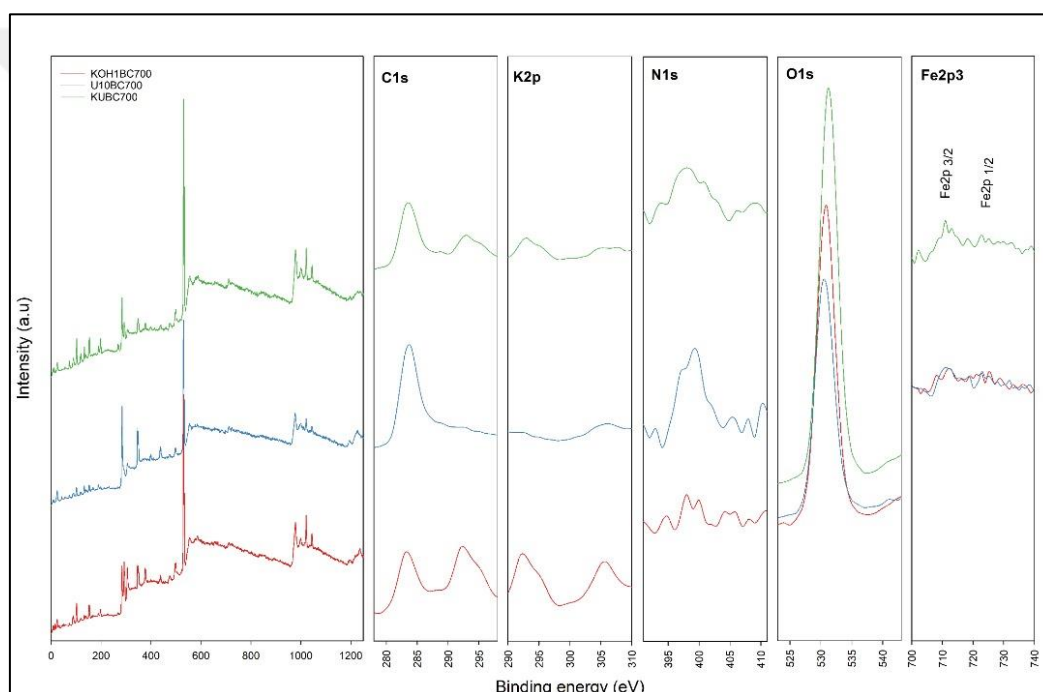
Figure 4.26. XPS spectra of modified biochars
