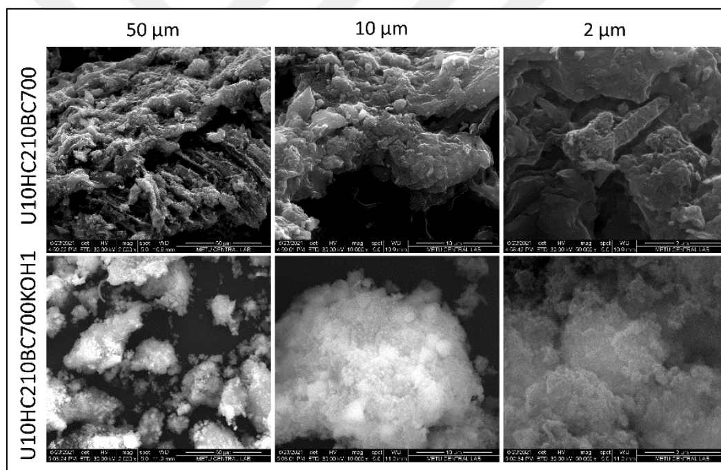
Figure 4.6. SEM images of pre- and post-modified hydrothermally treated biochar materials
