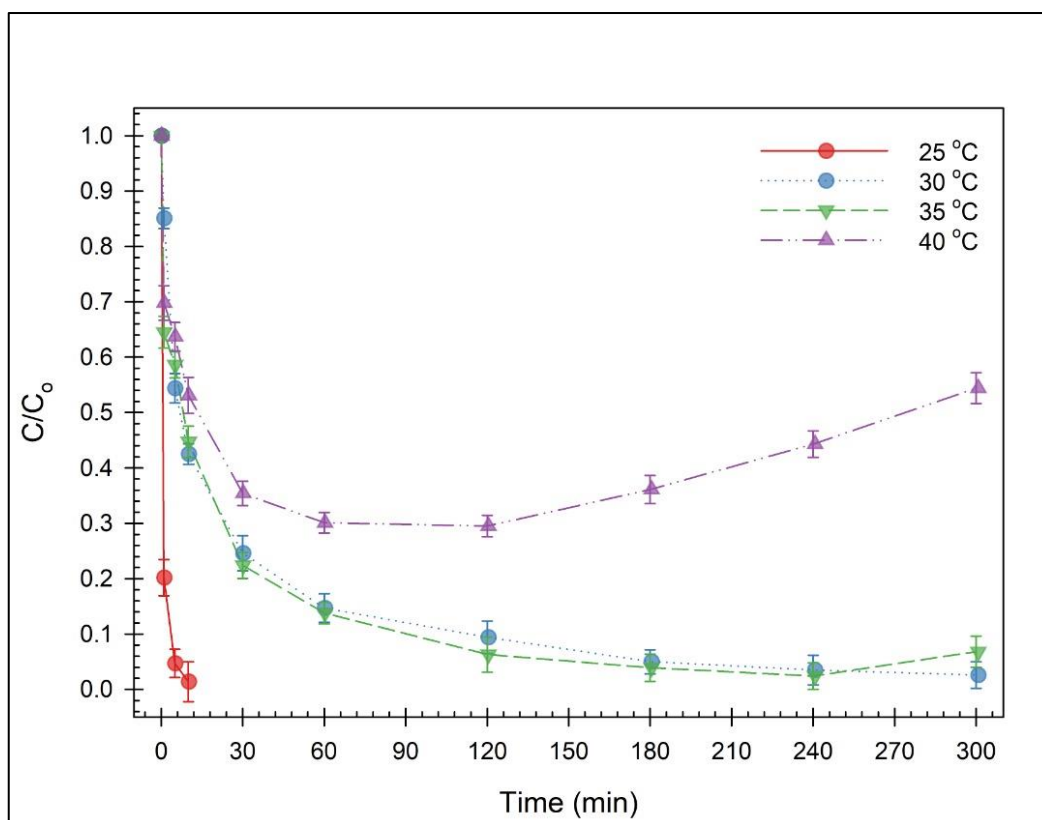
Figure 4.40. Effect of 1 g/L U10BC210BC700KOH1 on the phorate removal under varied temperatures
