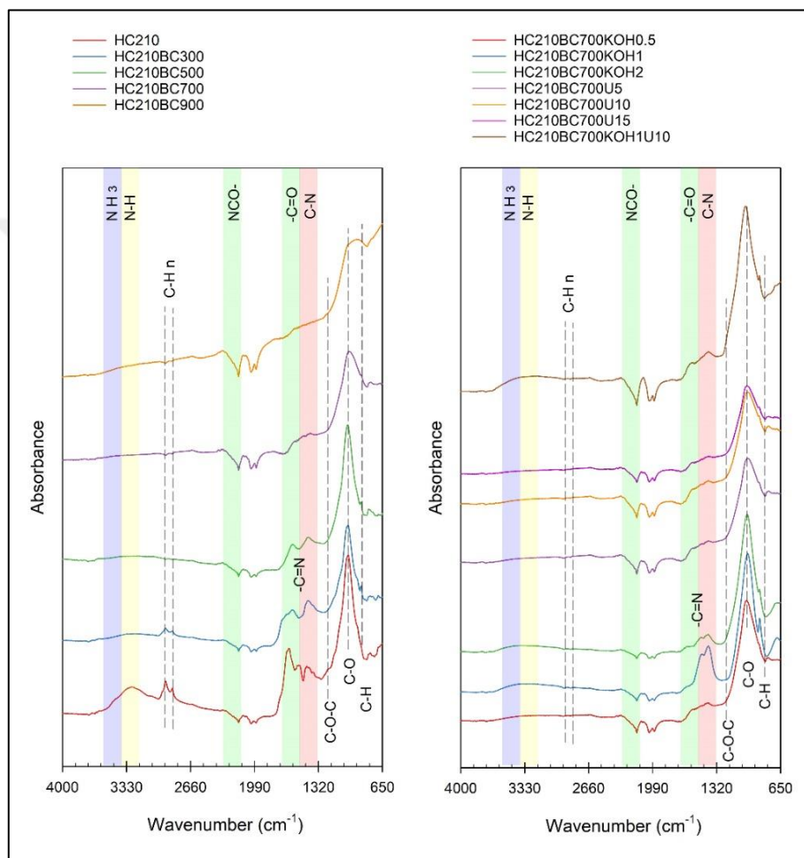
Figure 4.16. FTIR spectra of pristine and modified hydrothermally treated biochars
