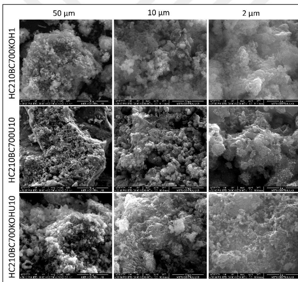
Figure 4.5. SEM images of hydrothermally treated and post-modified biochar materials
