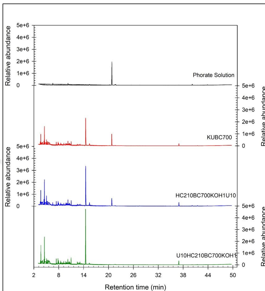
Figure 4.52. GS-MS chromatogram obtained for a phorate solution and phorate degradation by different biochar samples
