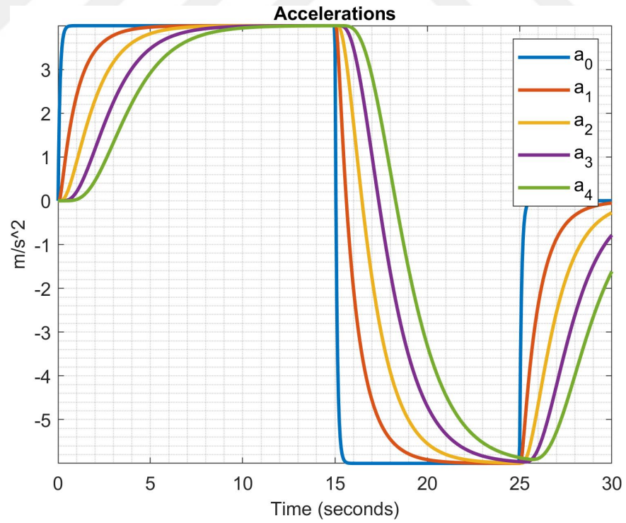
Figure 4.41: Case 6, Communication delay increased to \theta_i = 500ms
