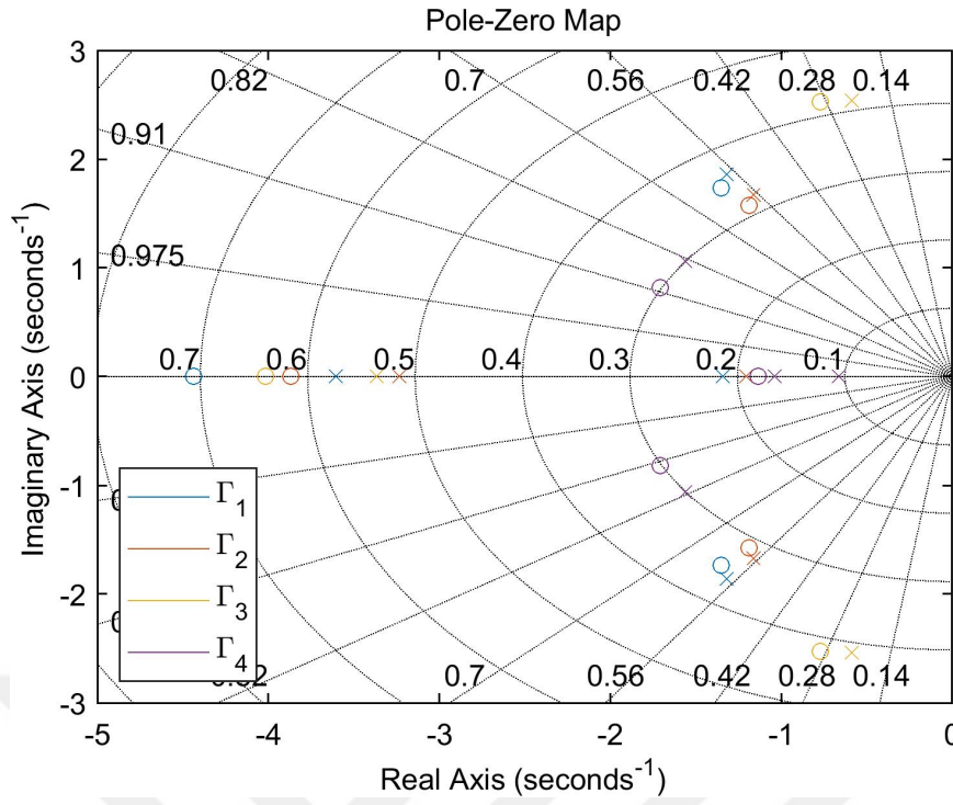
Figure 4.15: Pole-zero maps of heterogeneous string in Table 4.2 for case 3
