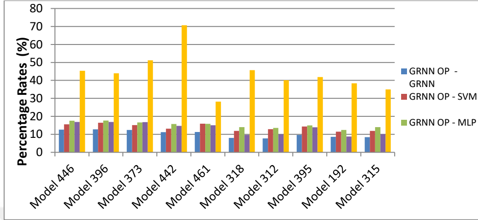
Figure 4.9. Percentage decrease rates in RMSE values of race time for OPGRNN-based models compared to RMSE values obtained by GRNN, SVM, MLP, SDT, and RBFNN-based models for quintuple combinations
