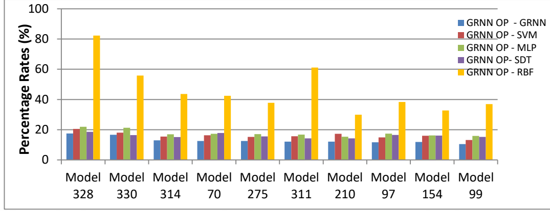
Figure 4.6. Percentage decrease rates in RMSE values of race time for OPGRNN-based models compared to RMSE values obtained by GRNN, SVM, MLP, SDT, and RBFNN-based models for quadruple combinations
