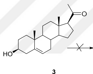
Figure 2.4. Incubation of 3 with P. citreo-viride [20].
