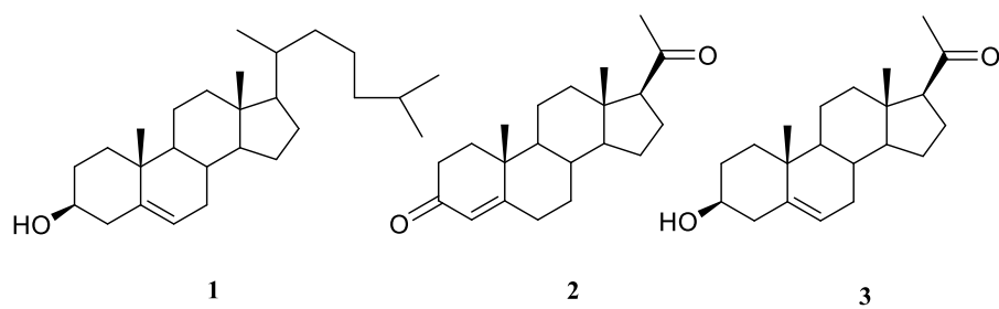
Figure 1.2. Structures of some important steroids [4-5]
