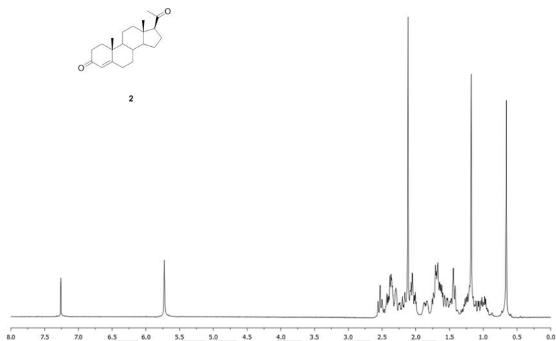
Figure A.1. ^1\text{H} NMR spectrum of compound 2.
