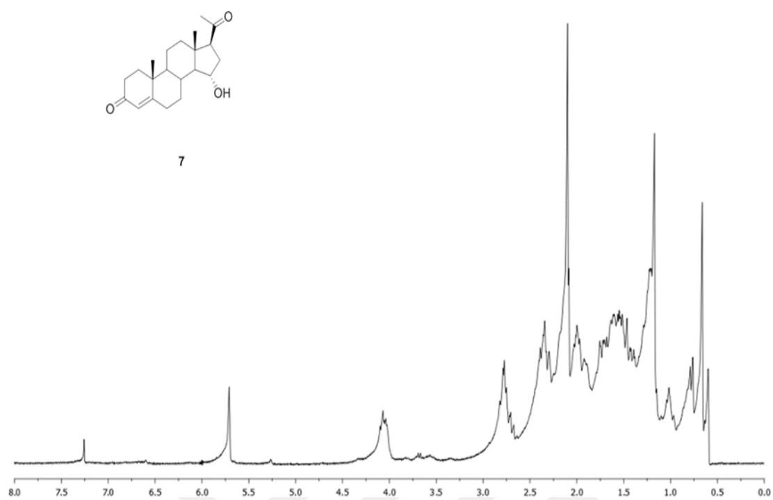
Figure A.5. ^1\text{H} NMR spectrum of compound 7
