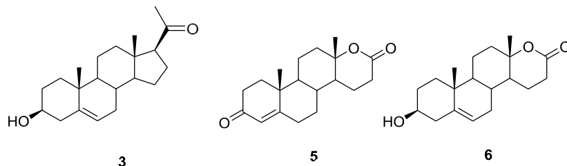
Figure 2.3. Incubation of 3 with some Penicillium species [17-19].
