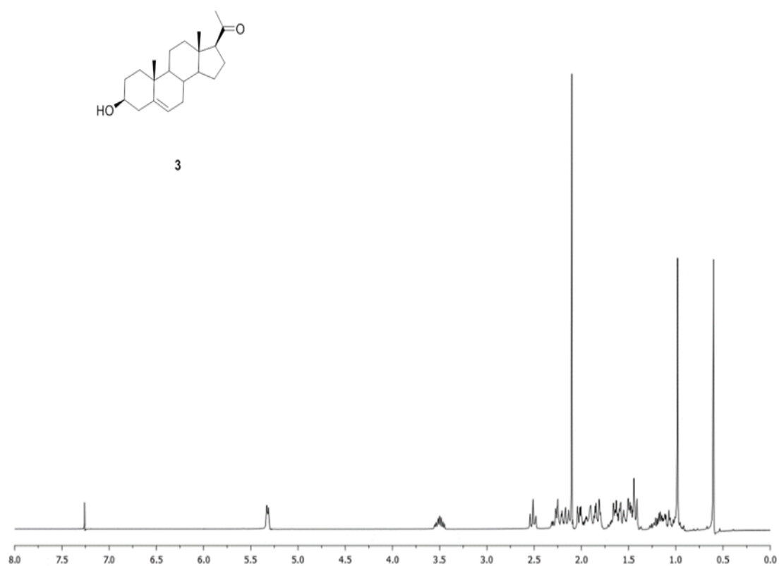
Figure A.3. ^1\text{H} NMR spectrum of compound 3
