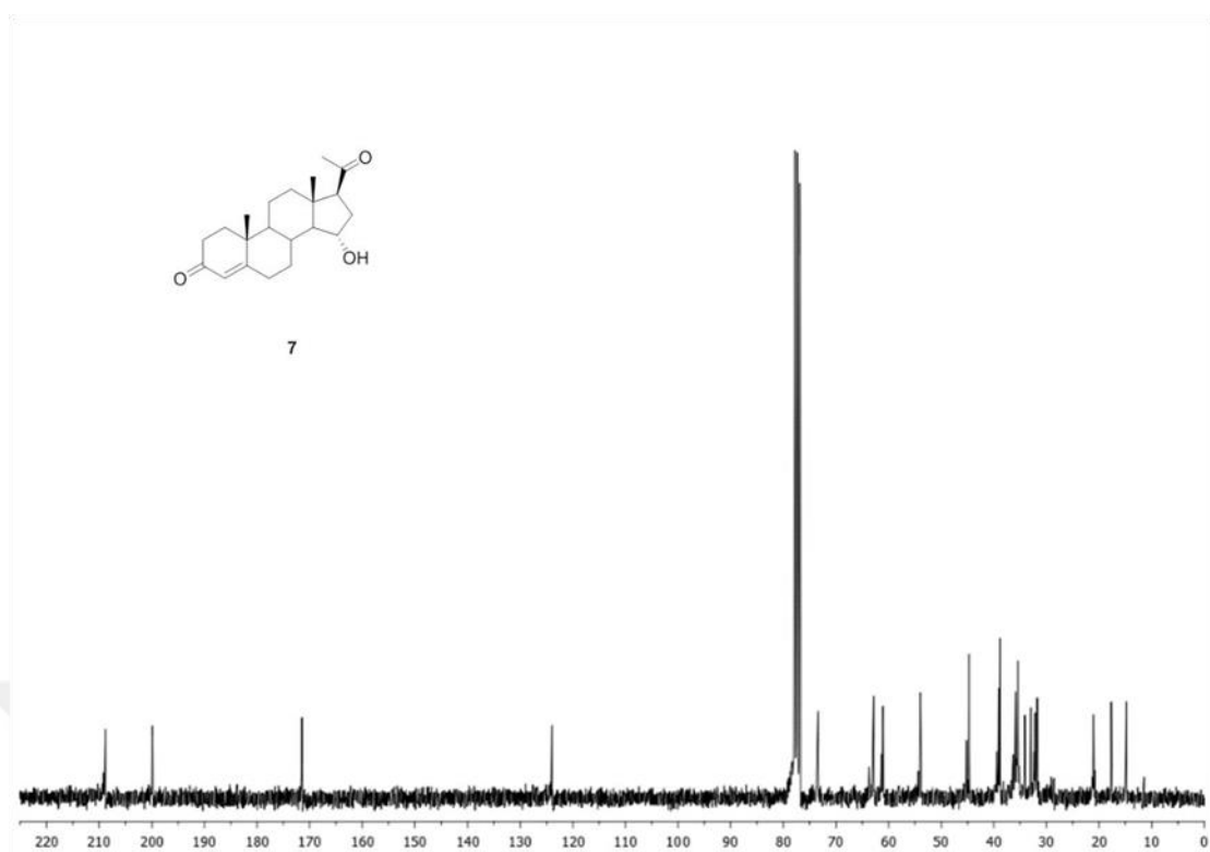
Figure A.6. ^{13}\text{C} NMR spectrum of compound 7
