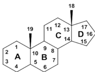
Figure 1.1. Cyclopentanoperhydrophenanthrene ring [4-5].
