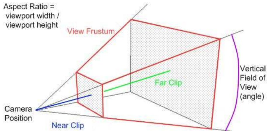
Figure 4.11. View frustum
