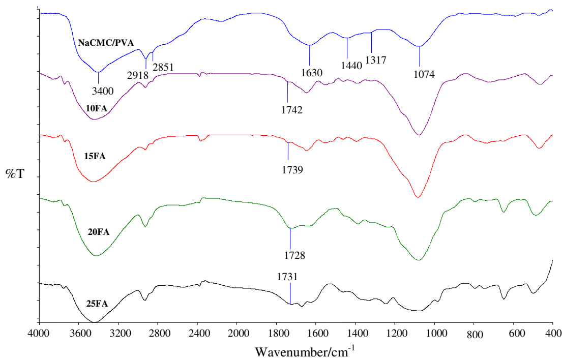
Figure 3.2 FTIR spectrum of the NaCMC7PVA blend, 10FA, 15FA, 20FA and 25FA.
