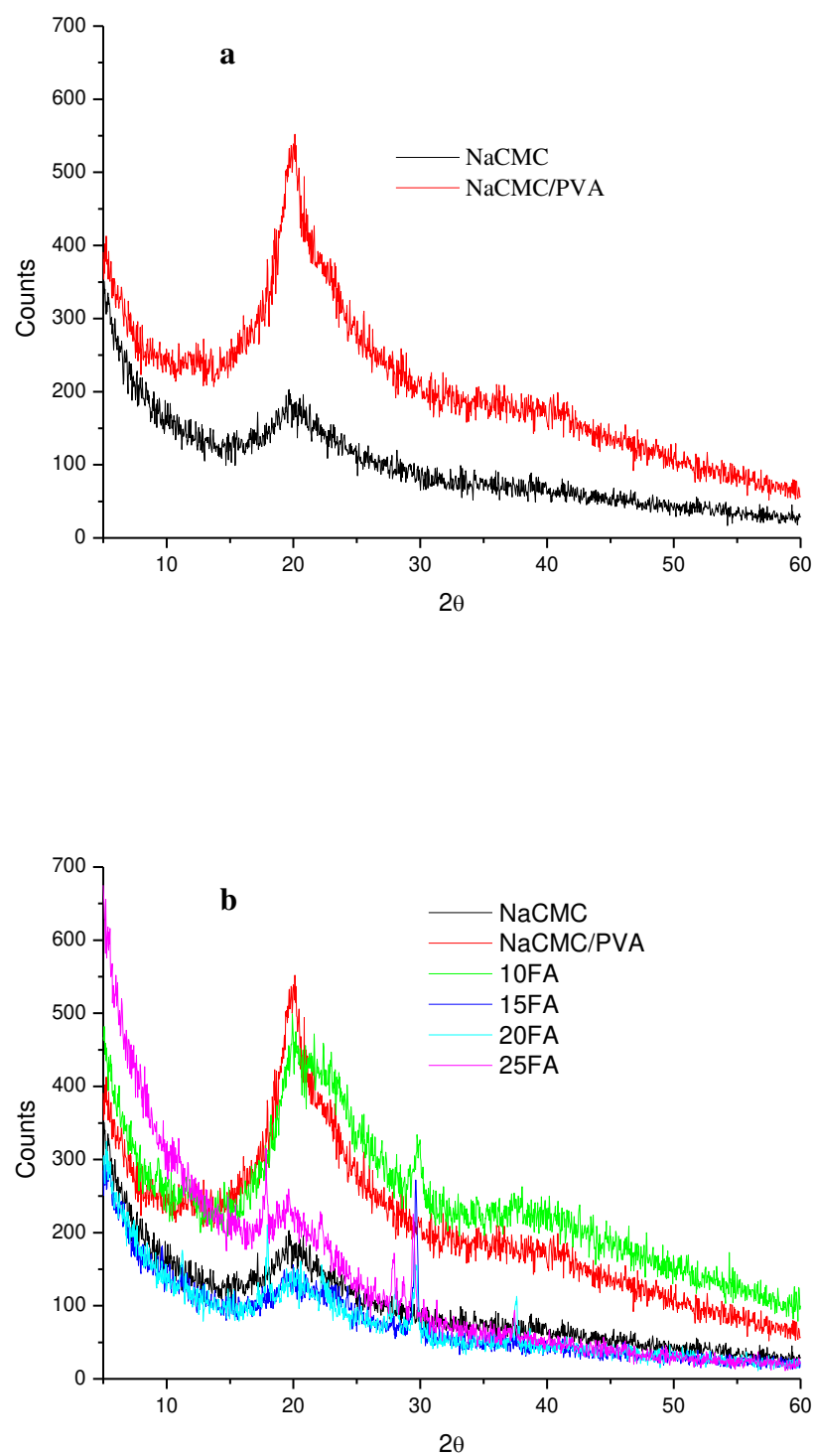
Figure 3.6 XRD pattern of the samples (a) NaCMC and NaCMC/PVA, (b) NaCMC, NaCMC/PVA and hydrogels.
