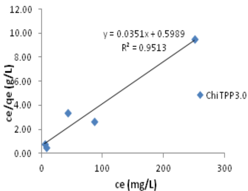
Figure 25: Langmuir plot of chi tpp 3.0
