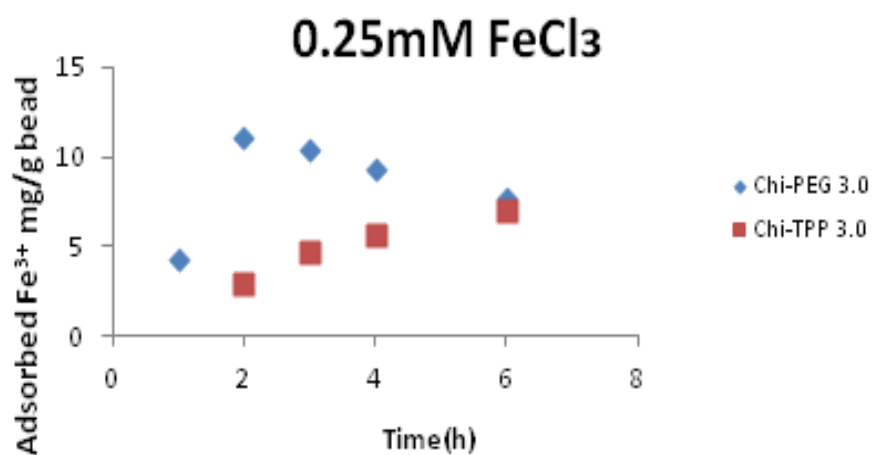
Figure 23: \text{Fe}^{3+} adsorption mg/g of bead in 0.25mM \text{FeCl}_3 with time at pH 3.0
