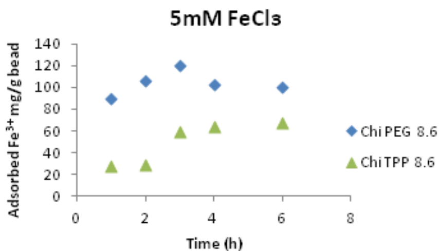
Figure 14: \text{Fe}^{3+} adsorption mg/g of bead in 5mM \text{FeCl}_3 with time at pH 8.6
