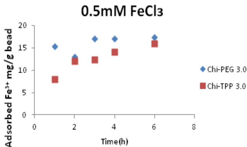
Figure 22: \text{Fe}^{3+} adsorption mg/g of bead in 0.5mM \text{FeCl}_3 with time at pH 3.0
