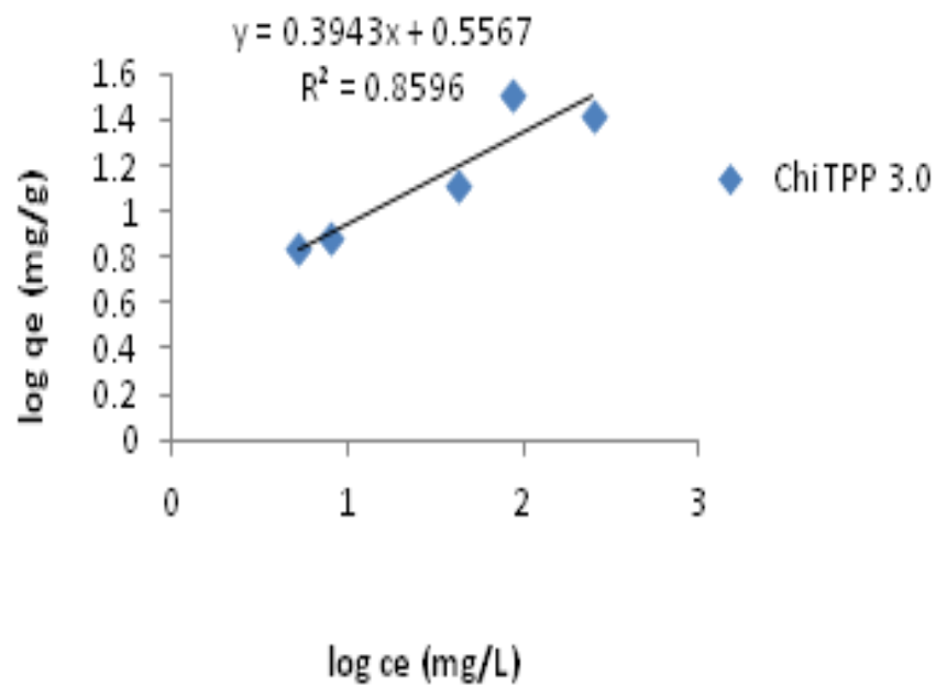
Figure 29: Freudlich plot of chi tpp 3.0
