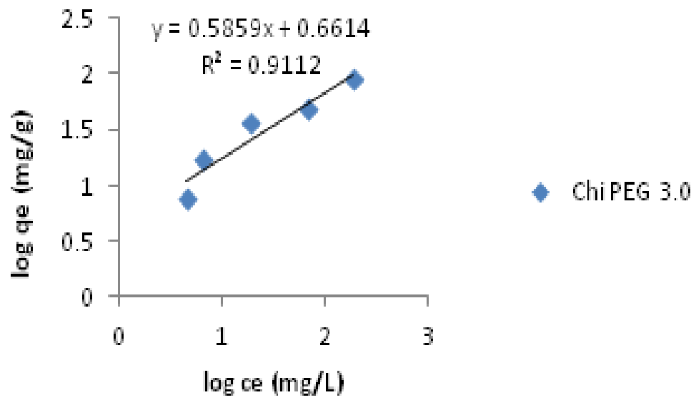
Figure 28: Freudlich plot of chi peg 3.0
