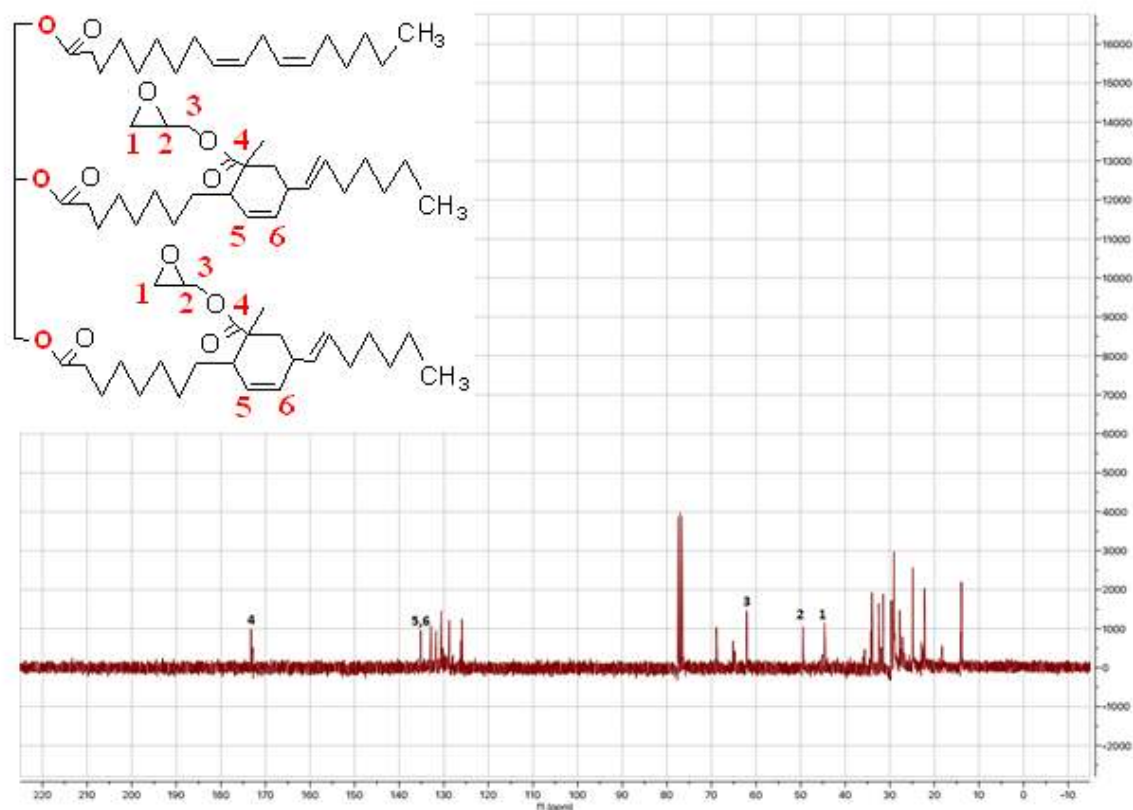
Figure 22b. ^{13}\text{C} -NMR Spectra of Epoxized-Tung Oil (ETO)
