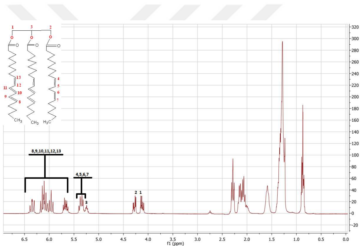
Figure 21a. ^1\text{H} -NMR Spectra of Tung Oil
