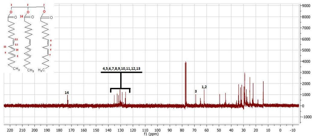
Figure 21b. ^{13}\text{C} -NMR Spectra of Tung Oil
