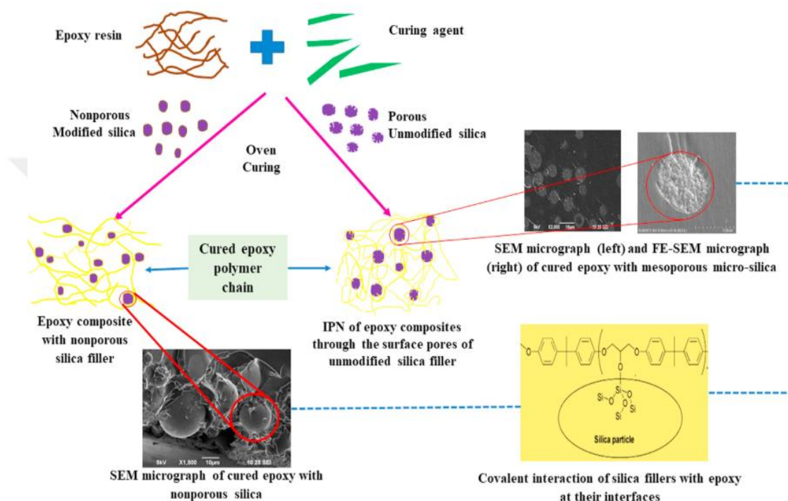
Figure 14. Schematic Description by Including Nano/Micro Filler of The Production of The Polymeric Resin Composite Epoxy.
