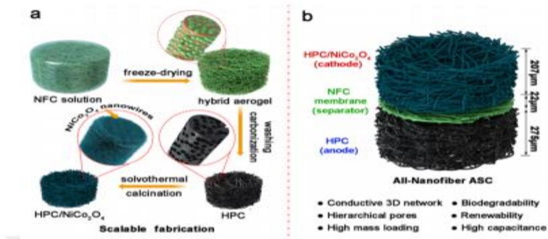
Figure 16. (A) Nanocellulose-Derived Aerogels for Nanocellulose Manufacturing (HPC / NiCo 2 O 4 ).
