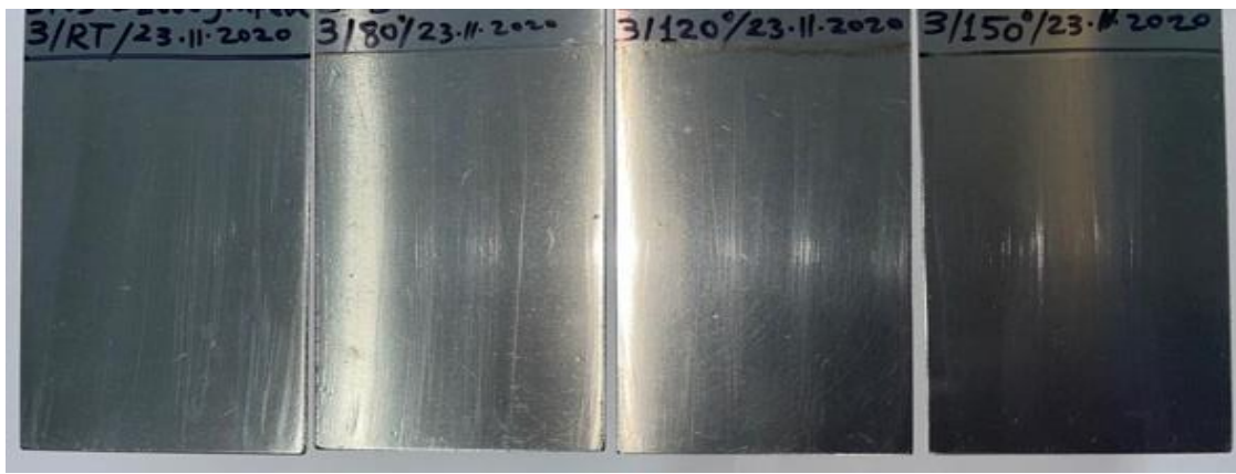
Figure 20. Pictures of ETO-ED900 Coatings (Views of Graphene-Doped Nanocomposite Coatings from Left to Right, at 25°C, 80 °C, 120 °C and 150 °C, Respectively)
