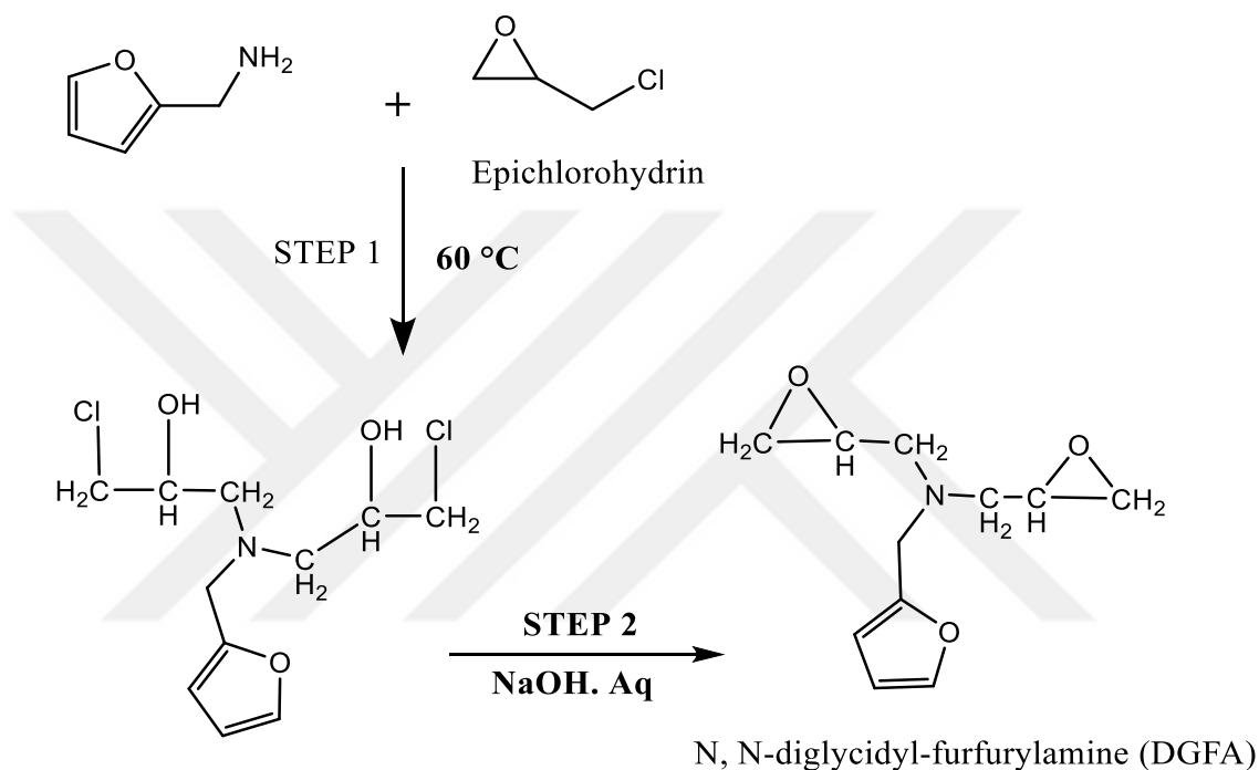
Scheme 20. Synthesis of N, N-Diglycidyl-Furfurylamine (DGFA) By 2 Steps.
