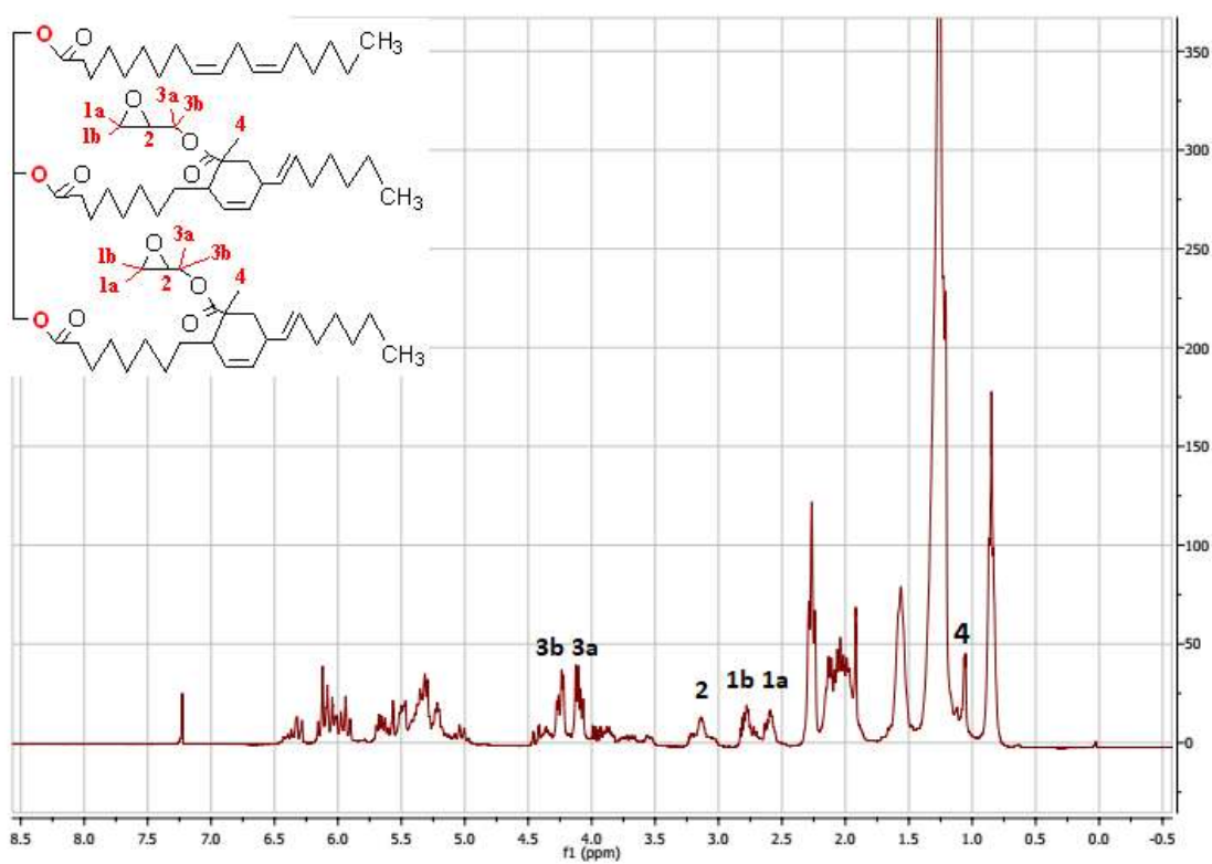
Figure 22a. ^1\text{H} -NMR Spectra of Epoxidized-Tung Oil (ETO)
