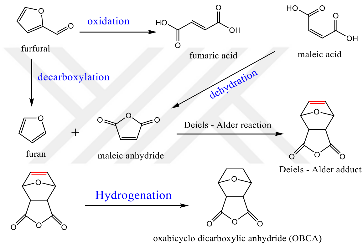
Scheme 12. Synthesis of Furfural-Based Curing Agent (OBCA)
