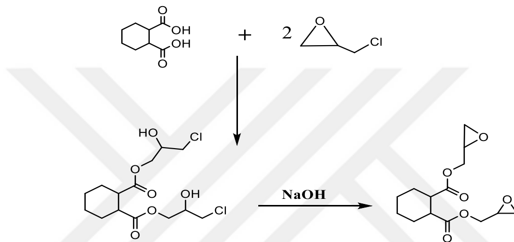
Scheme 8. Synthesis of Diglycidyl Ester of Hexahydrophthalic Acid
