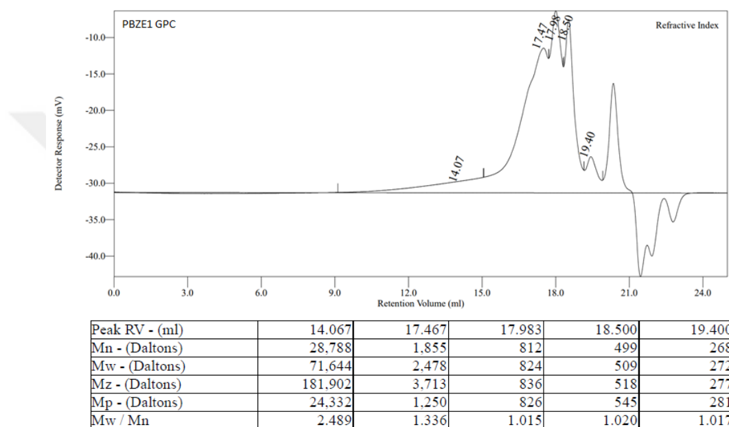
Figure 4.8. GPC measurement results for PBZE1 polymer [201]
