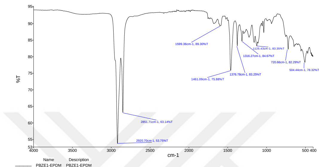
Figure 4.33. The FTIR spectrum of PBZE1-EPDM
