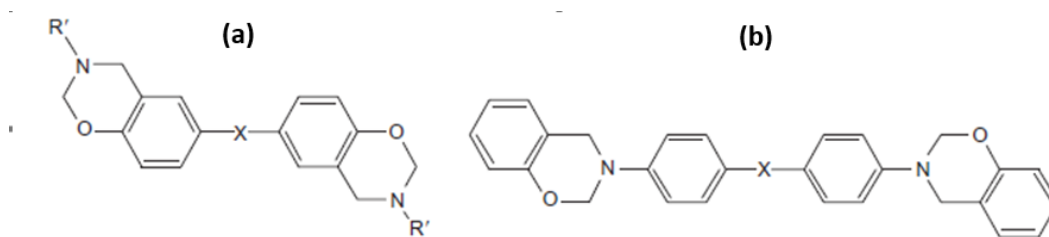
Figure 3.3. Different combinations of a bifunctional phenol and primary amine
