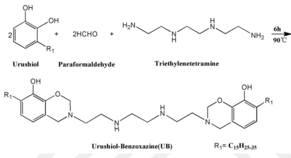
Figure 3.8. Synthesis of urushiol BZ [142]
