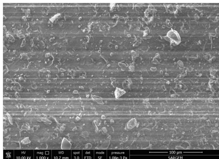
Figure 4.13. SEM image of PBZE1-EPDM-PTFE-Nano \text{TiO}_2 -S polymer nanocomposite sample
