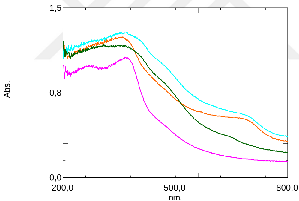
Figure 4.32. The compare of UV-vis. analysis for PBZE1-EPDM-PTFE-Nano \text{TiO}_2 nanocomposite samples with sulfur
