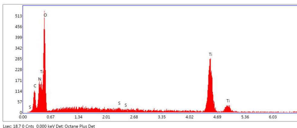
Figure 4.24. EDX spectrum elemental analysis for PBZE1-EPDM-PTFE-Nano \text{TiO}_2 -S-180 polymer nanocomposite sample
