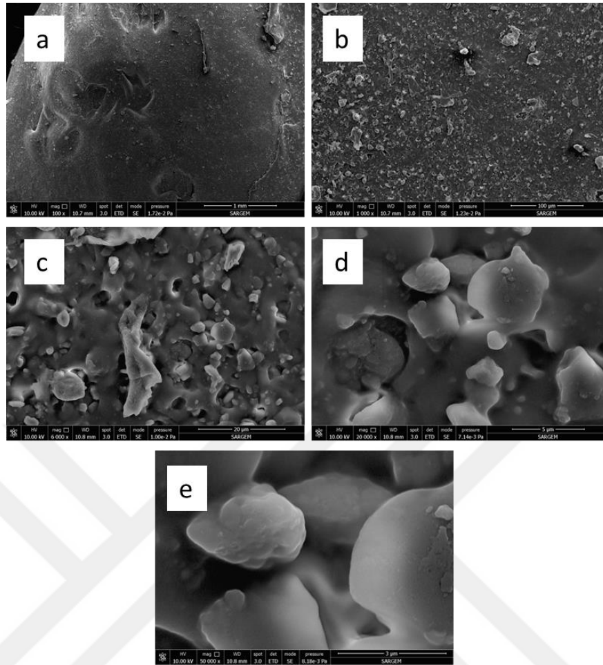
Figure 4.12. SEM images of PBZE1-EPDM-PTFE-Nano \text{TiO}_2 zoomed a) 100x times b) 1000x times c) 6000x times d) 20000x times e) 50000x times
