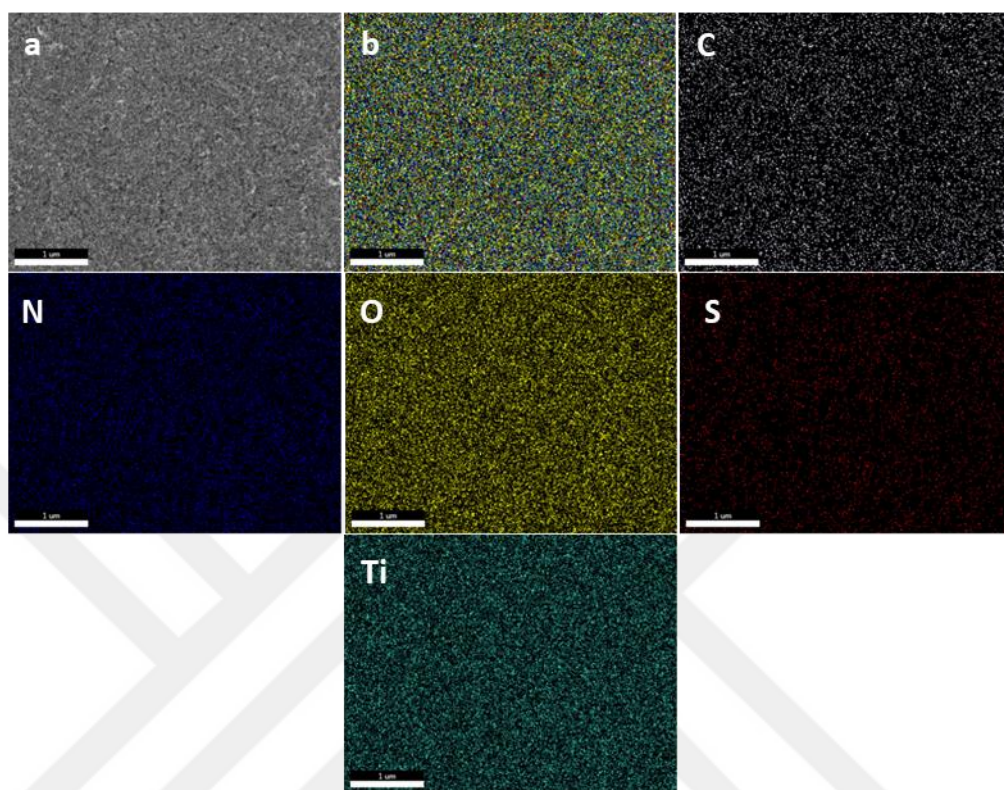
Figure 4.23. For PBZE1-EPDM-PTFE-Nano \text{TiO}_2 -S-180 polymer nanocomposite sample a) SEM image b) SEM-EDX and C, N, O, S, Ti element respectively
