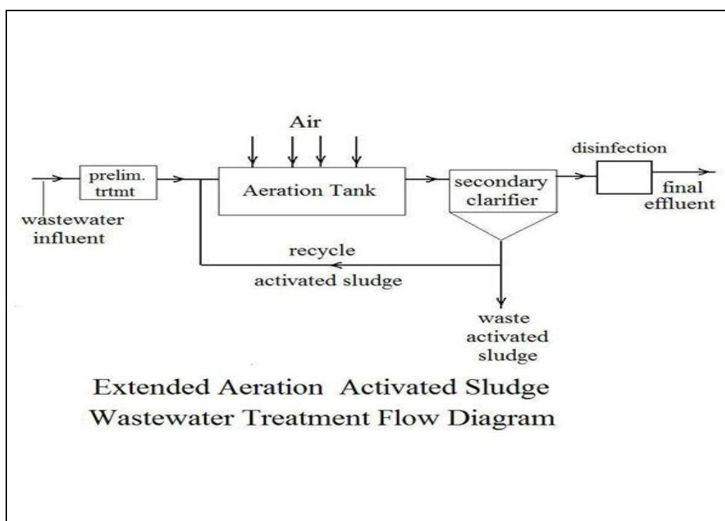
Figure 2.2 EAAS wastewater treatment flow scheme (Source: www.brighthub.com , 2012)
