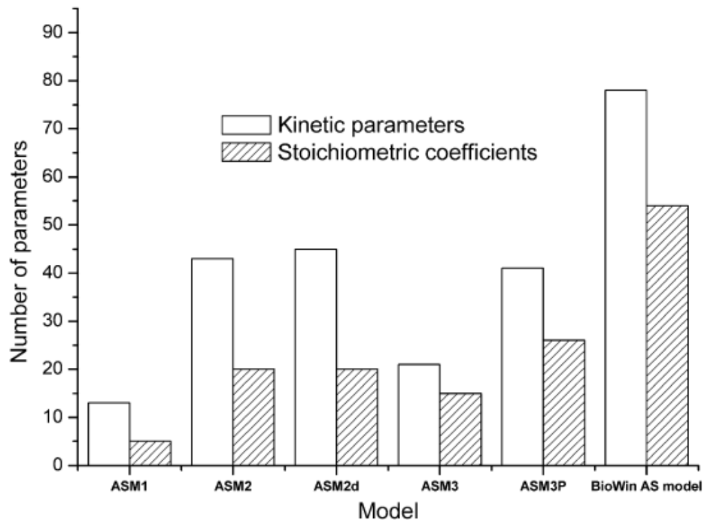
Figure 2.6 The changes of the number of parameters within ASMs development (Source: Liwarska-Bizukojs and Biernacki, 2010)
