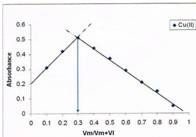
Figure 3.22: Jobe's Method for Absorbance of Cu (II)-BrTAMP at 647 nm.
