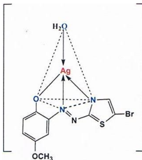
Figure 3.29: The Proposed Structural Formula of Ag (I) - BrTAMP Complex
