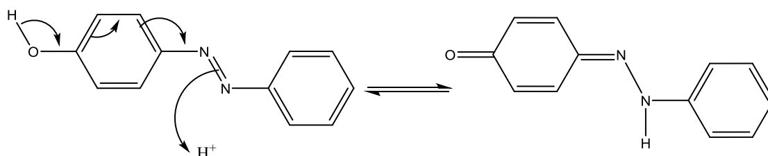
Scheme 1.2: Tautomerisim of Azo Dyes.
