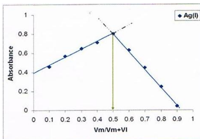
Figure 3.24: Jobe's Method for Absorbance of Ag (I)-BrTAMP at 518 nm
