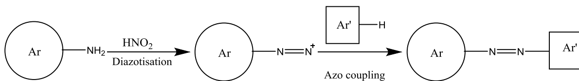
Scheme 1.3: General Reaction for the Synthesis of Azo Dyes
