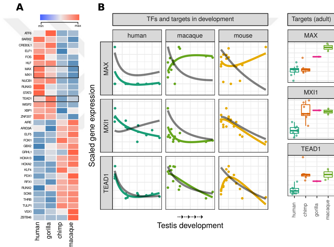
Figure 3.16: Results of transcription factor binding site enrichment analysis. (A) Bulk testis gene expression of enriched TFs in cluster #1 and showing convergent gene expression across human, chimpanzee, gorilla and macaque. (B) Gene expression profiles of selected TFs (marked with rectangles on pane A) and their target genes, throughout testis development (left) and adult bulk testis transcriptomes (right).
