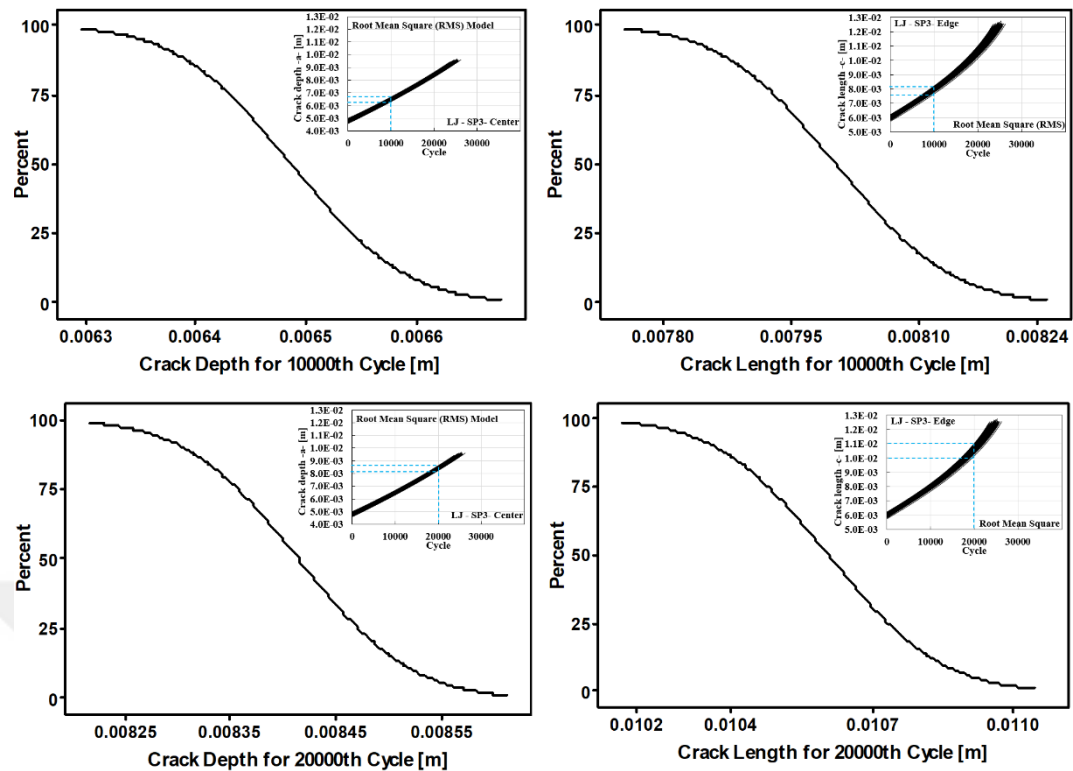
Figure 5.148. CDF for crack lengths under constant cycle load conditions (LJ specimen, SP3 loading spectrum, Root mean square model)
