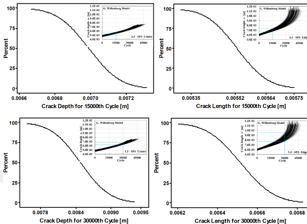
Figure 5.144. CDF for crack lengths under constant cycle load conditions (LJ specimen, SP3 loading spectrum, Generalized Willenborg model)
