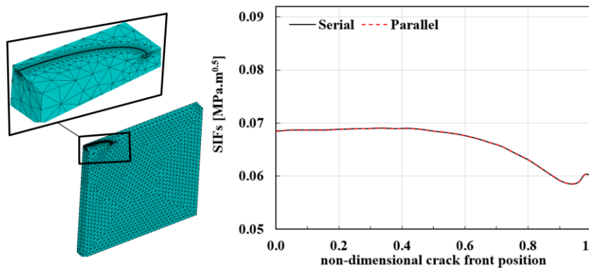
Figure 2.9. Surface crack in a finite thickness plate, a/c = 0.33 (Case 4)
