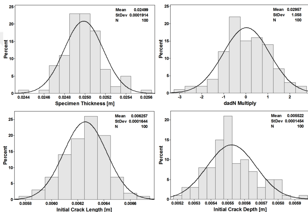
Figure 5.78. Distributions of the inputs used in crack growth life analysis (LJ specimen, SP1 loading spectrum, Wheeler model with Walker)
