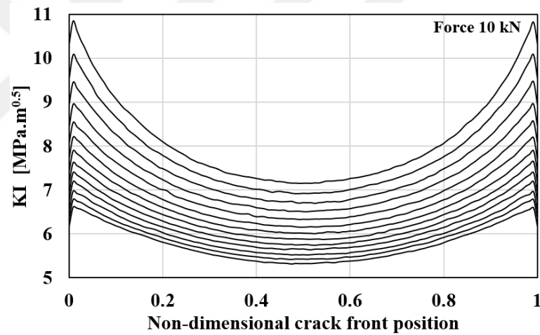
Figure 4.23. KI SIFs for LJ specimen calculated by FCPAS
