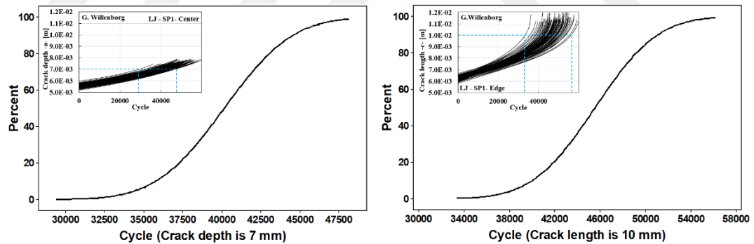
Figure 5.88. CDF for load cycles under constant crack length conditions (LJ specimen, SP1 loading spectrum, Generalized Willenborg model)
