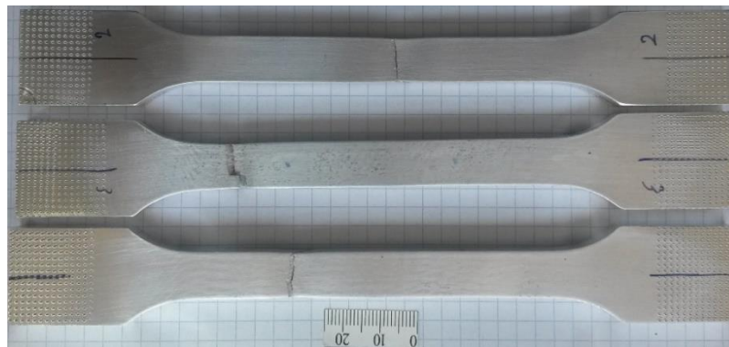
Figure 3.2. View of specimens after tensile testing
