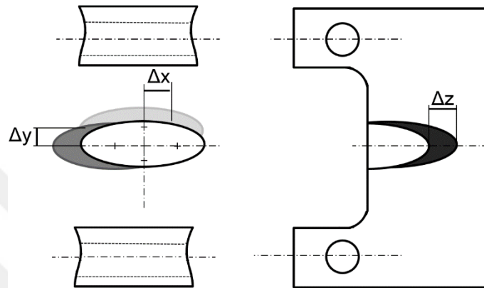
Figure 4.13. Offsets of the ellipsoid notch
