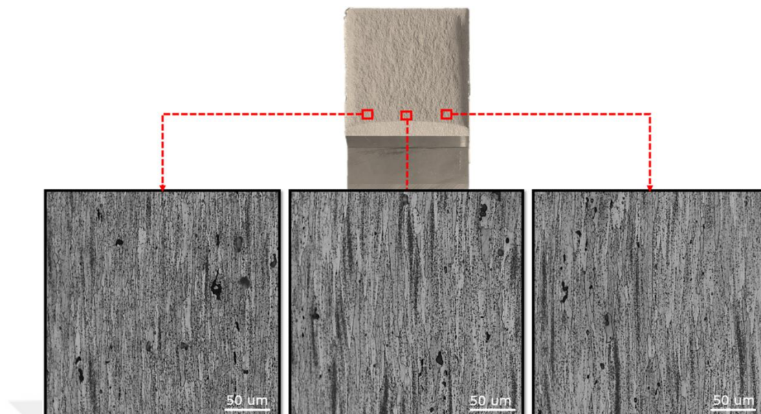
Figure 4.46. Optical microscopy images of marked regions of the 1st CT specimen in Figure 4.44
