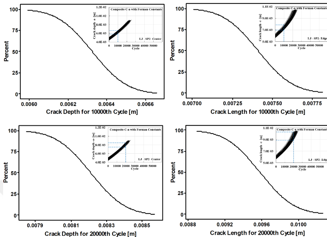
Figure 5.95. CDF for crack lengths under constant cycle load conditions (LJ specimen, SP2 loading spectrum, Composite C-n with Forman Constants)
