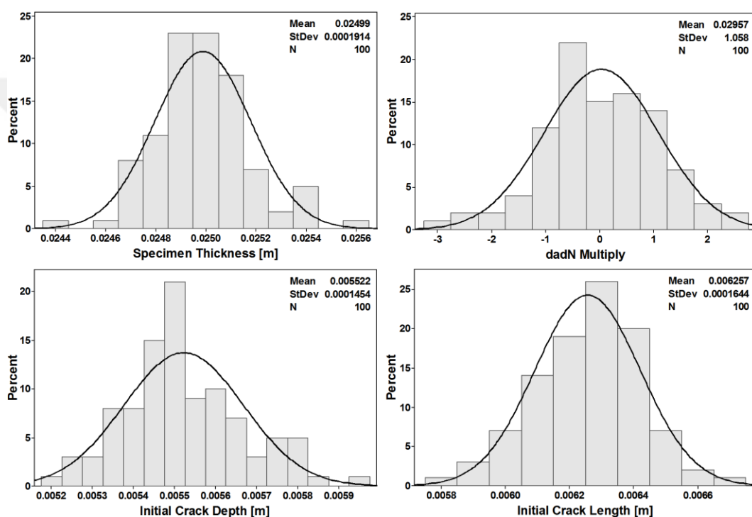
Figure 5.82. Distributions of the inputs used in crack growth life analysis (LJspecimen, SP1 loading spectrum, Xiaoping model)
