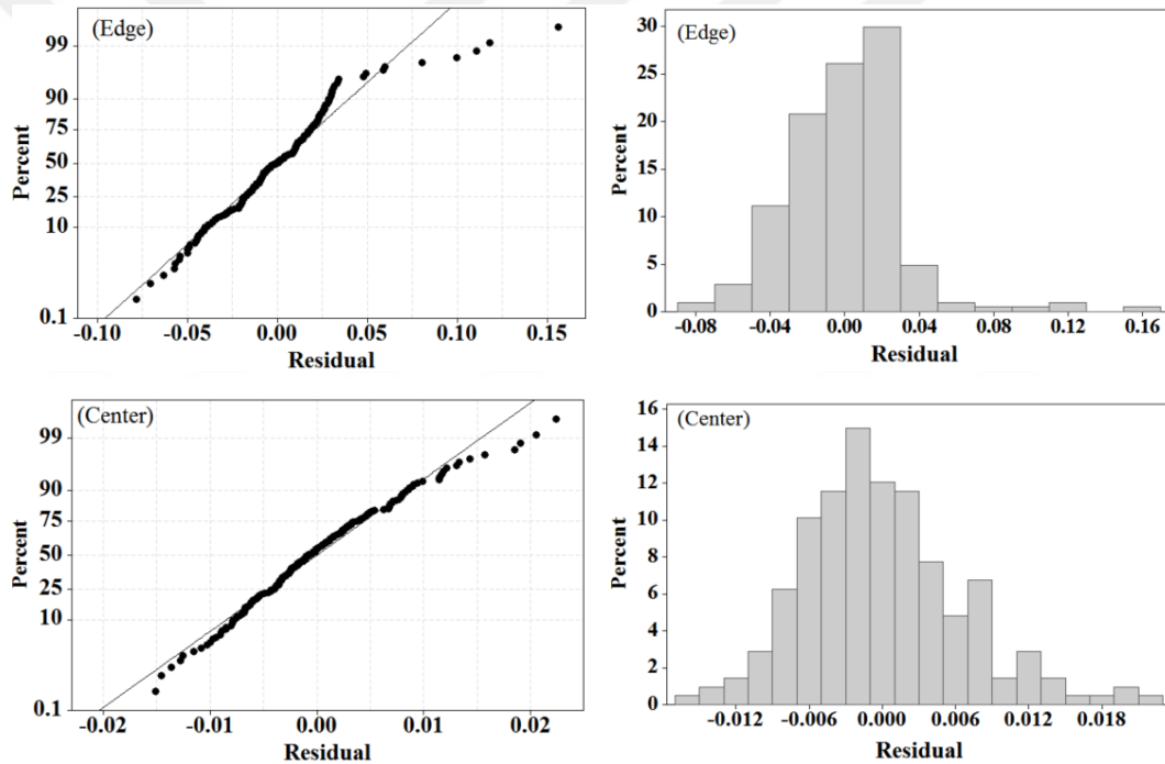
Figure 4.21. Residual plots for transfer functions
