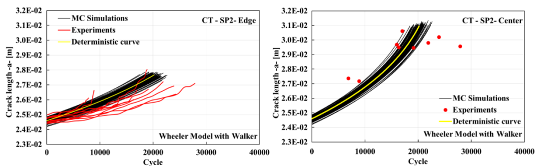
Figure 5.49. Probabilistic crack growth life curves and their comparison with the experiments (CT specimen, SP2 loading spectrum, Wheeler model with Walker)
