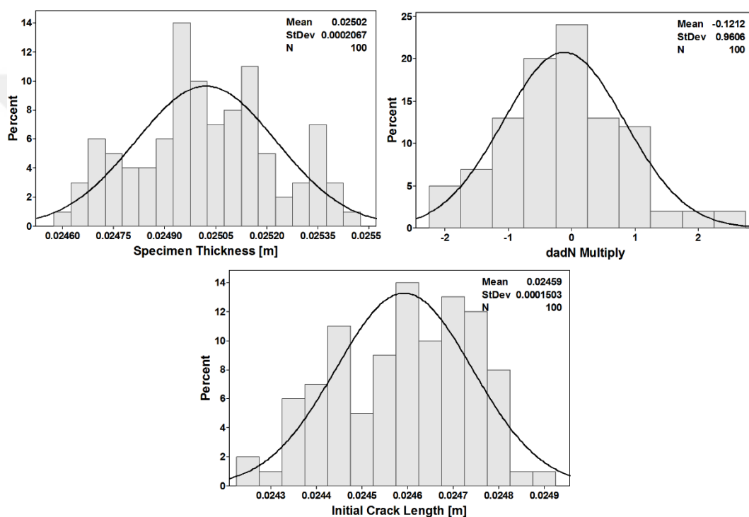
Figure 5.46. Distributions of the inputs used in crack growth life analysis (CT specimen, SP2 loading spectrum, Wheeler model with Forman)
