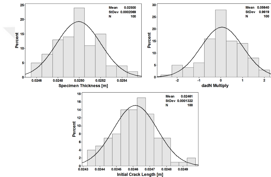
Figure 5.62. Distributions of the inputs used in crack growth life analysis (CT specimen, SP2 loading spectrum, Root mean square model)
