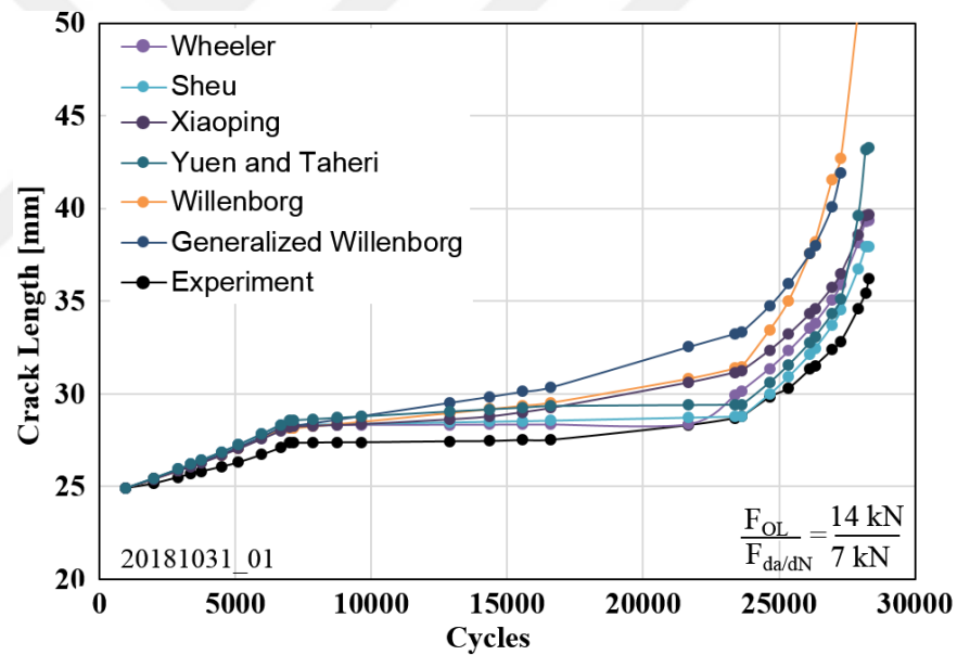
Figure 3.43. Comparison of variable amplitude loading models for F_{OL}/F_{da/dN} = 2.0 overload ratio
