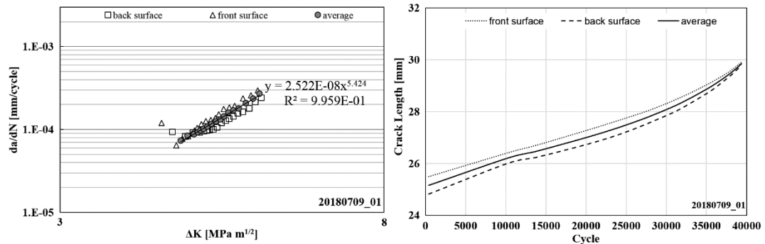
Figure 3.15. Crack growth curves, R = 0.8
