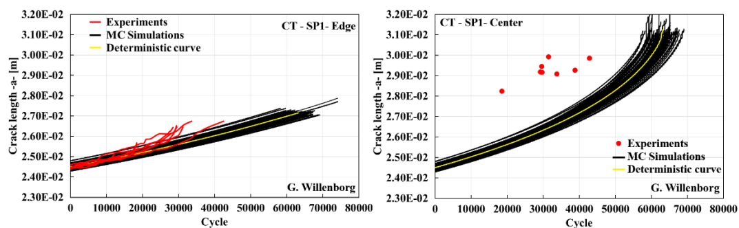
Figure 5.29. Probabilistic crack growth life curves and their comparison with the experiments (CT specimen, SP1 loading spectrum, Generalized Willenborg model)
