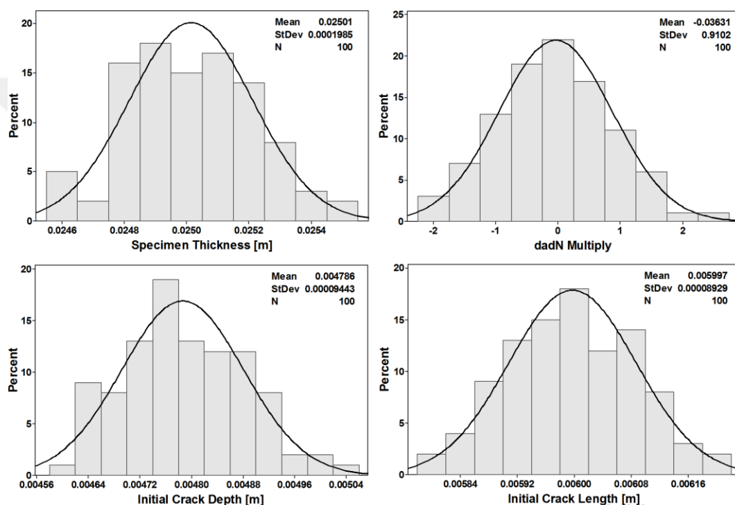
Figure 5.143. Distributions of the inputs used in crack growth life analysis (LJ specimen, SP3 loading spectrum, Generalized Willenborg model)
