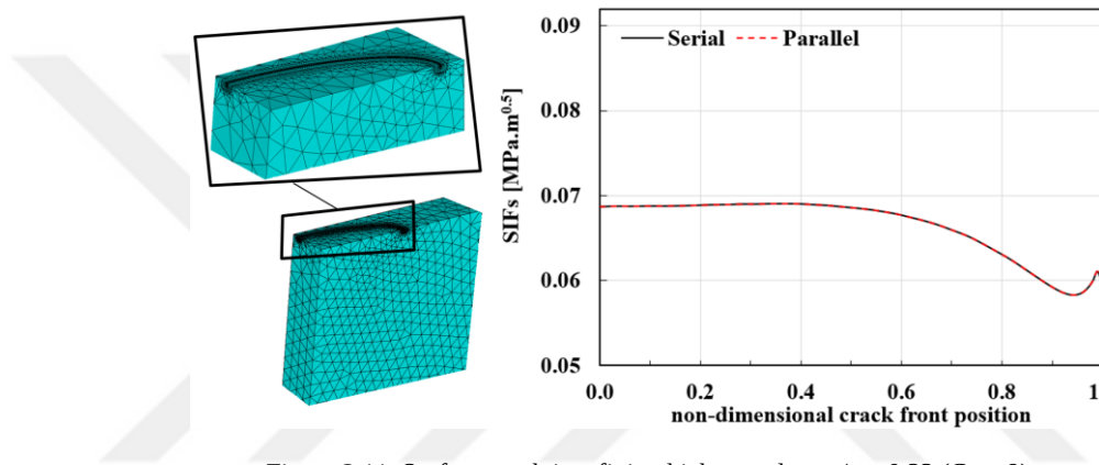
Figure 2.11. Surface crack in a finite thickness plate, a/c = 0.33 (Case 9)
