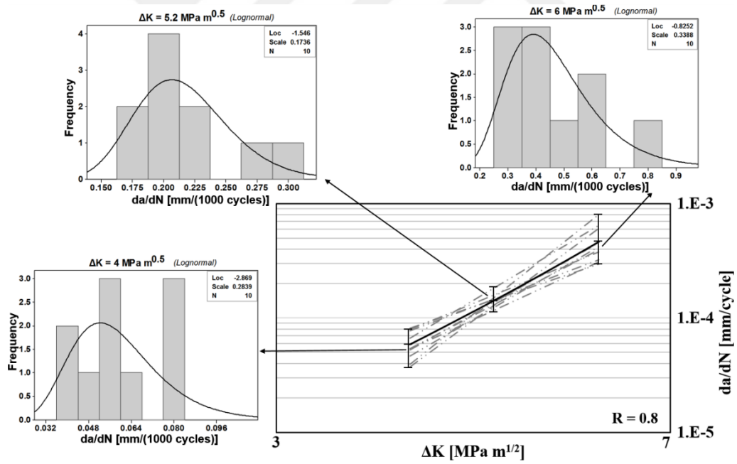
Figure 3.19. da/dN variations under constant amplitude loading, R = 0.8
