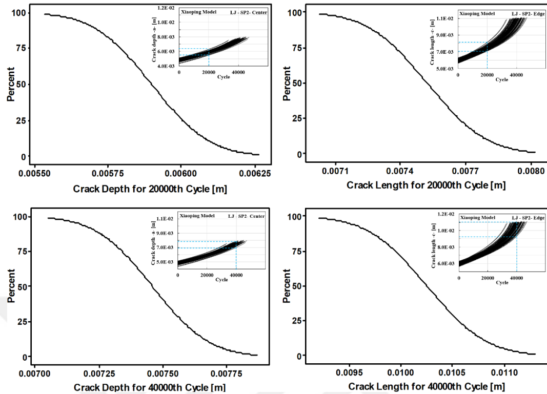
Figure 5.111. CDF for crack lengths under constant cycle load conditions (LJ specimen, SP2 loading spectrum, Xiaoping model)
