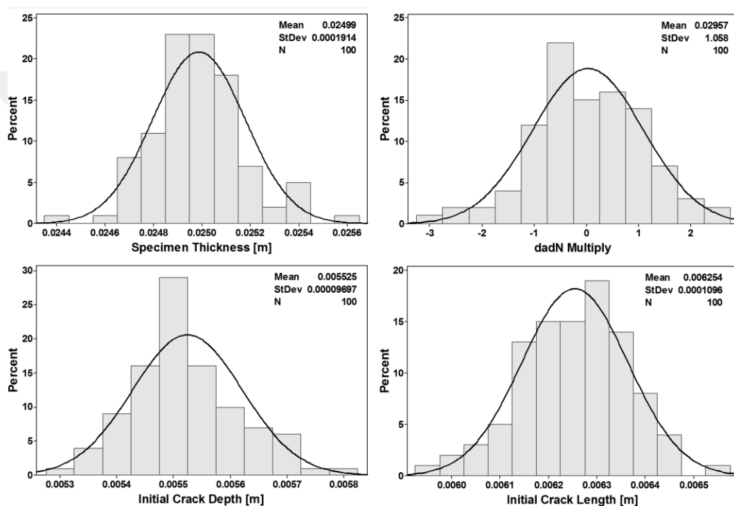
Figure 5.66. Distributions of the inputs used in crack growth life analysis (LJ specimen, SP1 loading spectrum, Composite C-n with Forman Constants)
