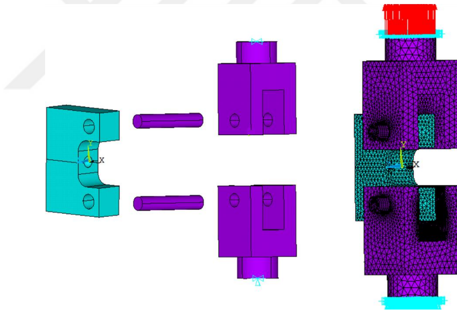
Figure 4.6. Lee James specimen, loading apparatus and applied boundary conditions for elasto-plastic analysis
