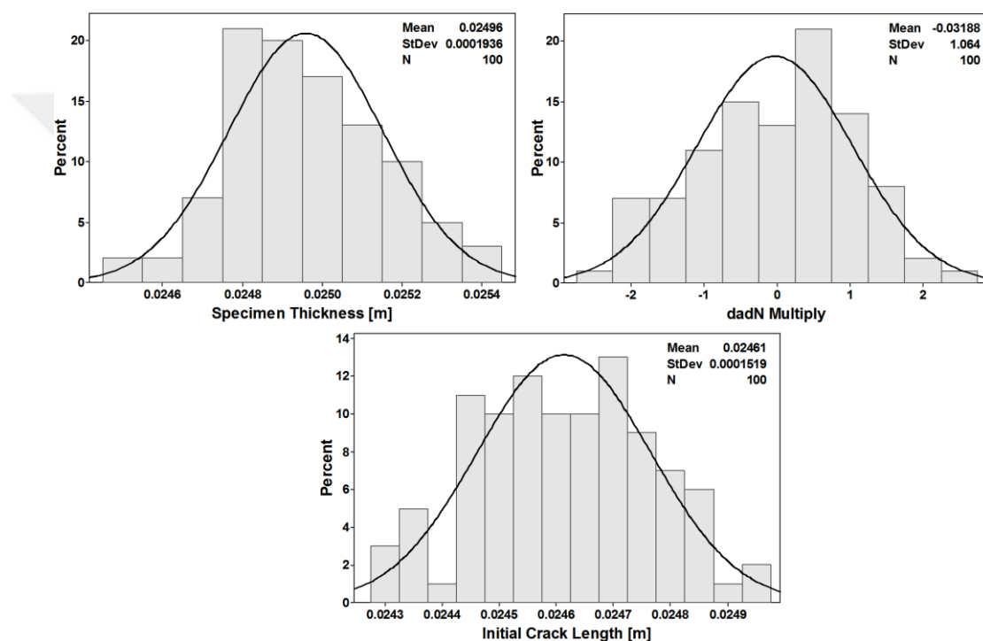
Figure 5.54. Distributions of the inputs used in crack growth life analysis (CT specimen, SP2 loading spectrum, Xiaoping model)
