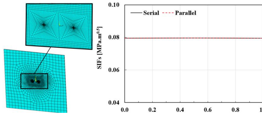
Figure 2.7. Central crack on a functionally graded material (Case 2)
