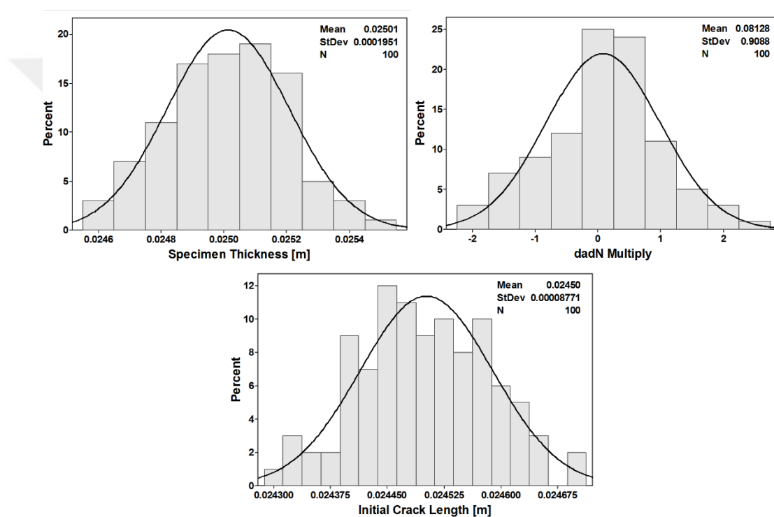
Figure 5.26. Distributions of the inputs used in crack growth life analysis (CT specimen, SP1 loading spectrum, Xiaoping model)
