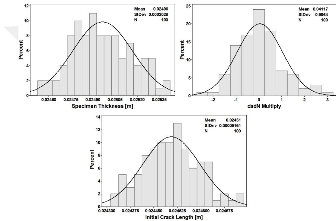
Figure 5.22. Distributions of the inputs used in crack growth life analysis (CT specimen, SP1 loading spectrum, Wheeler model with Walker)
