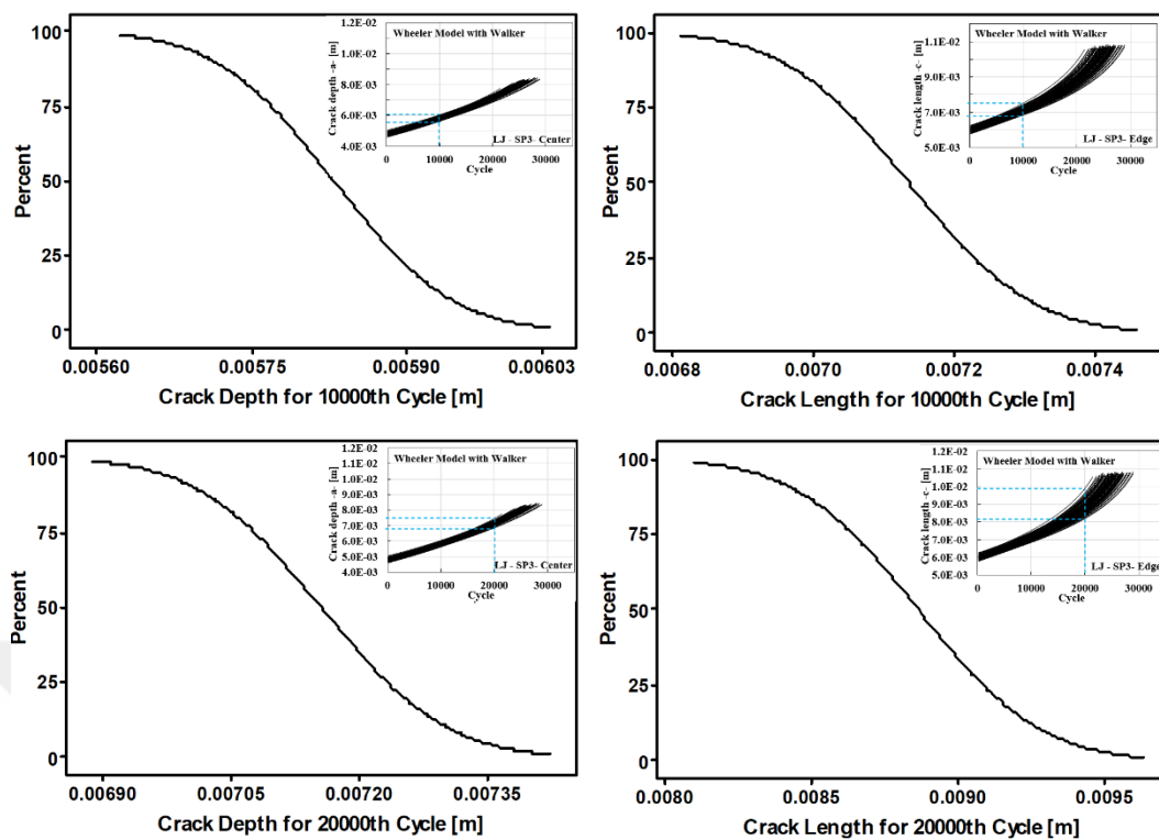
Figure 5.136. CDF for crack lengths under constant cycle load conditions (LJ specimen, SP3 loading spectrum, Wheeler model with Walker)
