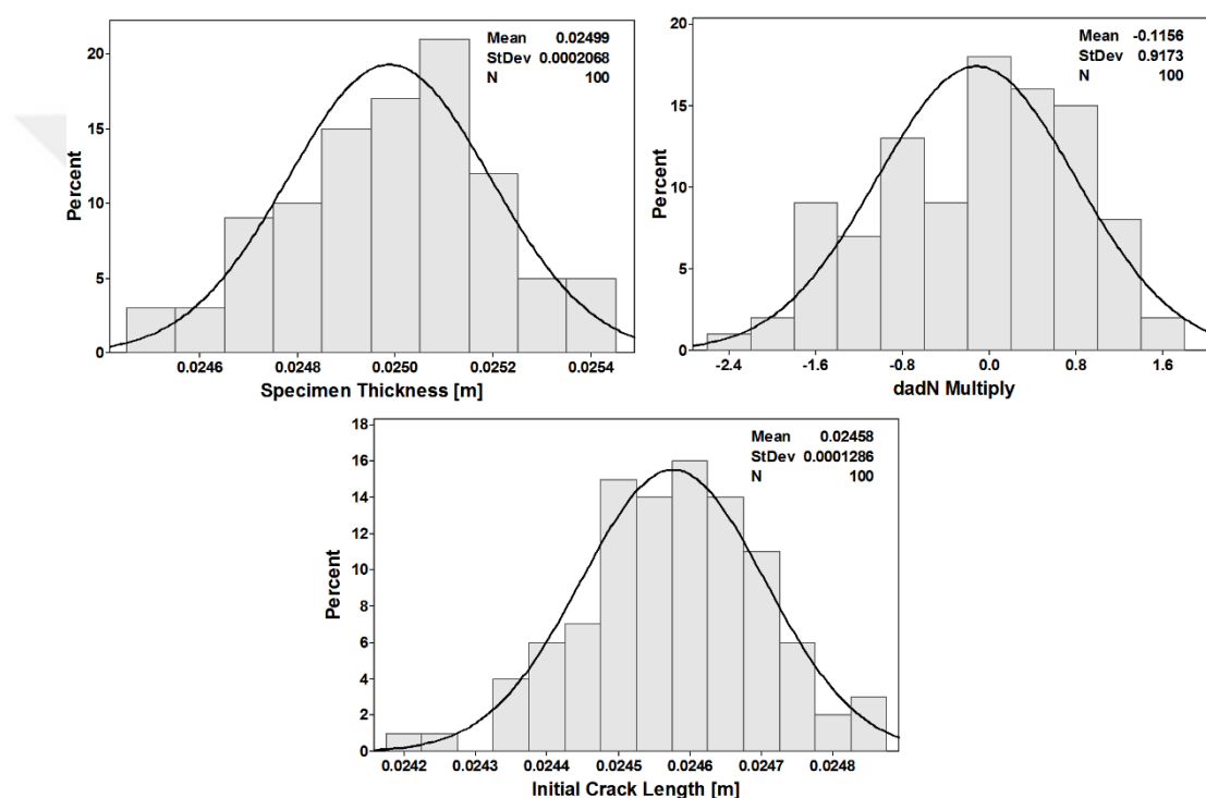
Figure 5.50. Distributions of the inputs used in crack growth life analysis (CT specimen, SP2 loading spectrum, Wheeler model with Walker)
