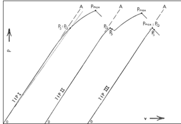
Figure 3.4. Typical force-displacement curves obtained from fracture toughness tests [36]
