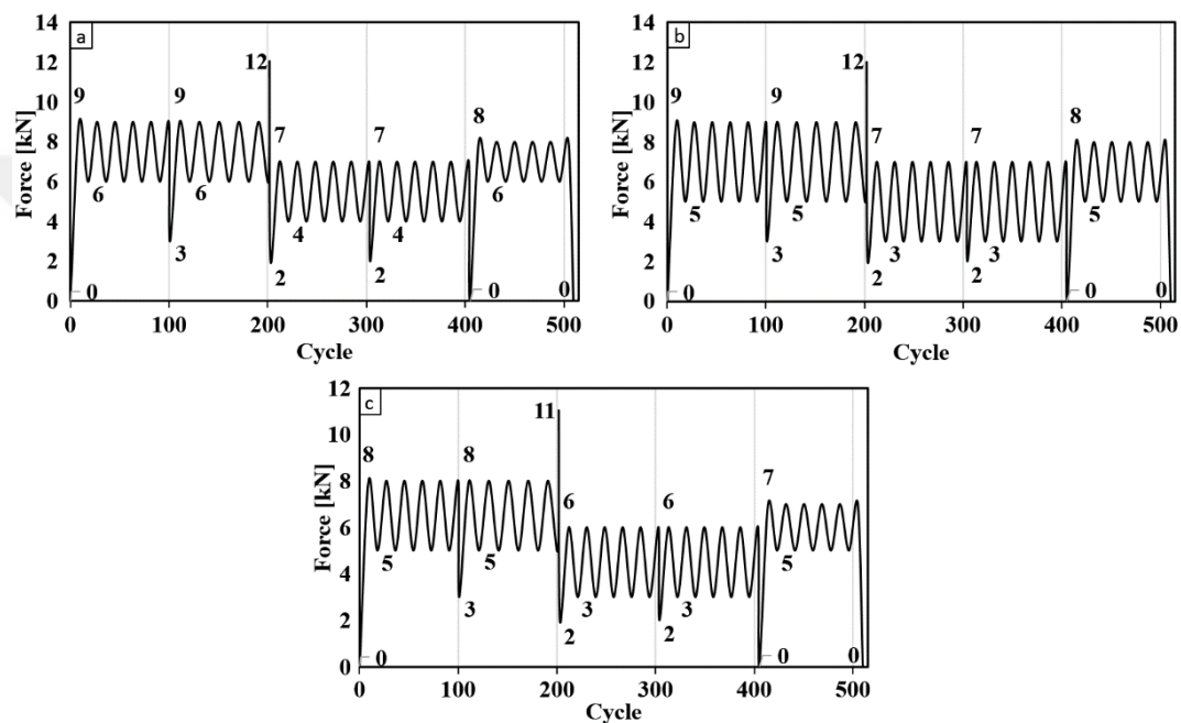
Figure 3.24. Random loading spectrum-1 (SP1)
