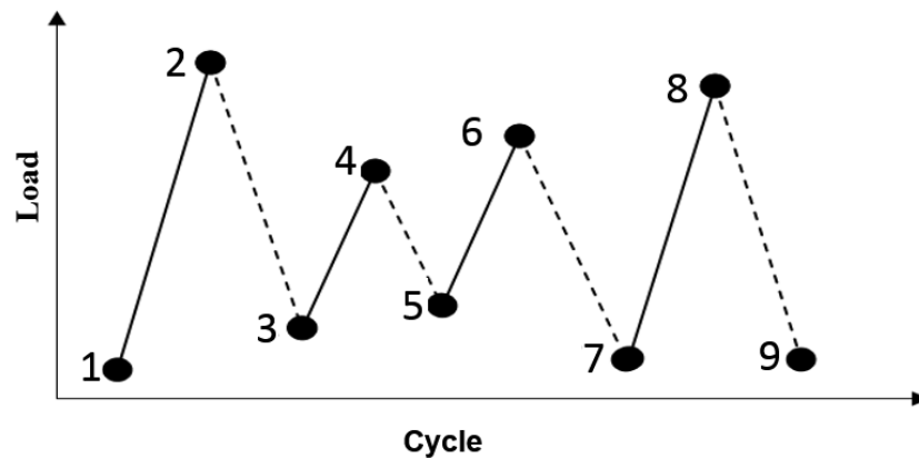
Figure 3.48. Definition of spectrum profile positions
