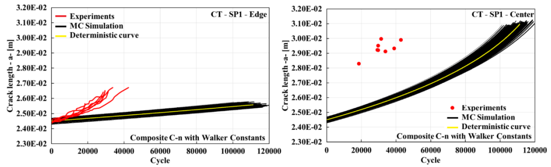
Figure 5.13. Probabilistic crack growth life curves and their comparison with the experiments (CT specimen, SP1 loading spectrum, Composite C-n with Walker Constants)
