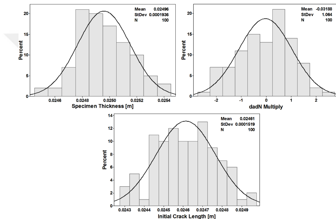
Figure 5.38. Distributions of the inputs used in crack growth life analysis (CT specimen, SP2 loading spectrum, Composite C-n with Forman Constants)
