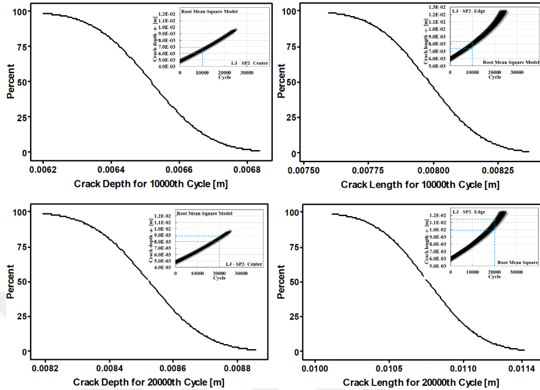
Figure 5.119. CDF for crack lengths under constant cycle load conditions (LJ specimen, SP2 loading spectrum, Root mean square model)
