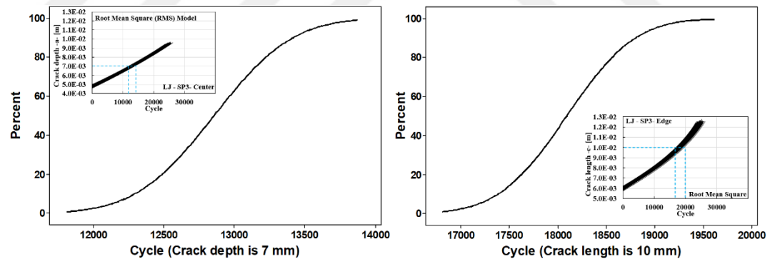
Figure 5.149. CDF for load cycles under constant crack length conditions (LJ specimen, SP3 loading spectrum, Root mean square model)
