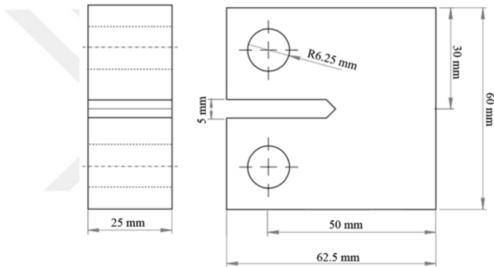
Figure 3.3. Technical drawing of CT specimen
