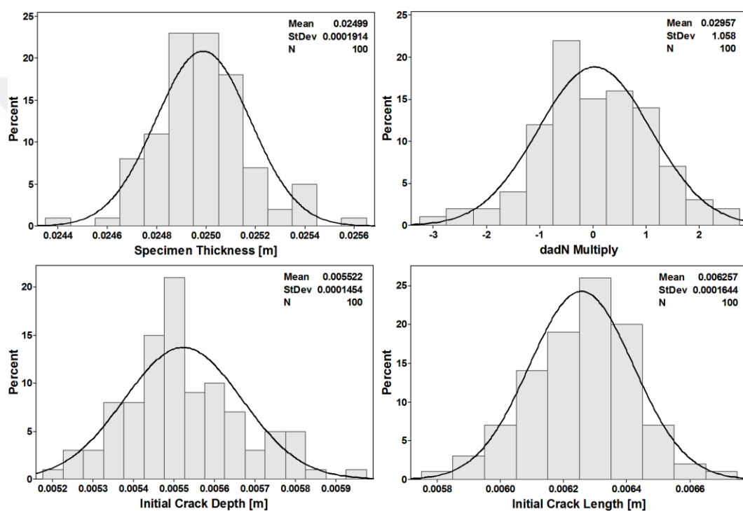
Figure 5.74. Distributions of the inputs used in crack growth life analysis (LJ specimen, SP1 loading spectrum, Wheeler model with Forman)
