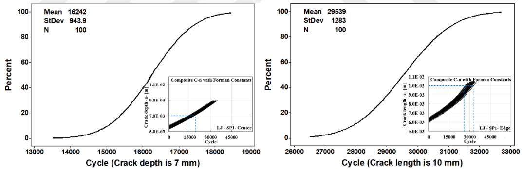
Figure 5.68. CDF for load cycles under constant crack length conditions (LJ specimen, SP1 loading spectrum, Composite C-n with Forman Constants)
