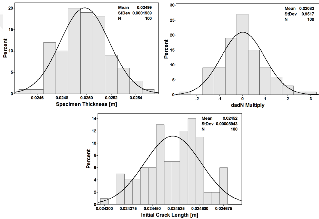
Figure 5.14. Distributions of the inputs used in crack growth life analysis (CT specimen, SP1 loading spectrum, Composite C-n with Walker Constants)
