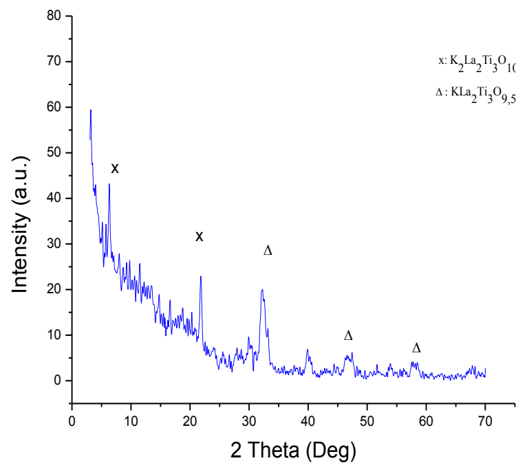
Figure 4.5 XRD pattern of \text{K}_2\text{La}_{1.5}\text{Sm}_{0.5}\text{Ti}_3\text{O}_{10} films on Si substrate
