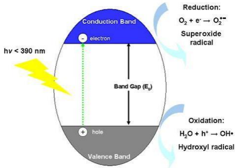
Figure 2.1 A schematic diagram of photocatalysis (Pelaiez et al., 2012).
