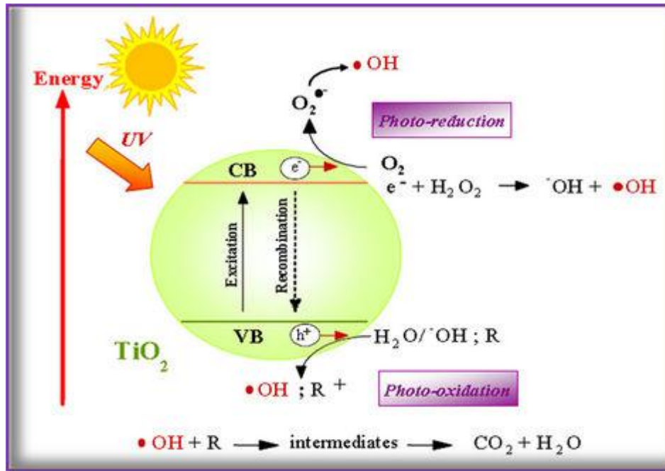
Figure 2.5 Semiconductor \text{TiO}_2 (Giwa et al., 2012).
