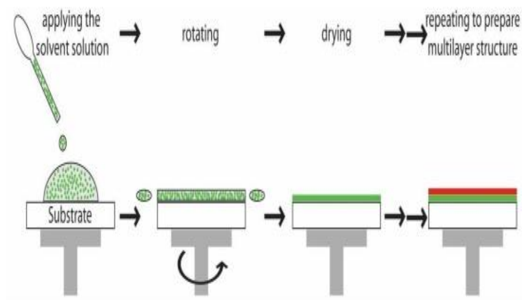
Figure 3.1 Spin coating technique (Anonym, n.d).
