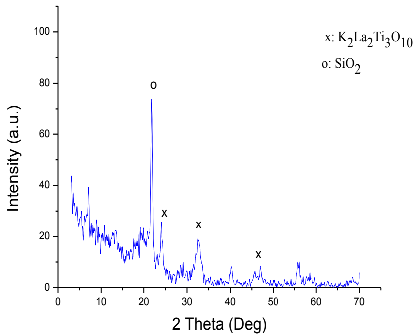
Figure 4.4 XRD pattern of \text{K}_2\text{La}_{1.1}\text{Nd}_{0.9}\text{Ti}_3\text{O}_{10} films on Si substrate
