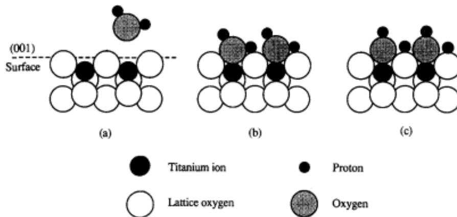
Figure 2.6 Surface hydroxyl groups on \text{TiO}_2 . (a) Hydroxyl-free surface; (b) physical adsorption of water; (c) dissociation of water, giving rise to two distinct OH groups (Boehm and Hermann, 1967).
