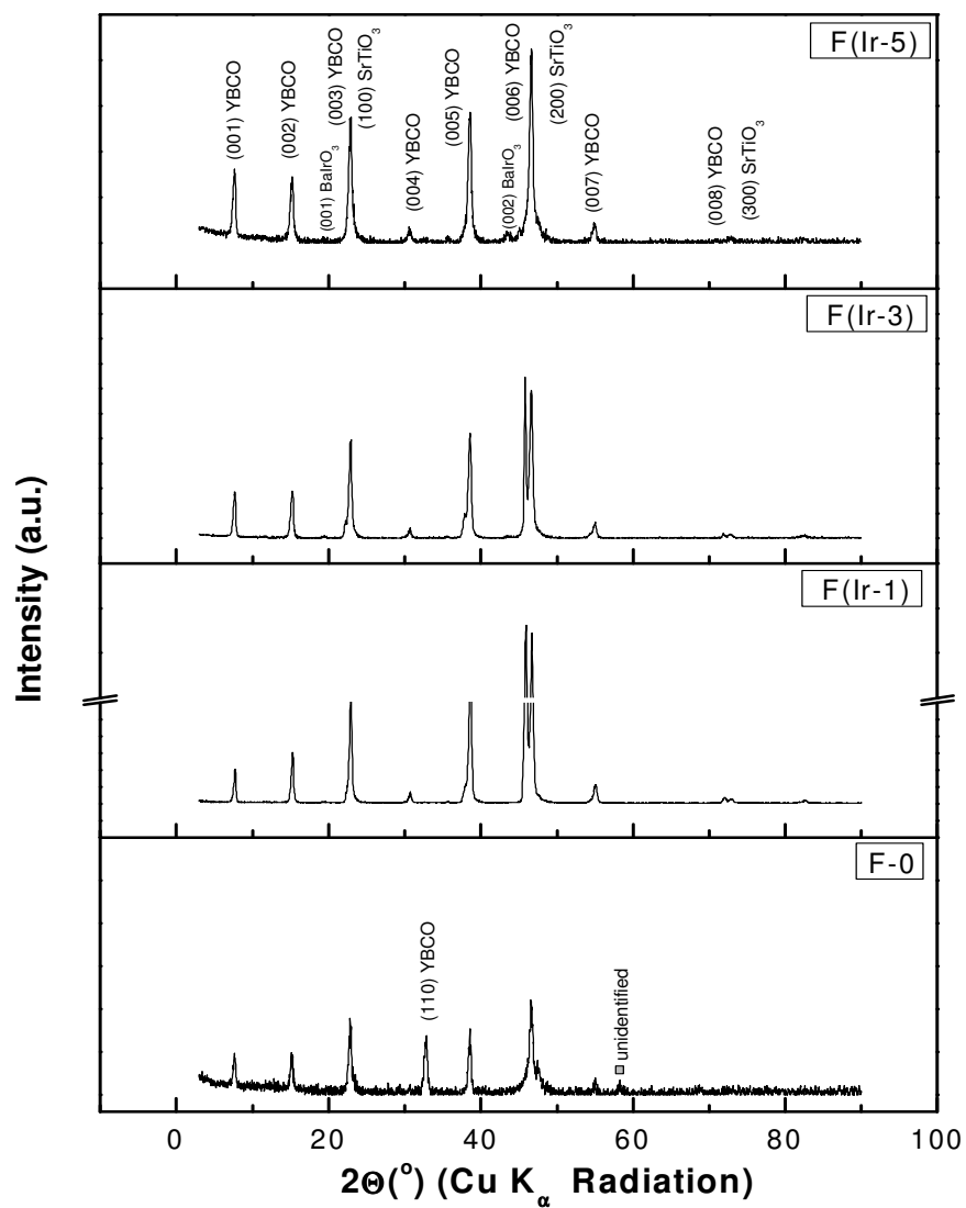
Figure 5.10 X-ray \theta - 2\theta scans of samples including undoped and \text{BaIrO}_3 doped YBCO with a \text{Cu K}\alpha radiation. (YBCO JCPDS card no: 040-0159, \text{SrTiO}_3 JCPDS card no: 035-0734).
