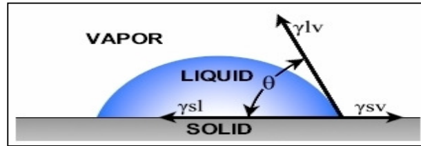
Figure 4.9 The schematic view of contact angle.
