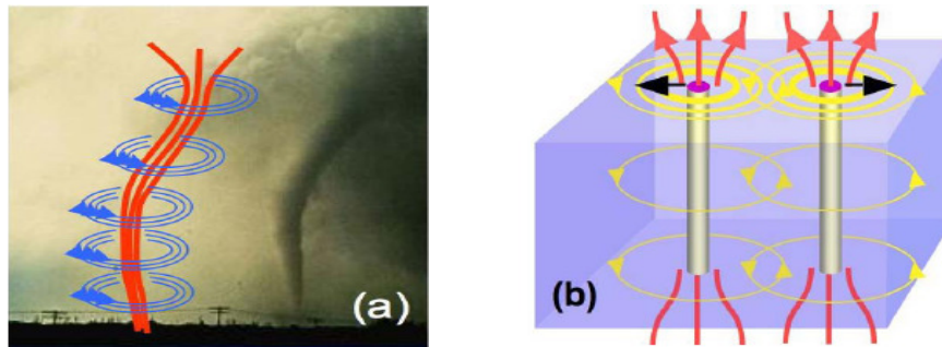
Figure 2.12 (a) A tornado and (b) schematic view of vortex (Sarraf et al., 2006)
