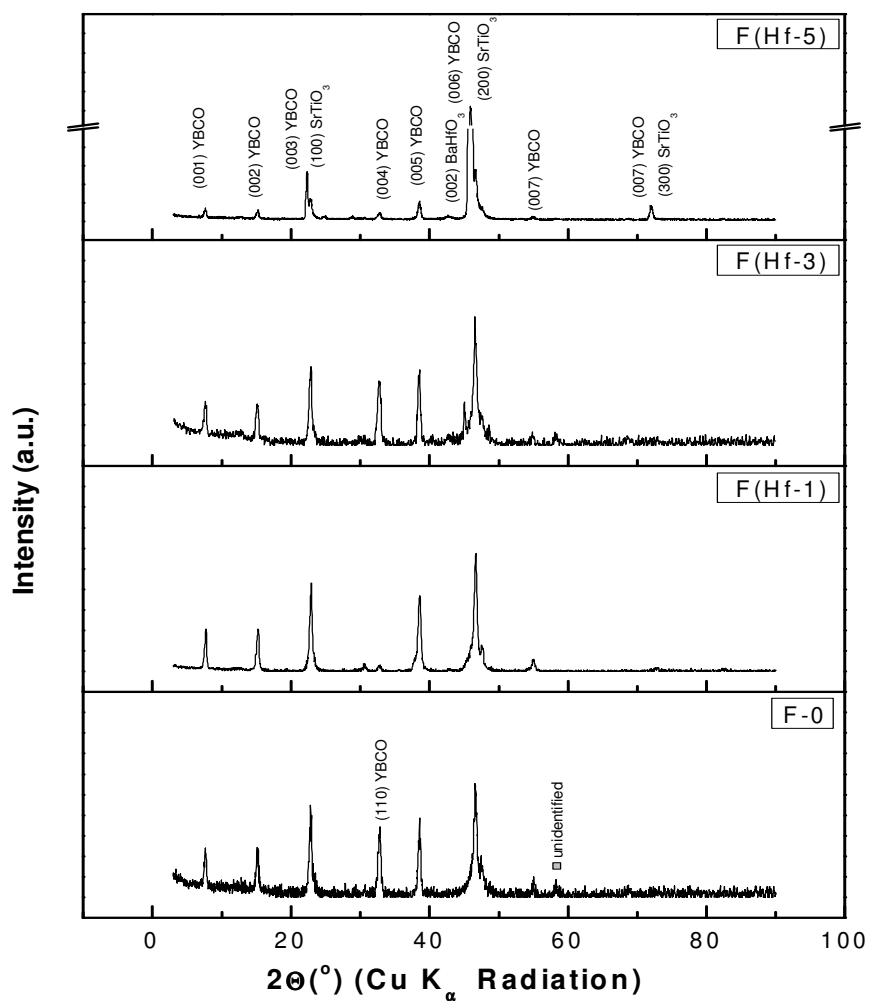
Figure 5.9 X-ray \theta - 2\theta scans of superconducting samples including undoped and \text{BaHfO}_3 doped YBCO with a Cu K_{\alpha} radiation. (YBCO JCPDS card no: 040-0159, \text{SrTiO}_3 JCPDS card no: 035-0734).
