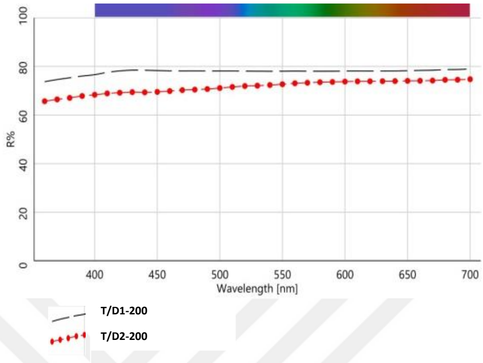
Figure 4.6 %R vs wavelength diagrams for 200 filaments BCF samples
