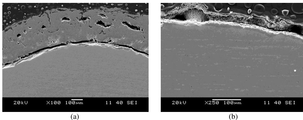
Figure 4.14 Cross-sectional SE micrograph of (a) as-received Nb and (b) 950°C/8h boronized Nb slugs after oxidation at 1000°C for 30 min.
