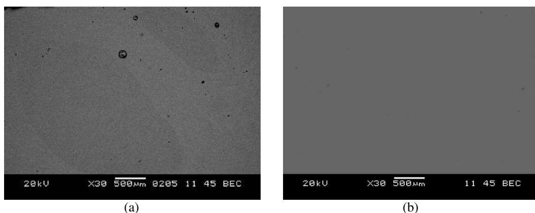
Figure 4.21 BE images of NM (b)-1 and NM (p)-5 alloy samples.
