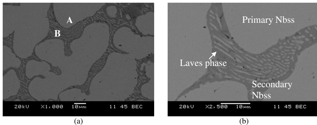
Figure 4.17 Micrographs showing the microstructure of the NC (b)-1 alloy.
