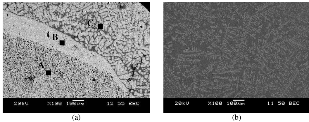
Figure 4.16 Micrographs showing (a) unmelted Nb pieces in NC (b)-3 and (b) microstructure of NC (b)-4 alloy produced by the ‘stepwise’ method.
