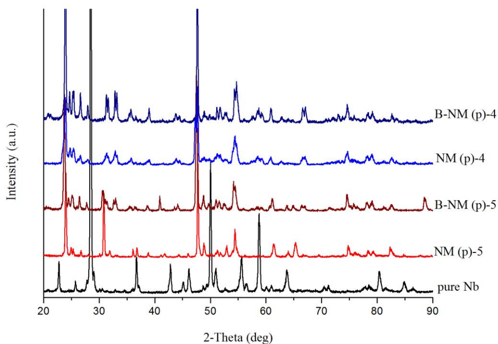
Figure 4.34 XRD analysis of “as-cast” and “boronized” Nb-Mo samples and as-received Nb plate after oxidation at 1000°C for 30 min.
