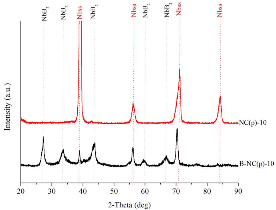
Figure 4.25 XRD diffraction pattern of the unboronized and boronized NC (p)-10 alloy.
