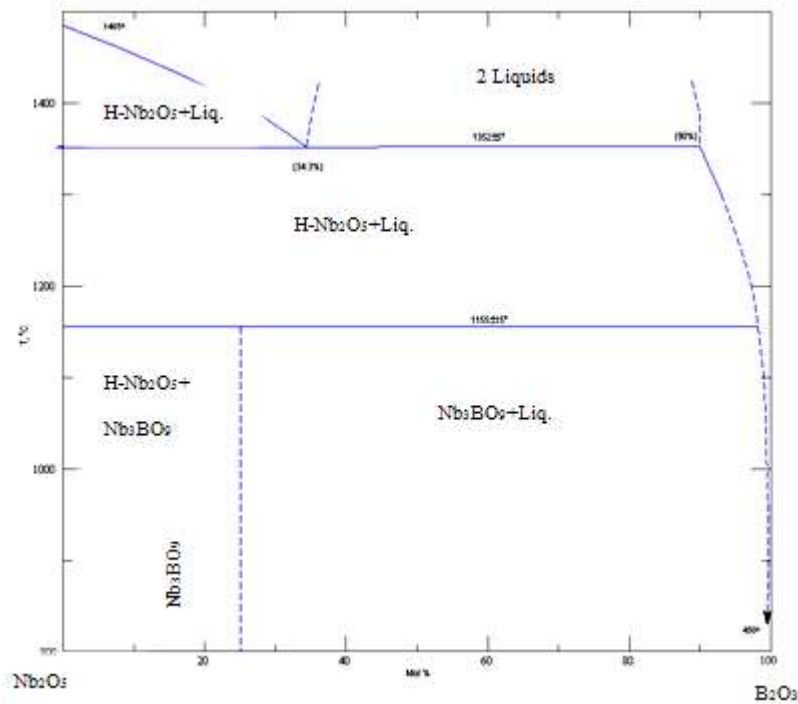
Figure 4.12 Binary \text{Nb}_2\text{O}_5 - \text{B}_2\text{O}_3 oxides phase diagram (Levin, 1966)
