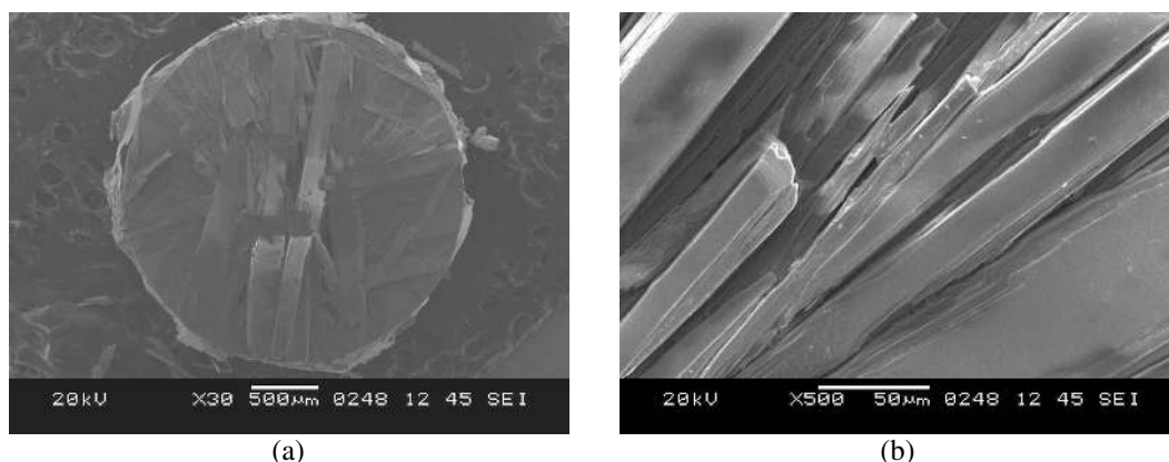
Figure 4.2 (a) a general and (b) high magnification SEM micrograph of pure Mo after oxidation test at 800°C for 30 min.
