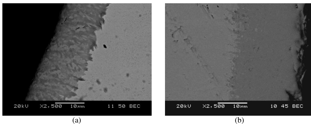
Figure 4.5 SEM/BE cross-sectional micrographs of Mo slugs boronized at 950°C for (a) 4h and (b) 6h.
