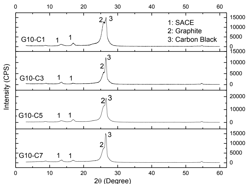
Figure 4.5 XRD patterns of binary graphite and carbon black reinforced CPC films (10 series).
