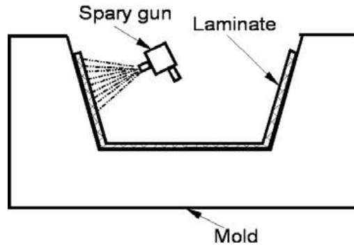
Figure 2.11 Schematic illustration of spray up molding (Mazumdar, 2001).
