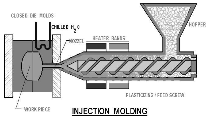
Figure 2.8 Schematic illustration of Injection molding (Western Carolina University, 2013)
