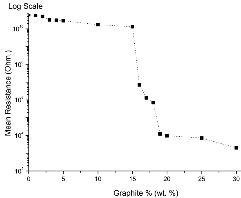
Figure 4.20 Mean resistance versus graphite content.
