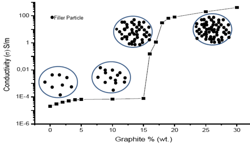
Figure 1.1 Schematic illustration of percolation phenomena.
