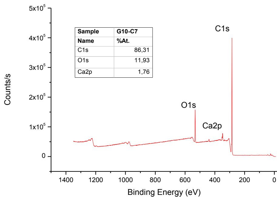
Figure 4.9 XPS result of sample G10-C7
