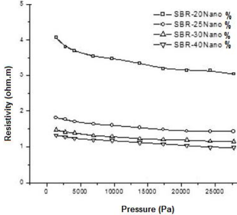
Figure 2.19 Effect of pressure on DC resistivity of SBR-nano composites (Mohanraj et al., 2007).
