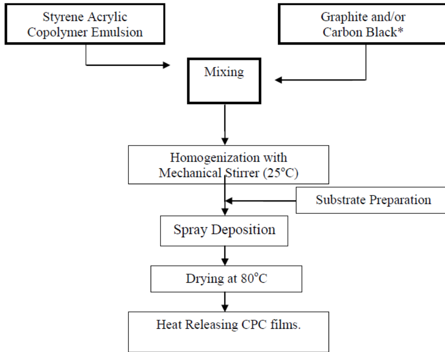
Figure 3.7 Flow chart for the production of heat releasing CPC films.
