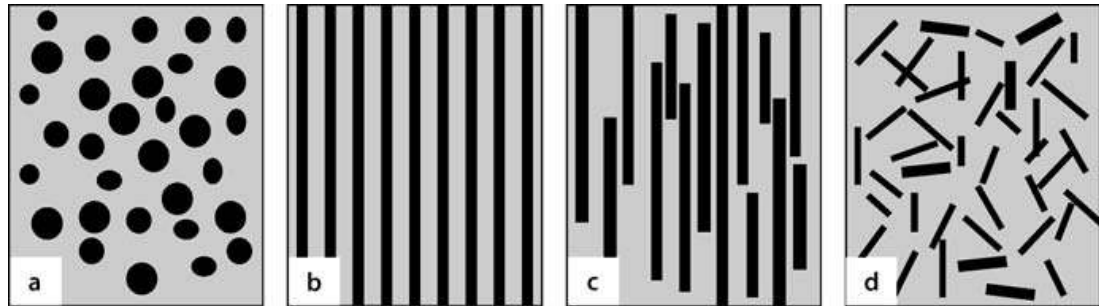
Figure 2.1 Schematic representations of polymer composites: (a) particle reinforcement, (b) fiber reinforcement with continuous and aligned fibers; (c) with discontinuous and aligned fibers; (d) with discontinuous and randomly oriented fibers (Michler, 2008).
