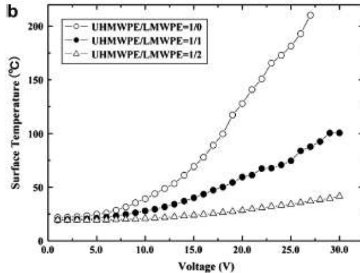
Figure 2.22 An example study for PMC heating elements (Isaji et al 2009).
