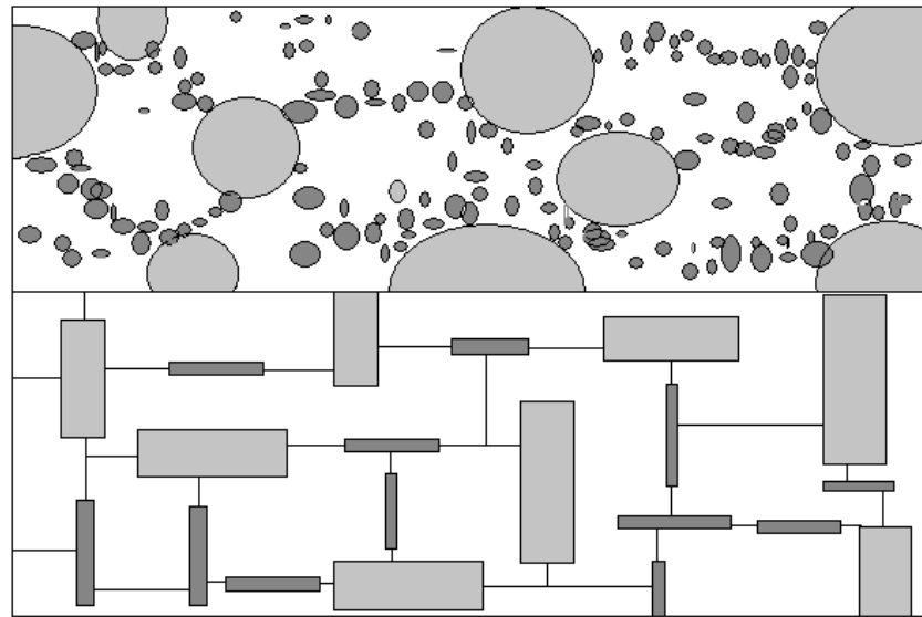
Figure 4.24 Two-dimensional model of the composition based on polymers with a binary filler (graphite + carbon black) (top) and equivalent direct current scheme (bottom). Big circles - graphite particles; small circles - carbon black particles; big rectangles – resistance of graphite particles; small rectangles – resistance of carbon black particles (Aneli et al., 2011).
