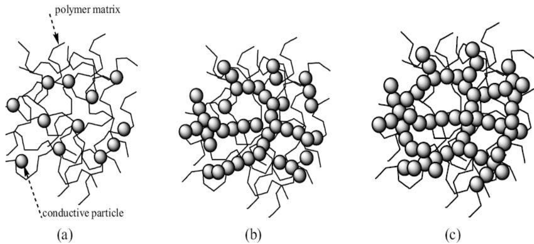
Figure 2.15 Schematic representation of conductive particles dispersed in a polymer matrix at different particle volume fractions: (a) X < X_{th} , (b) X = X_{th} , (c) X > X_{th} (Dai, 2004).
