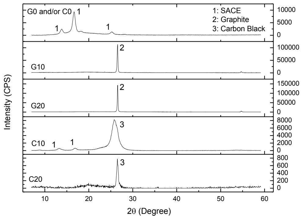
Figure 4.3 XRD patterns of carbon black and graphite reinforced CPC films.
