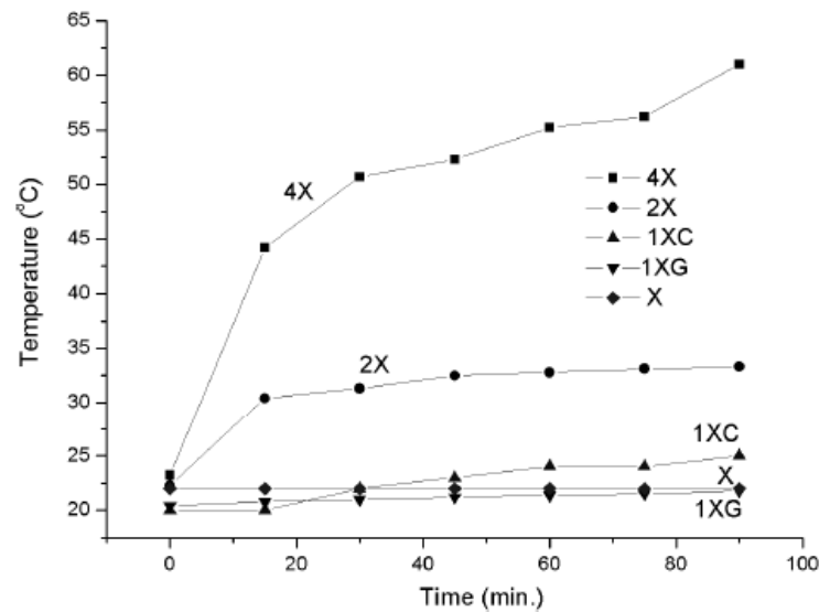
Figure 2.23 An example study for PMC heating elements (Erol, & Celik, 2013).
