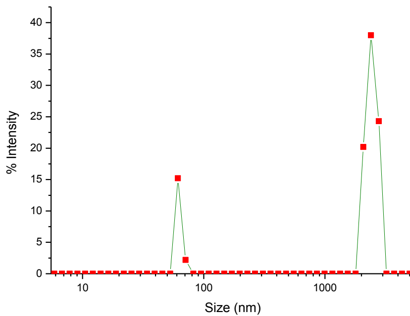
Figure 4.1 Particle size distribution of graphite powders.
