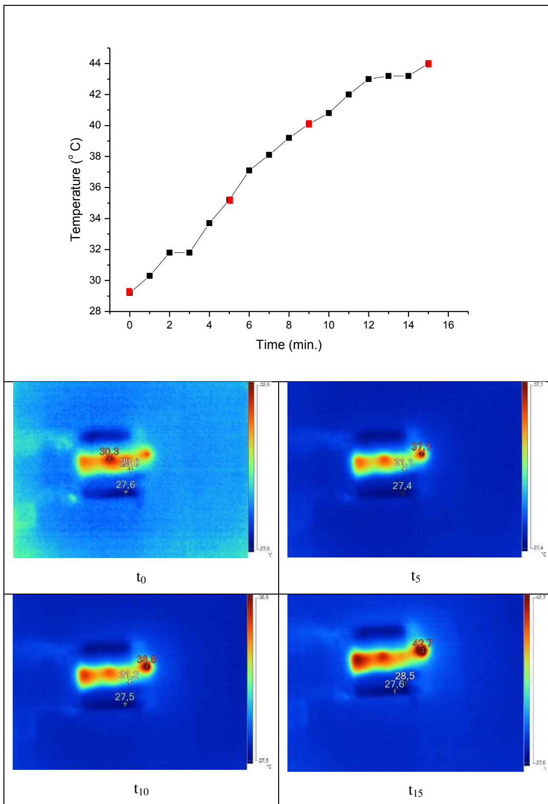
Figure 4.27 Thermal regime and thermal images of the sample G10-C1 (Red squares indicate the time when the images are taken).
