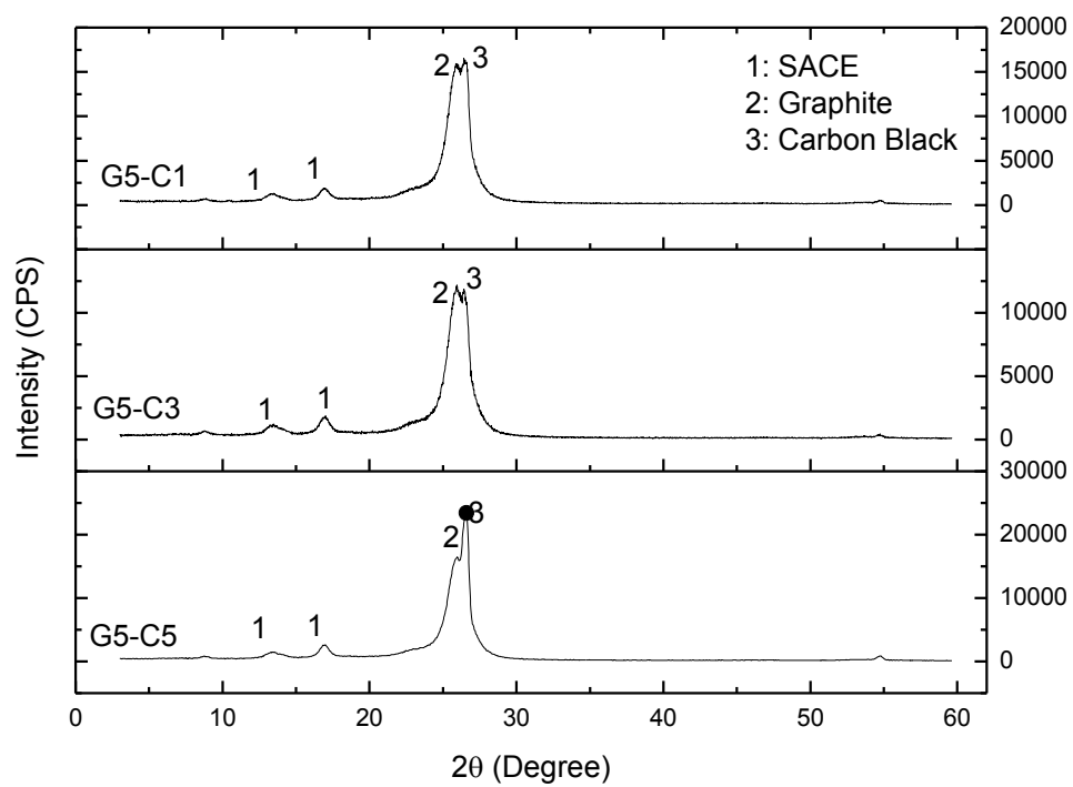
Figure 4.4 XRD patterns of binary graphite and carbon black reinforced CPC films (5 series).
