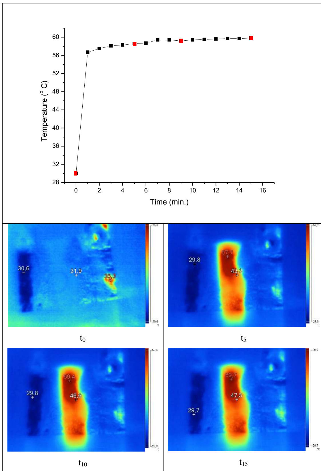
Figure 4.26 Thermal regime and thermal images of the sample C20 (Red squares indicate the time when the images are taken).
