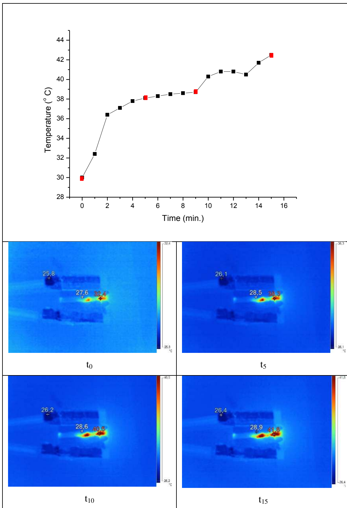
Figure 4.28 Thermal regime and thermal images of the sample G10-C3 (Red squares indicate the time when the images are taken).
