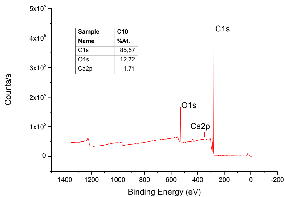
Figure 4.6 XPS result of sample C10
