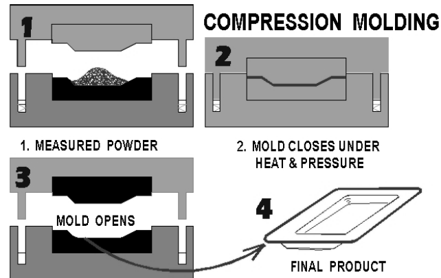
Figure 2.10 Schematic flow of compression molding (Western Carolina University, 2013).
