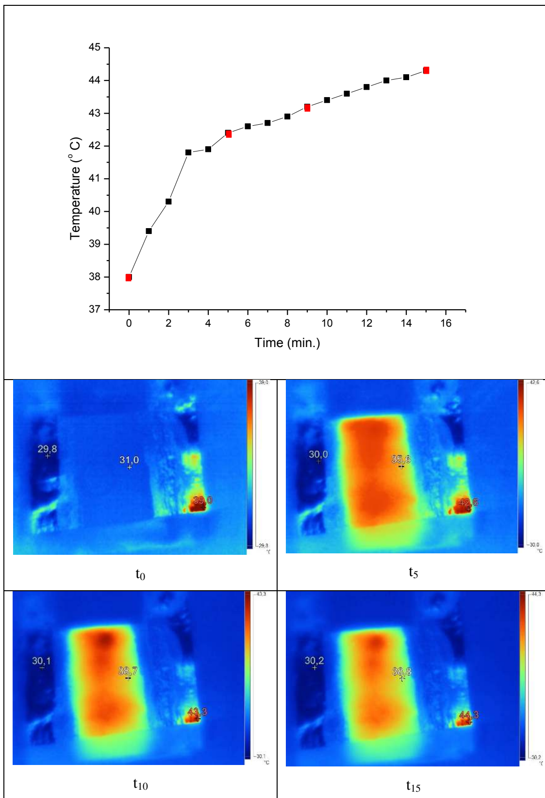
Figure 4.25 Thermal regime and thermal images of the sample G20 (Red squares indicate the time when the images are taken).
