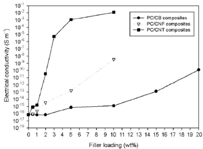
Figure 2.17 Electrical conductivity of the three types of PC composites with various carbon filler loadings (Lee et al. 2008).
