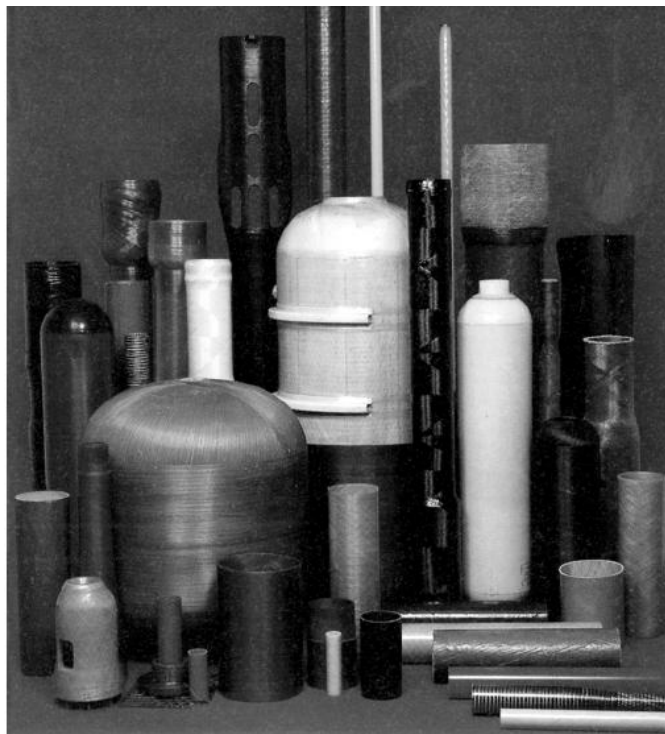
Figure 2.5 Filament wound parts (Mazumdar, 2001).
