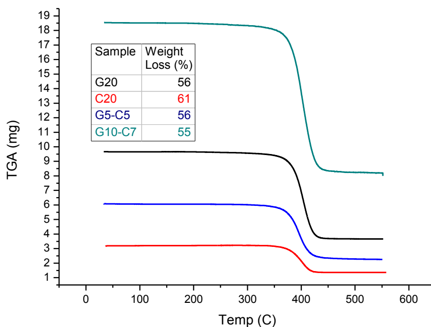
Figure 4.17 Thermogravimetric analysis of the samples
