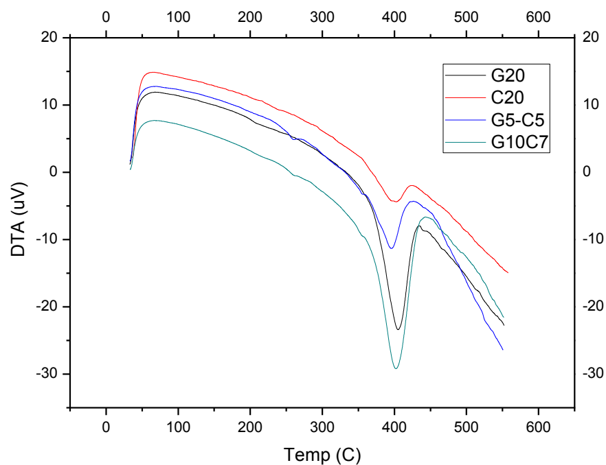
Figure 4.16 Differential thermal analysis of the samples
