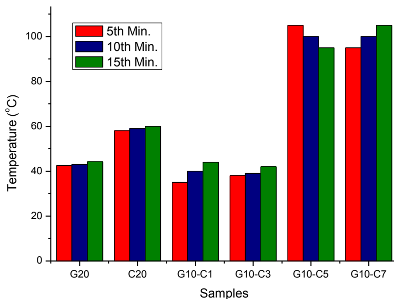
Figure 4.31 Comparative surface temperatures of the samples for different durations.
