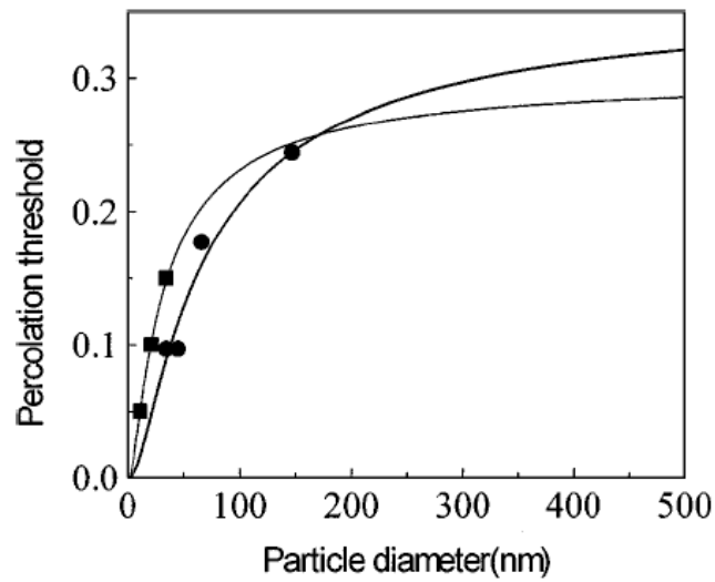
Figure 2.16 Plots of percolation threshold against particle diameter. Solid squares and solid circles are data taken from different studies respectively (Jing et al. 2000).
