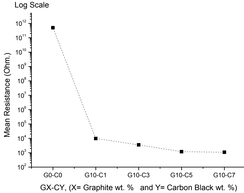
Figure 4.23 Mean resistance values of 10 series samples.
