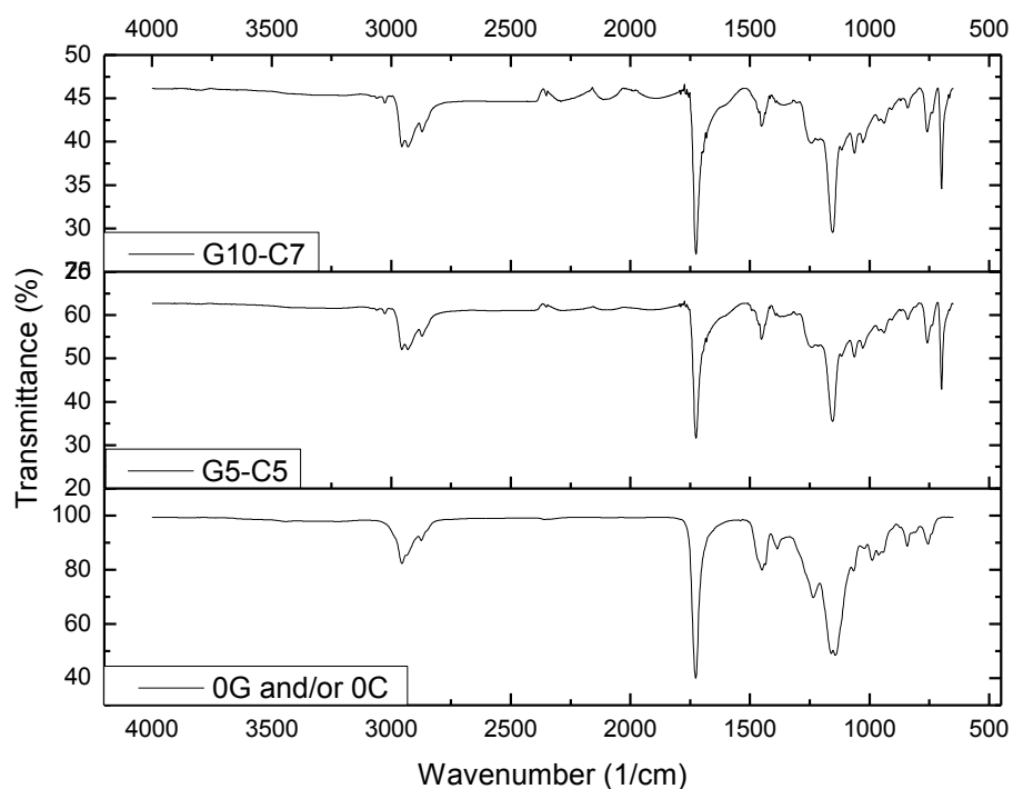
Figure 4.11 FTIR-ATR spectra of binary graphite and carbon black reinforced CPC films
