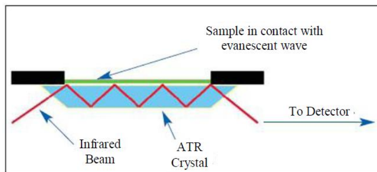
Figure 3.9 Schematic representation of an ATR system (Birlik, 2011)
