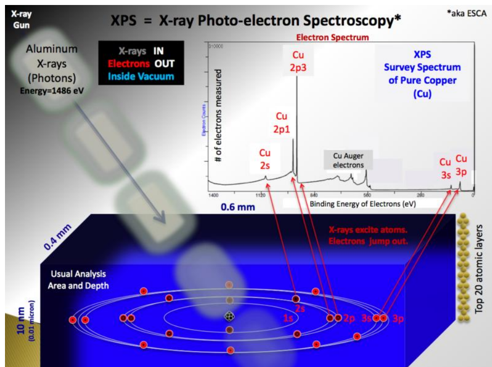
Figure 3.8 Rough schematic of XPS physics (Crist, 2011).
