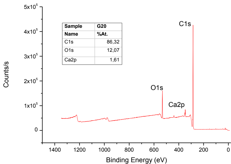
Figure 4.7 XPS result of sample G20
