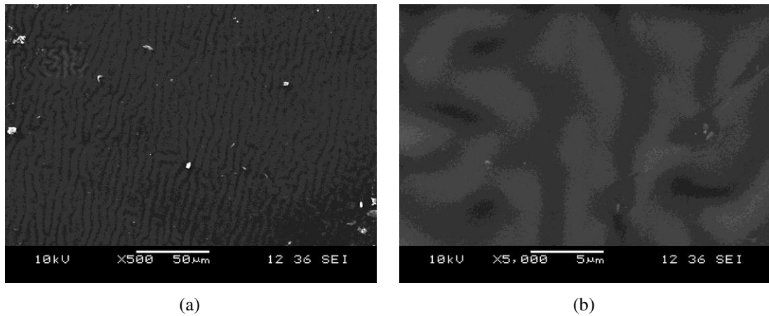
Figure 4.12 SEM micrographs of sample without any filler (a) general and (b) detail view.
