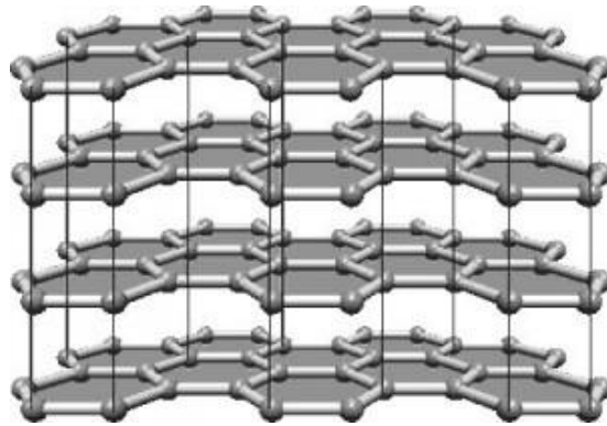
Figure 3.3 Schematic crystalline structure of graphite (Nano Enhanced Wholesale Technologies, 2013).
