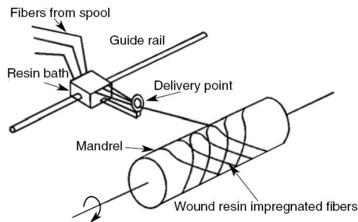
Figure 2.4 Schematic of the filament winding process (Mazumdar, 2001).
