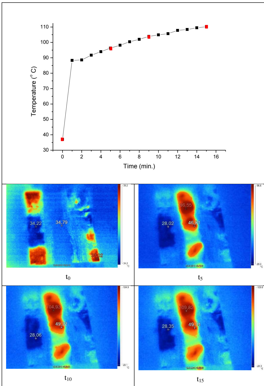
Figure 4.30 Thermal regime and thermal images of the sample G10-C7 (Red squares indicate the time when the images are taken)
