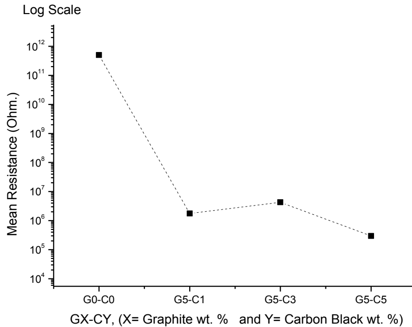
Figure 4.22 Mean resistance values of 5 series samples.
