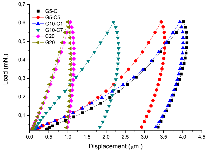
Figure 4.18 Load versus displacement plots of the samples.
