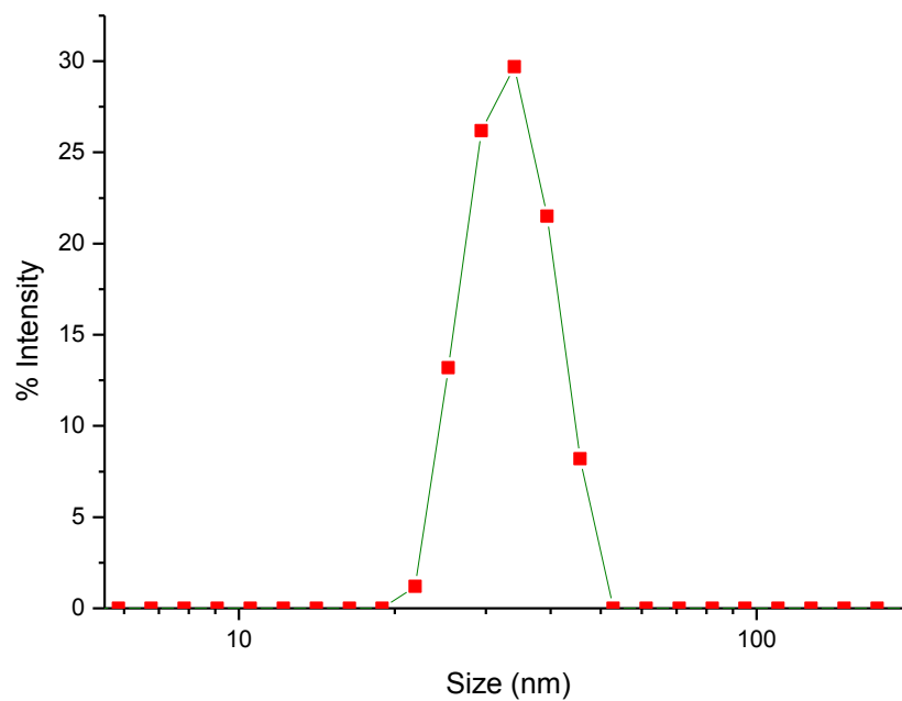
Figure 4.2 Particle size distribution of carbon black powders.
