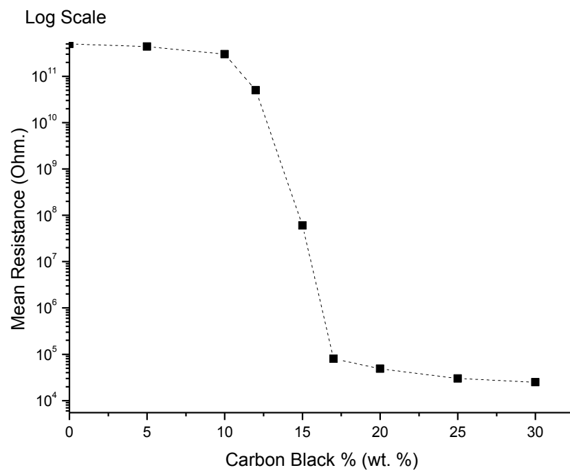
Figure 4.21 Mean resistance versus carbon black content.
