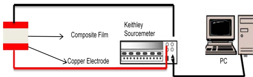
Figure 3.13 A schematic representation of electrical measurements setup.
