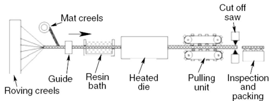
Figure 2.6 Illustration of a pultrusion process (Mazumdar, 2001).
