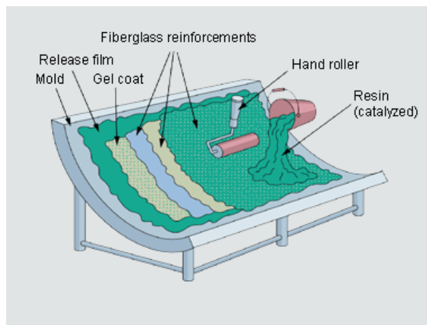
Figure 2.2 Schematic illustration of layup process (Wacker Chemie, 2013).
