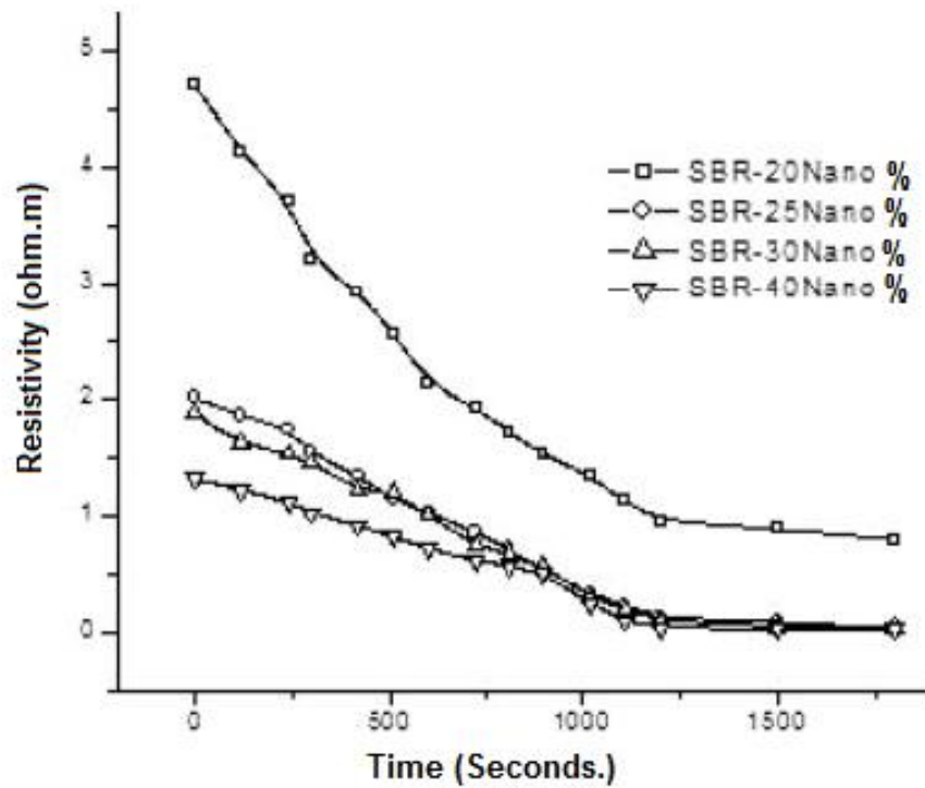
Figure 2.20 Effect of constant compressive stress on DC resistivity of SBR-nano composites (Mohanraj et al 2007).
