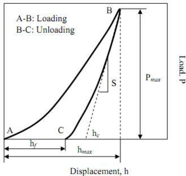
Figure 3.11 A schematic representation of load versus displacement during nanoindentation (Oliver & Pharr, 1992).
