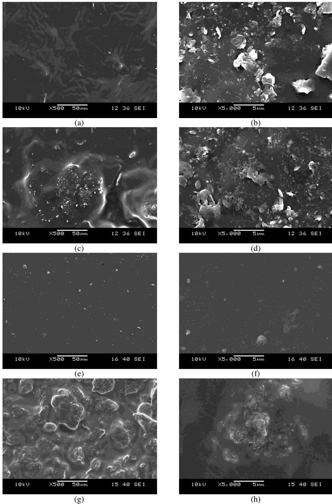
Figure 4.13 SEM micrographs of samples G10, G20, C10 and C20 (a, c, e and g are general b, d, f and h are detail views).
