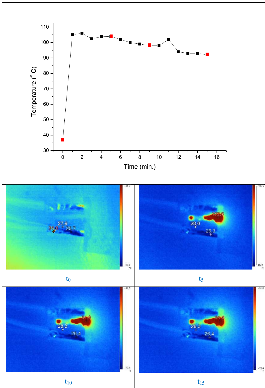
Figure 4.29 Thermal regime and thermal images of the sample G10-C5 (Red squares indicate the time when the images are taken).
