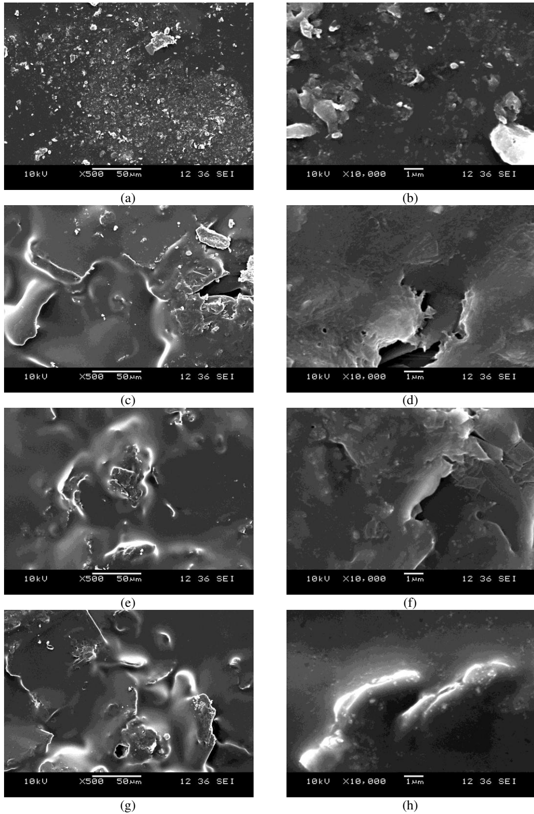
Figure 4.15 SEM micrographs of samples -C1, G10-C3, G10-C5, G10-C7 (a, c, e and g are general b, d, f and h are detail views).
