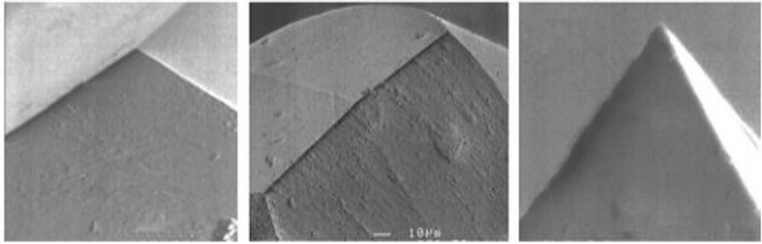
Figure 3.10 SEM images of the tips of (a) Berkovich, (b) Knoop, and (c) cube-corner indenters used for nanoindentation testing. The tip radius of a typical diamond pyramidal indenter is in the order of 100 nm (Fischer-Cripps, 2009).
