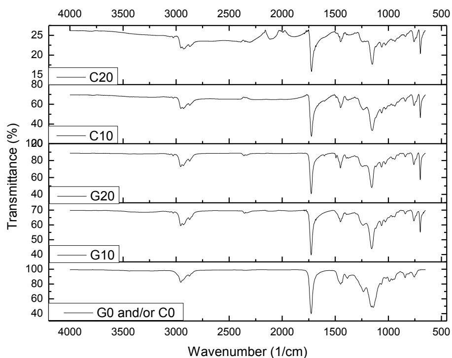
Figure 4.10 FTIR-ATR spectra of carbon black and graphite reinforced CPC films.
