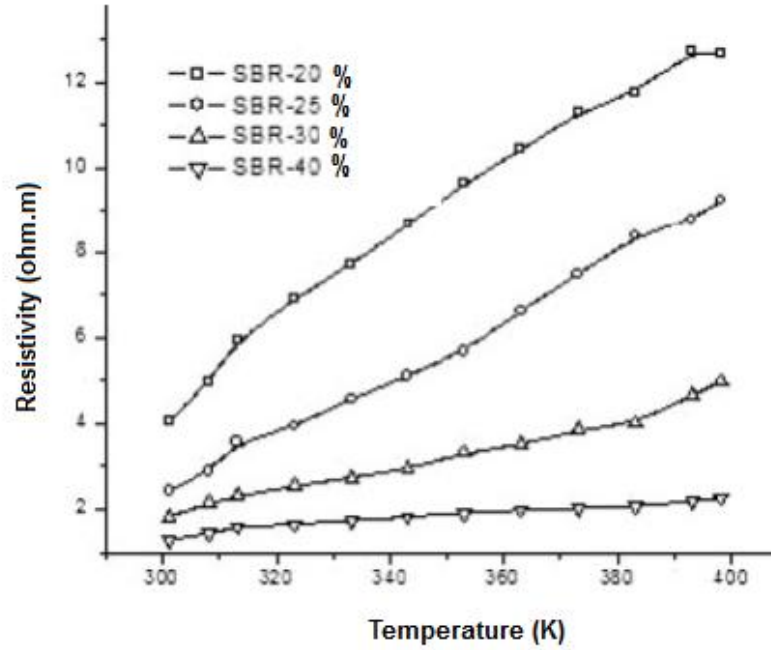
Figure 2.18 Effect of temperature on DC resistivity of SBR-nano composites (Mohanraj et al., 2007).
