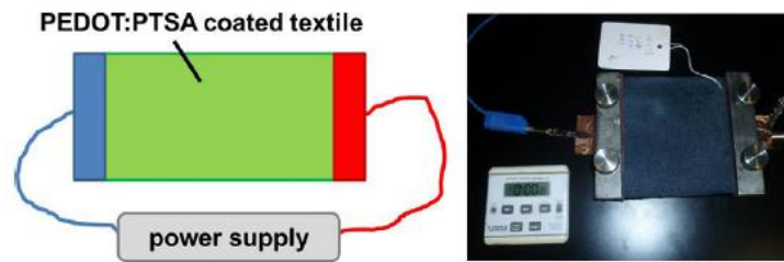
Fig. 7. New strategy: parallel contacting using longish copper panels.
