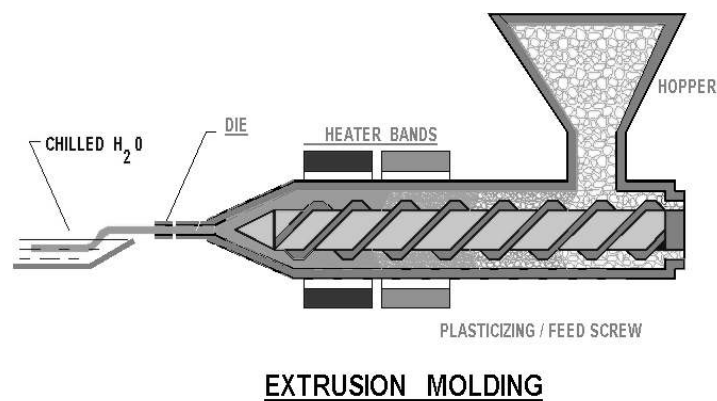
Figure 2.9 Schematic illustration of extrusion molding (Western Carolina University, 2013)
