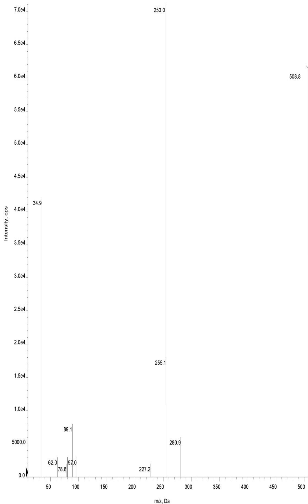
Figure 4.19 Mass spectrum of 2-linolein-1(3)-acetylleucine-rac-glycerol
