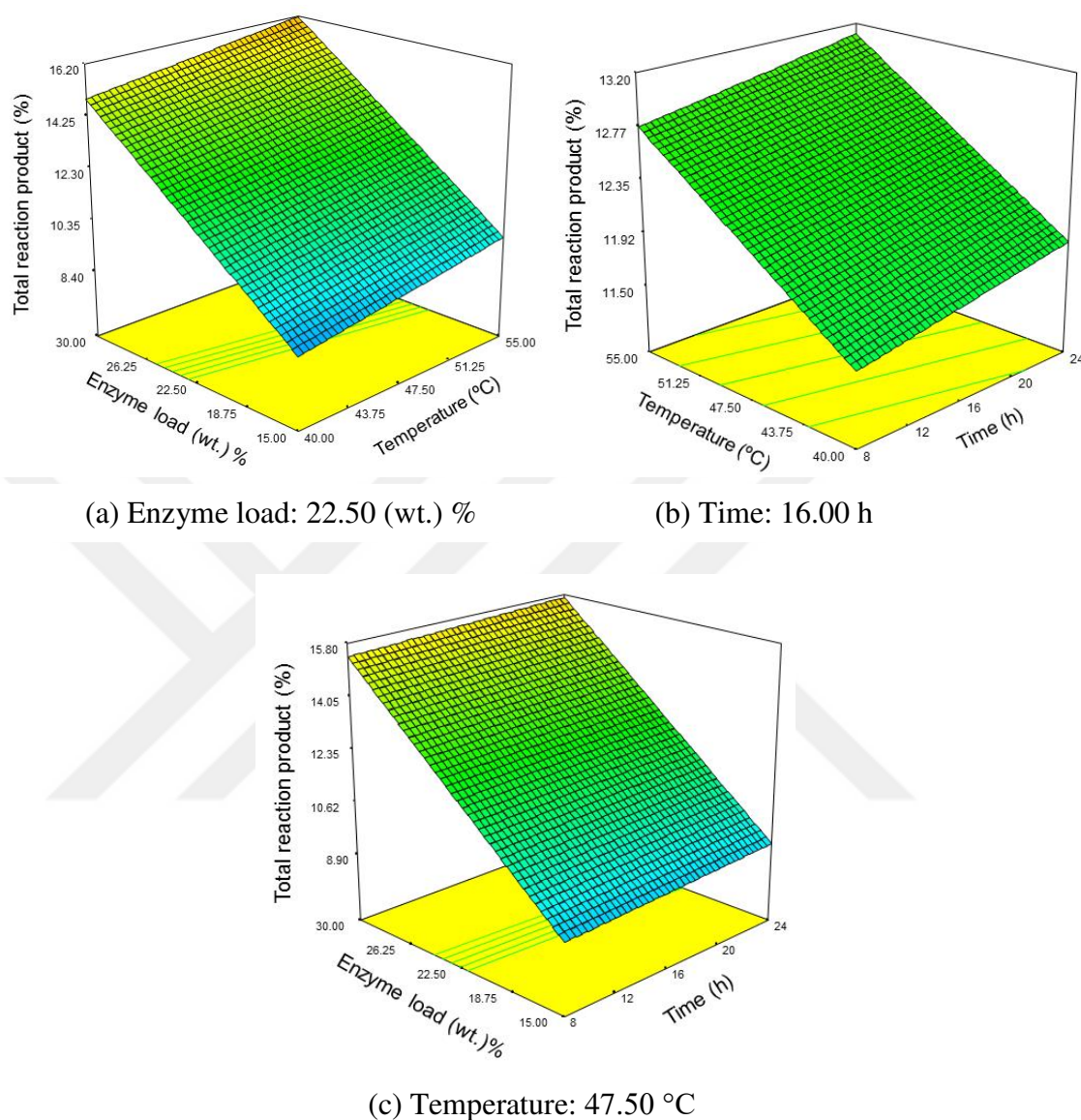
Figure 4.28 Response surface plots for the total reaction product after the reaction of 2-MAG and N -acetyl-L-valine. Total reaction product contains 2-acyl-(1)3-acetylvaline-rac-glycerol ve 2-acyl-1,3-di-acetylvaline-rac-glycerol (A) enzyme load-temperature, (B) temperature-time, (C) enzyme load (wt%)-time.
