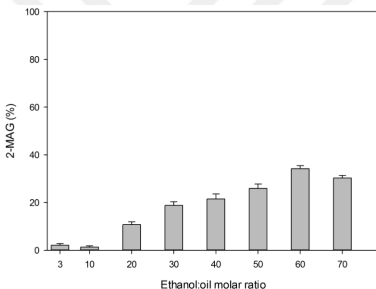
Figure 4.9 The effect of ethanol:oil molar ratio on the ethanolysis of refined olive pomace oil carried out using lipase from C. antarctica . The reaction conditions were enzyme load 15 (wt%), temperature 50°C, time 6 h
