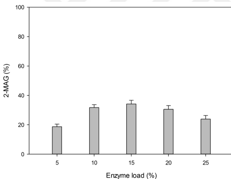
Figure 4.12 The effect of enzyme load on the ethanolsynthesis of refined olive pomace oil with lipase from C. antarctica . The reaction conditions were temperature 50°C, ethanol:oil molar ratio 60:1, time 6 h
