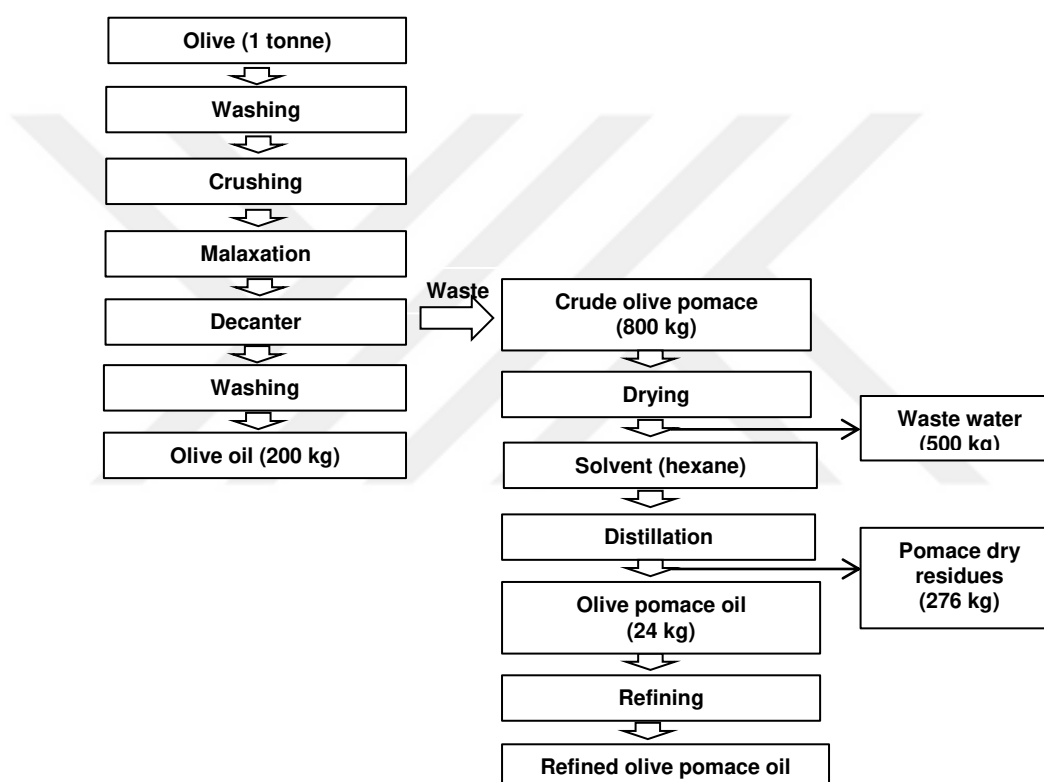
Figure 2.7 Flowchart of olive oil and refined olive pomace oil production
