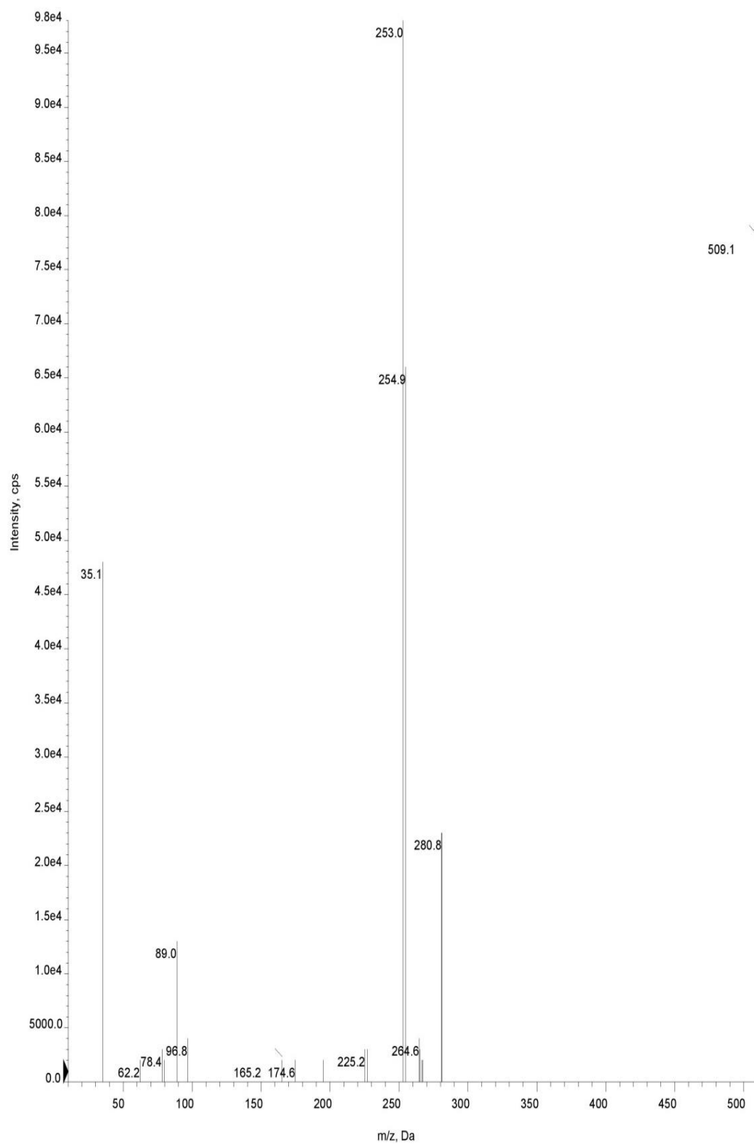
Figure 4.20 Mass spectrum of 2-olein-(1)3-acetylleucine-rac-glycerol
