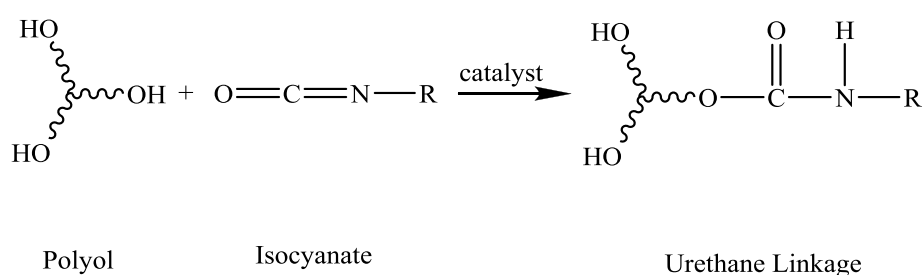
Figure 1.7 Gelling reaction
