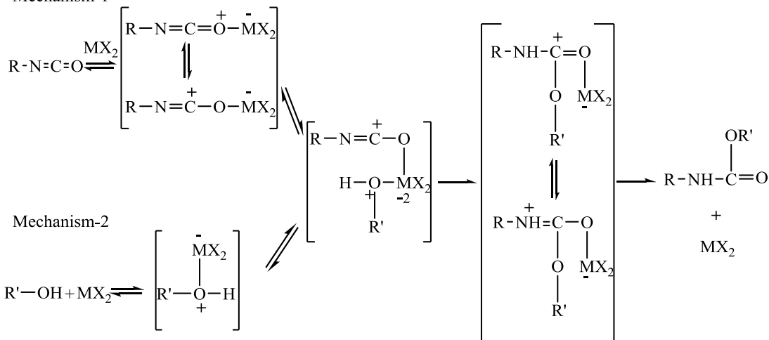
Figure 1.21 Activation mechanism of an organometallic catalyst on the gelling reaction
