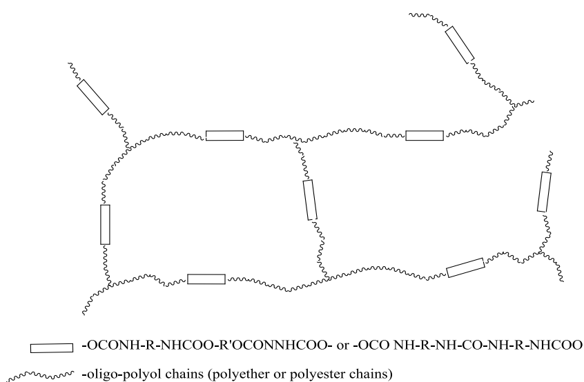
A) Hypothetical crosslinked structure of a flexible polyurethane foam
