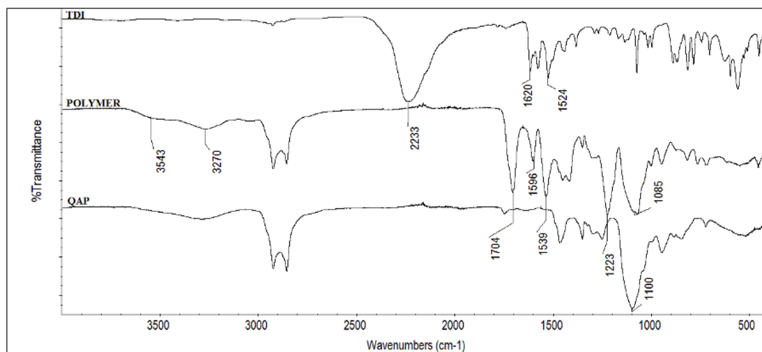
Figure 2. 4 FTIR spectra of the polymer obtained by the reaction between TDI and QAP
