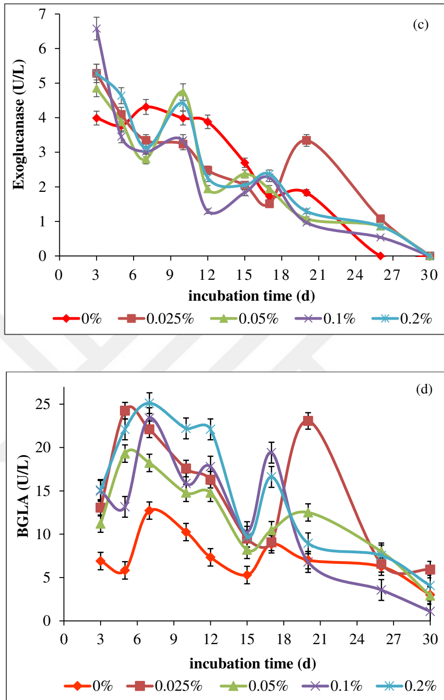
Figure 3.15 Variations of hydrolytic enzymes activities (CMCase (a), xylanase (b), exoglucanase (c), BGLA (d)) on SSF cultures using peach wastes depending on Tween 80 concentrations (% v/v). The values are the mean \pm SD for experiments of three separate experiments (continued)
