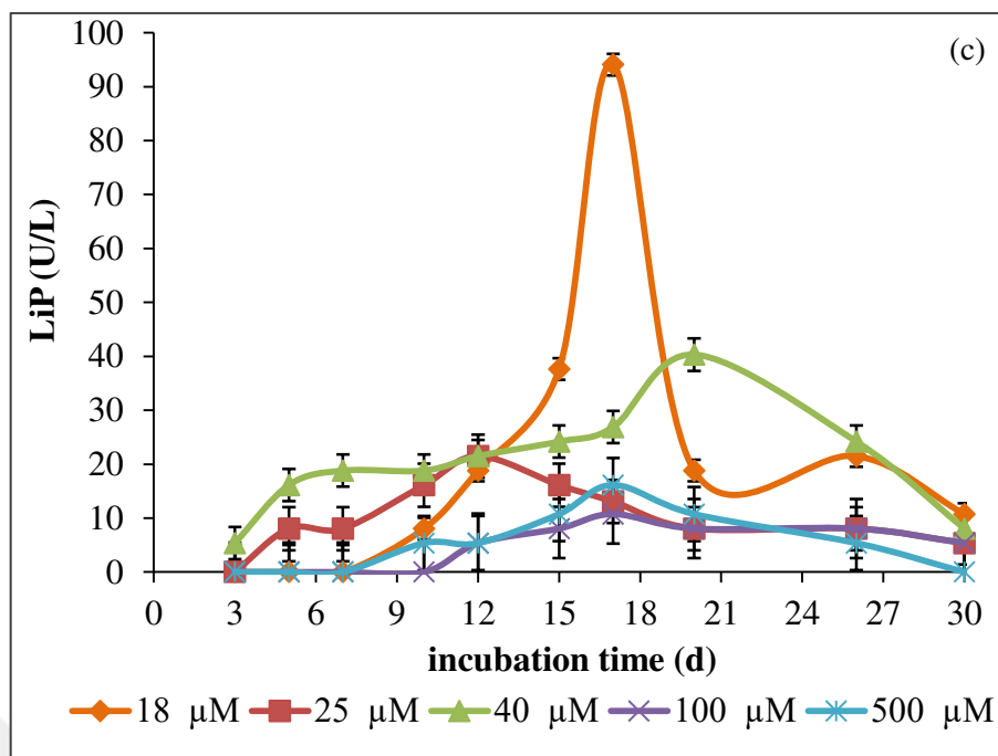
Figure 3.9 The influence of iron concentrations on ligninolytic enzymes activities (Lac (a), MnP (b), LiP (c)) on SSF cultures using peach wastes throughout incubation time. The values are the mean \pm SD for experiments of three separate experiments (continued)
