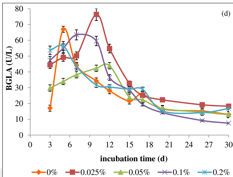
Figure 3.16 Variations of hydrolytic enzymes activities (CMCase (a), xylanase (b), exoglucanase (c), BGLA (d)) on SSF cultures using cherry wastes depending on Tween 80 concentrations (% , v/v). The values are the mean \pm SD for experiments of three separate experiments (continued)
