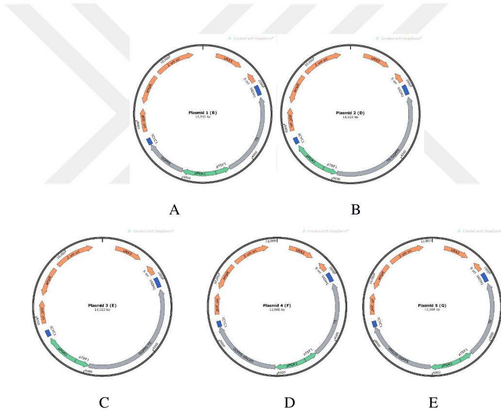
Figure 2.4. Episomal plasmids
