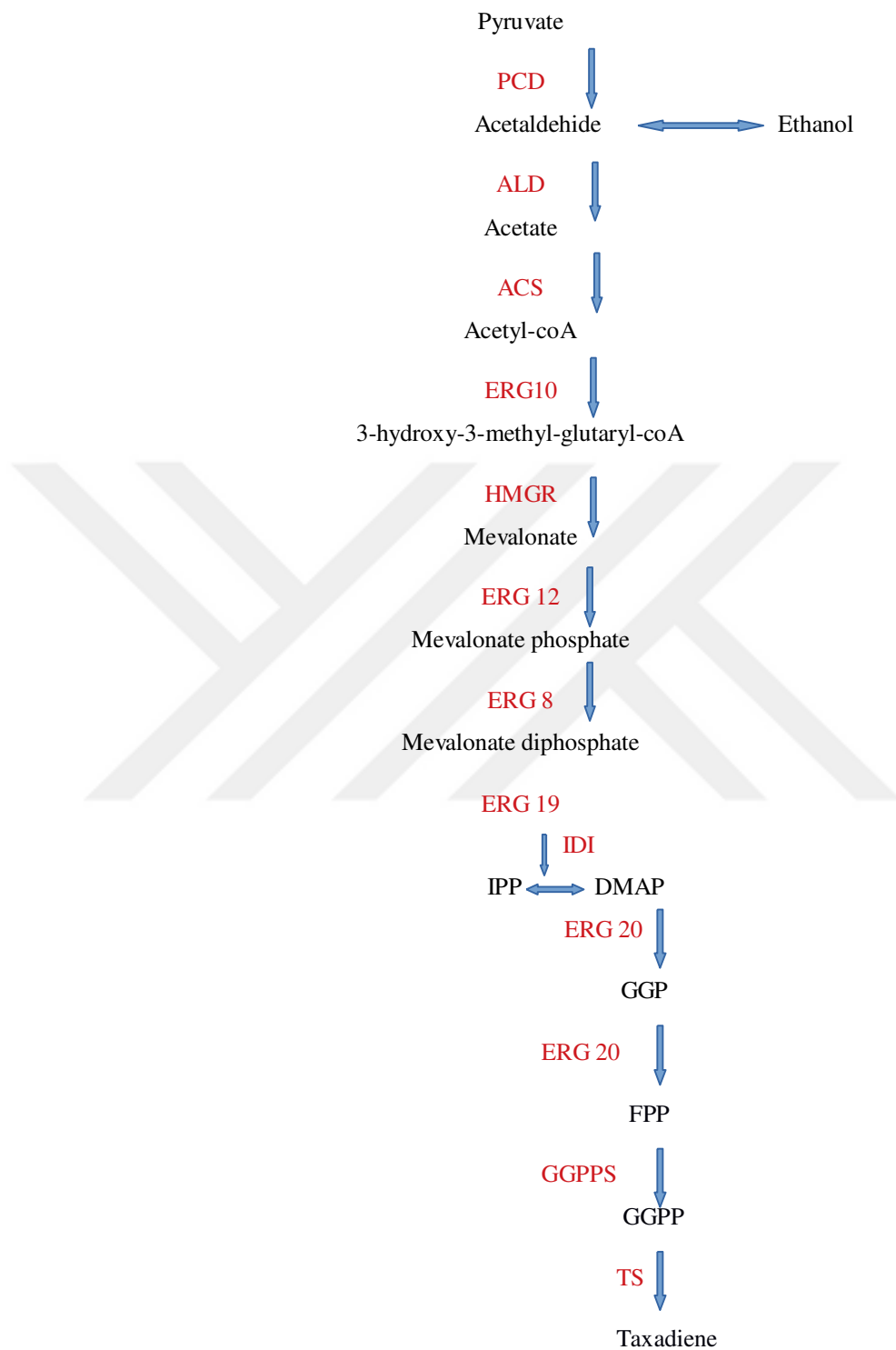
Figure 1.5. Mevalonate pathway in yeast and relationship with taxadiene synthesis.
