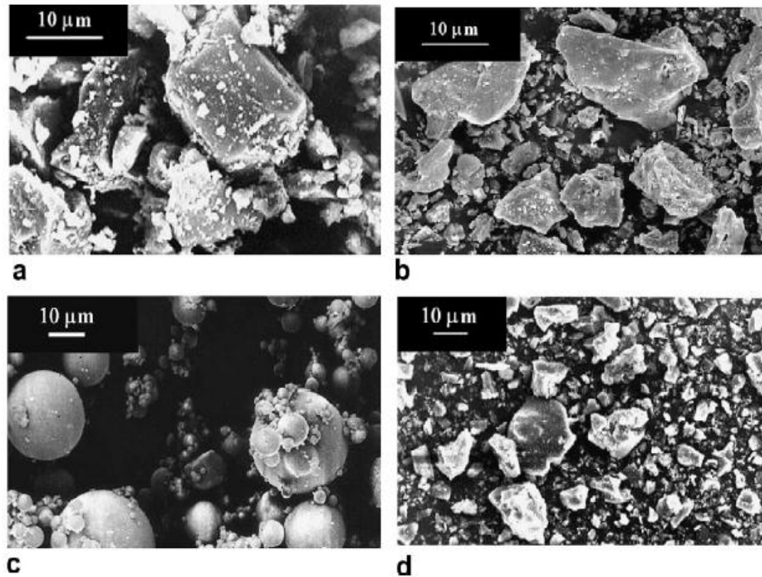
Figure 2.18 Scanning electron microscopy (SEM) of materials: (a) Portland cement type I (OPC); (b) original fly ash (OFA); (c) ground palm oil fuel ash (GPOA); and (d) ground rice husk-bark ash (GRBA).[54]
