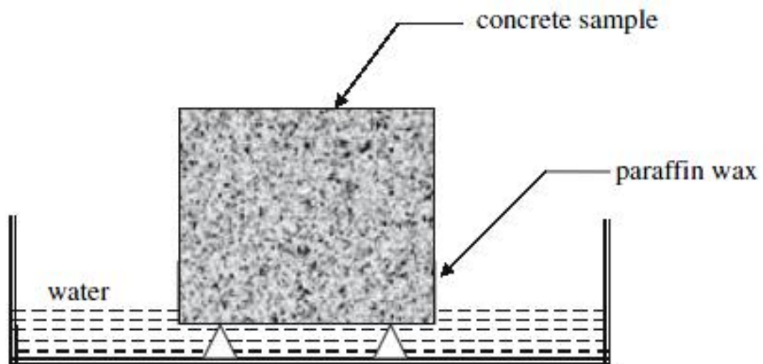
Figure 3.12 Measurement of concrete sorptivity
