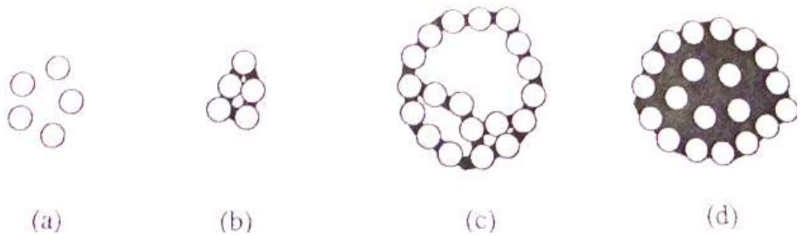
Figure 2.10 Mechanism of ball nuclei formation (water content below optimum state) [40]
