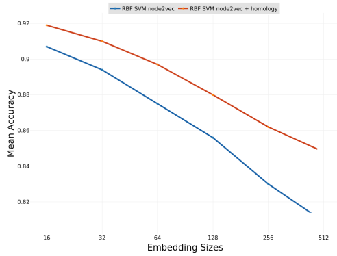
(b) Accuracy plot of RBF kernel
