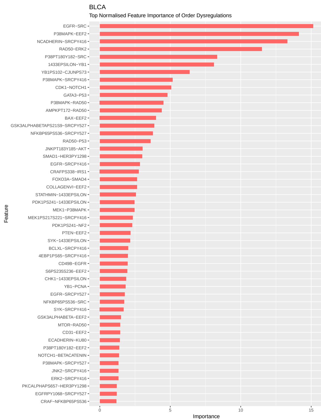
Figure B.3: Variable importance of significant pairwise ranking embeddings for bladder urothelial carcinoma
