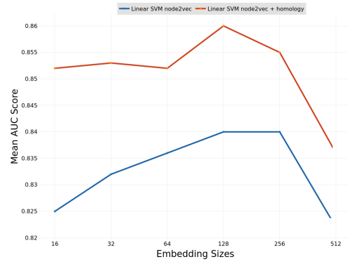
(a) AUC plot of linear kernel
