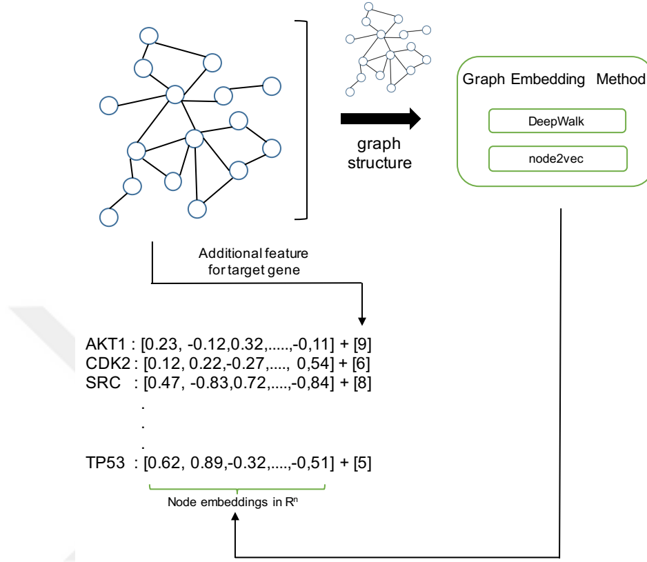
Figure 2.1: Schematic describing how the feature vectors are created based on node embeddings. Input is the PPI network and the output is a latent low-dimensional representation of nodes in the network. The node2vec and DeepWalk algorithms are used to generate the embeddings based on the topological features of the graph. Additional features about the genes can be concatenated to the node embedding vectors. In this case, homology feature is added.
