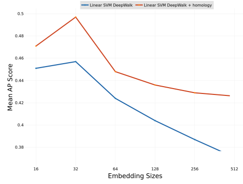
(a) Linear kernel
