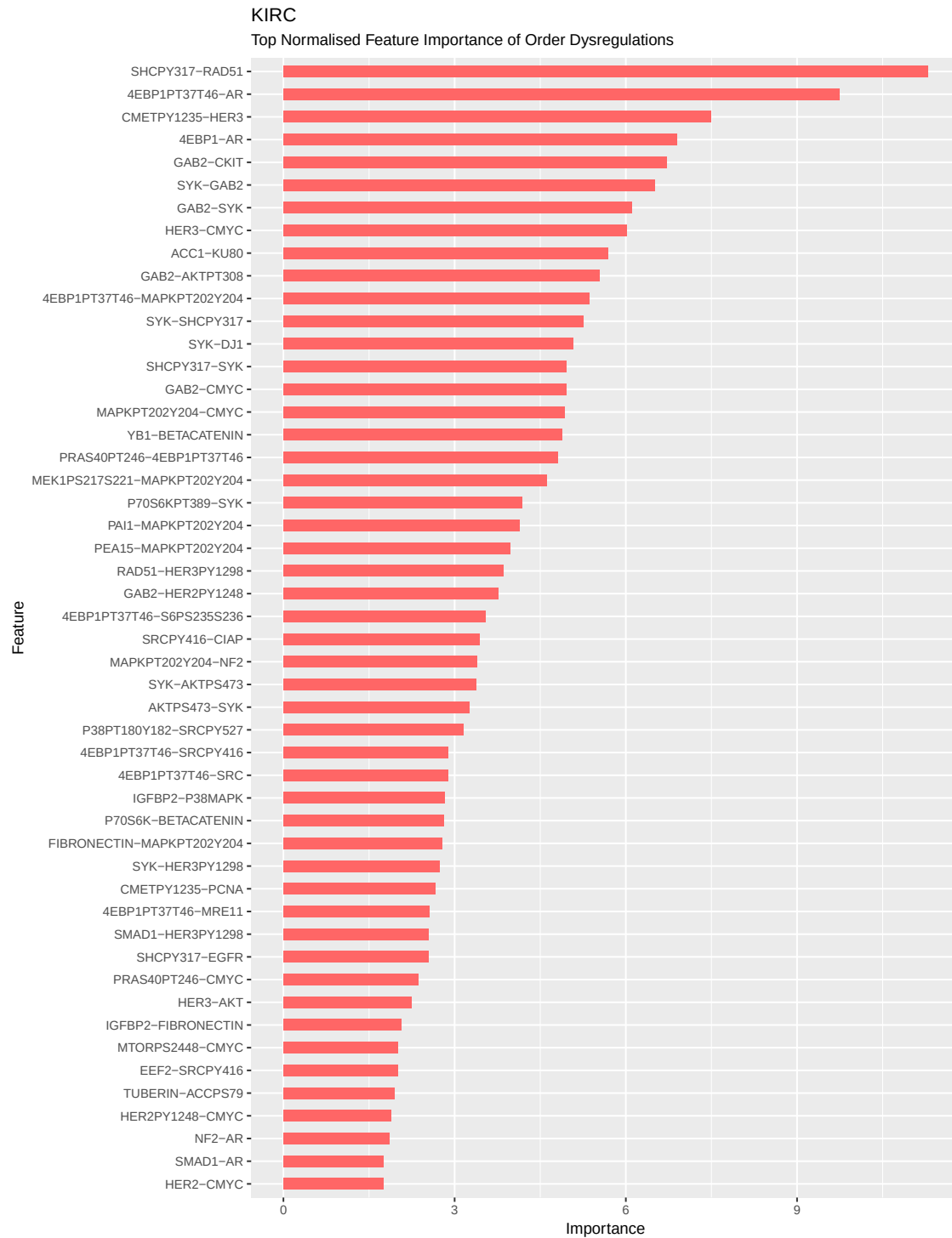
Figure B.1: Variable importance of significant pairwise ranking embeddings for kidney renal clear cell carcinoma
