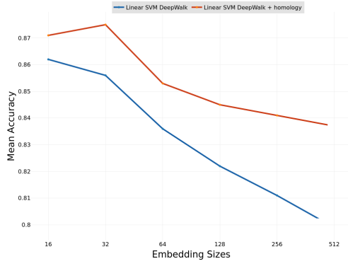
(a) Linear kernel
