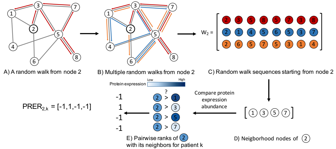
Figure 3.1: The pipeline of the pairwise rank representation which is based on random walks. By generating random walks on the graph, the neighborhood of node 2 is obtained. Then the pairwise comparison of the neighborhood proteins in terms of their protein expression quantities is used to form a representation of the protein.
