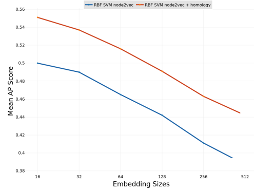
(b) Average precision plot of RBF kernel
