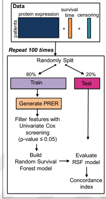
Figure 3.3: General pipeline for survival prediction. The step that involves generating PRER is skipped when the experiment is run with the alternative method of individual expression values.
