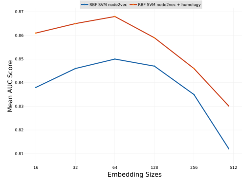
(b) AUC plot of RBF kernel
