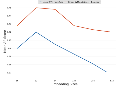
(a) Average precision plot of linear kernel
