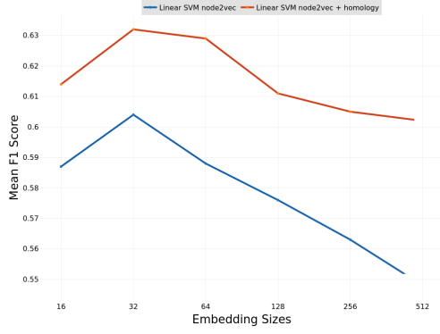
(a) F1 plot of linear kernel
