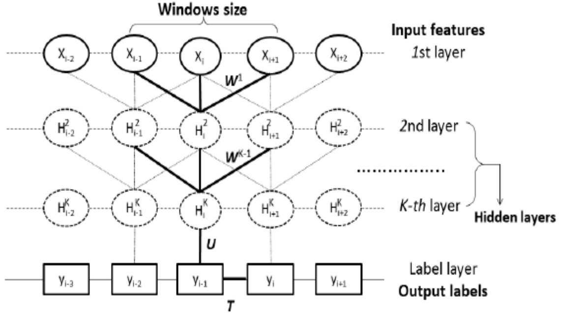
Figure 3.6.2.1 Design of Deep CNF [65], where i is the position index and X_i the associated input features, while H^k is for the k -th hidden layer and Y_i is for the output label. All the layers from the first to the top layer constitute a DCNN with parameter W^k \{k = 1, 2, \dots, K\} . The top layer and the label layer constitute a CRF with U and T as a model parameters. U determines association between output of the top layer and the label layer and T is used for adjacent label correlation.
