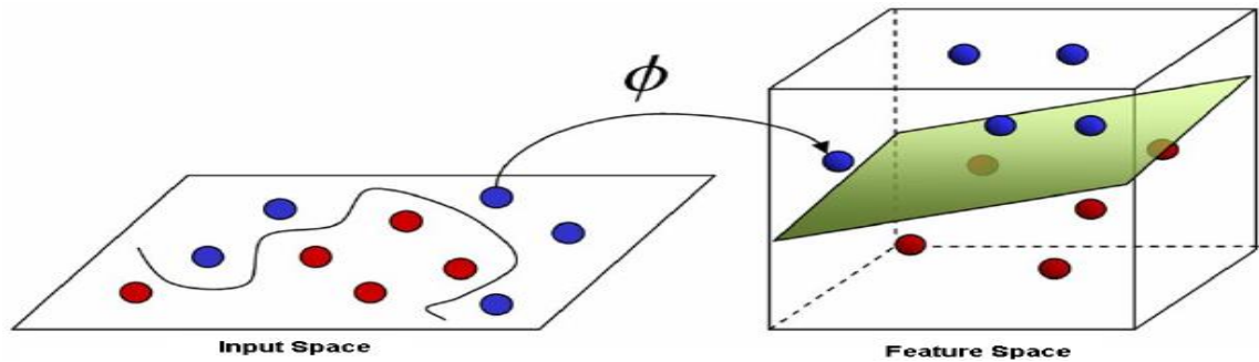
Figure 3.4.2.1 The non-linear SVM [51]
