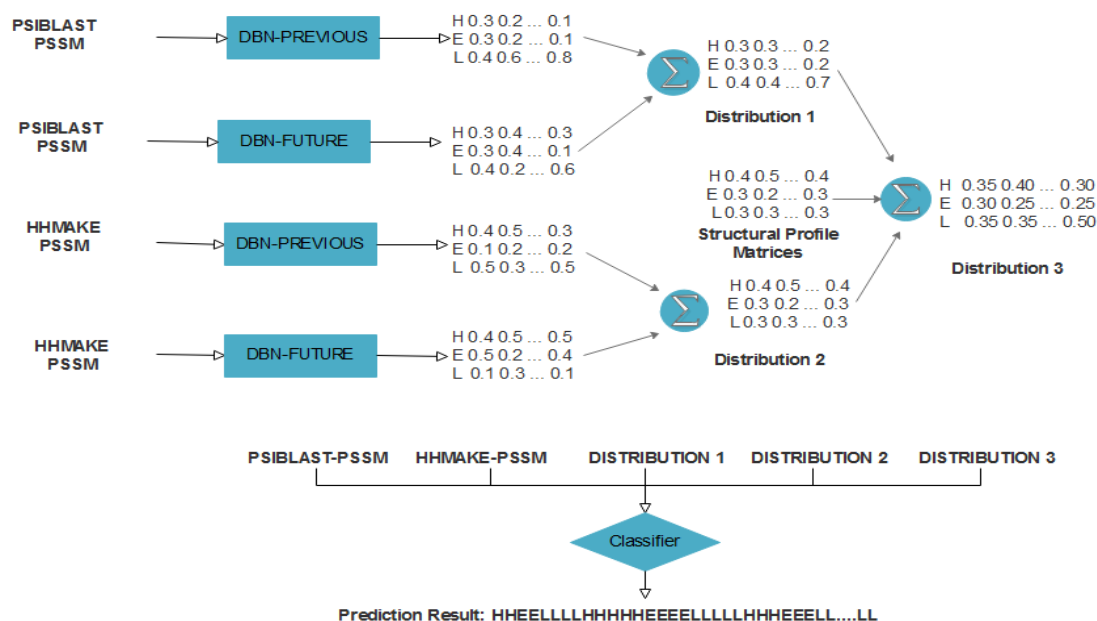
Figure 3.3.1 The two-stage hybrid model for estimating the 3-state secondary structure using dynamic Bayesian networks and a support vector machine
