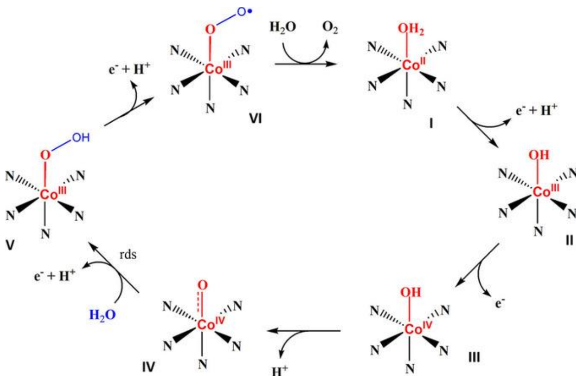
Fig 1. 5 Schematic diagram illustrating OER reaction on \text{Co}^{2+} . [Reprinted with permission from ref [58] (Alsaç et. al., Chem. Eur. J, 2018, 24(19), 4856-4863) WILEY-VCH verlag GmbH & Co. KGaA, Weinheim].
