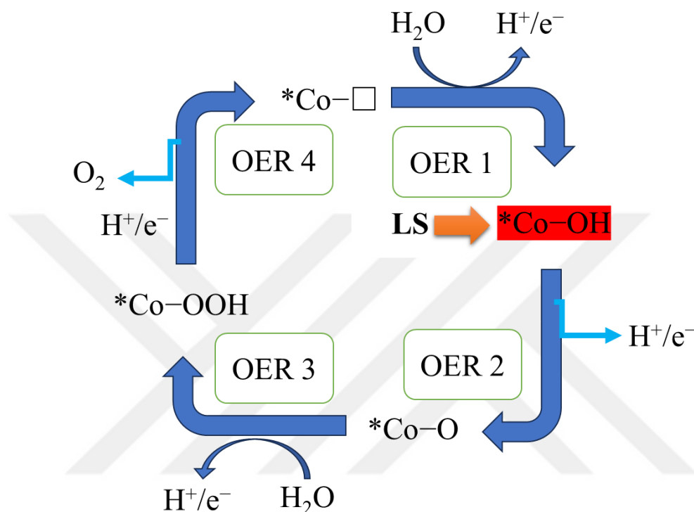
Fig 1. 9 Scheme illustrating the importance of spin crossover effect for Cobalt-based catalyst during a water splitting reaction.
