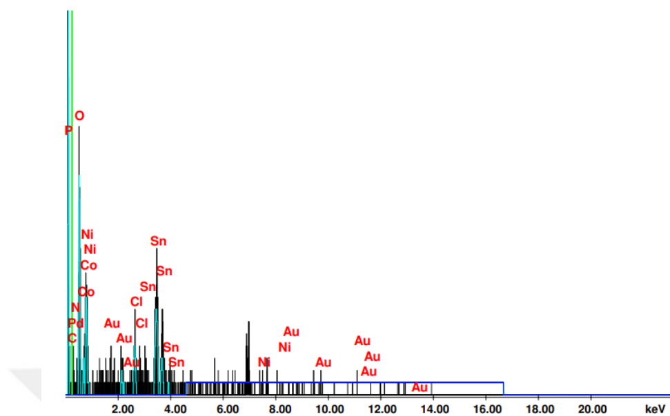
Fig 3. 6 EDAX analysis, the elemental profile of FTO/[Co-Ni].
