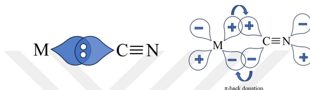
Fig 1. 4 Schematic diagram illustrating \sigma donation and \pi back donation.
