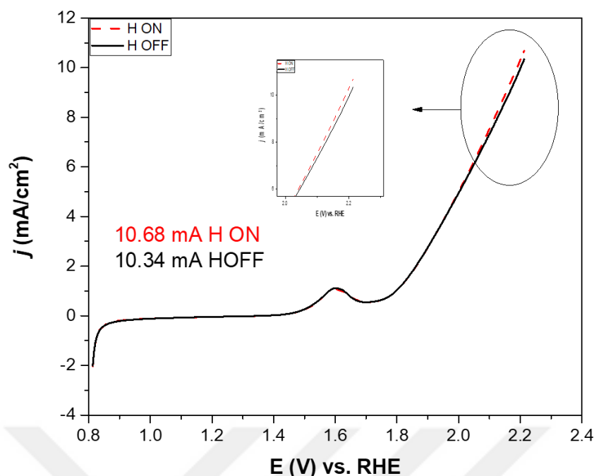
Fig 4. 2 LSV Profile of FTO/[Co-Co] illustrating magnetic enhancement (Inset: Magnified image of the enhancement zone).
