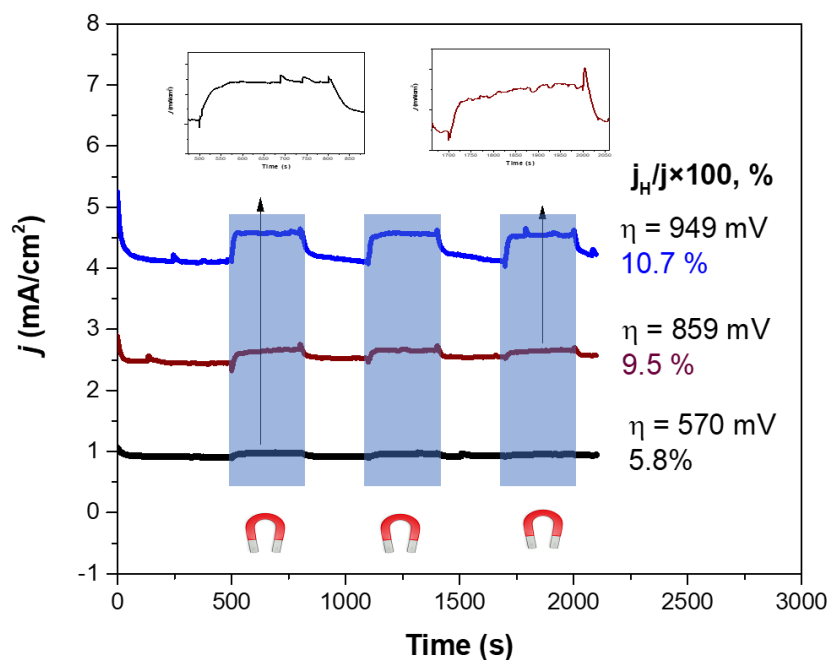
Fig 4. 5 CA Profile obtained for FTO/[Co-Co] at different overpotential (Insets: zoomed images of graphs that are not clear in the main graph).
