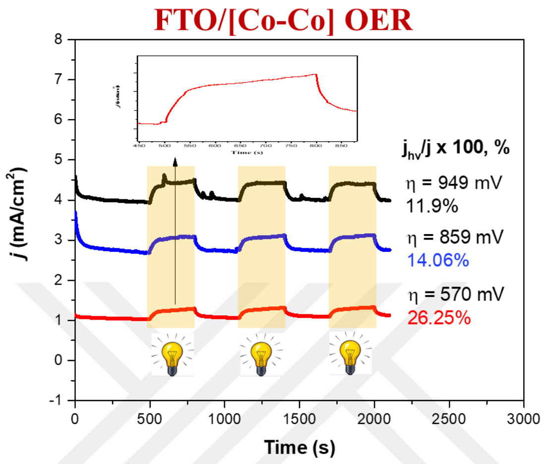
Fig 4. 11 CA Profile of FTO/[Co-Co] illustrating Light enhancement at different overpotentials (inset: Showing the red graph enhancement which is not very prominent in the main graph)
