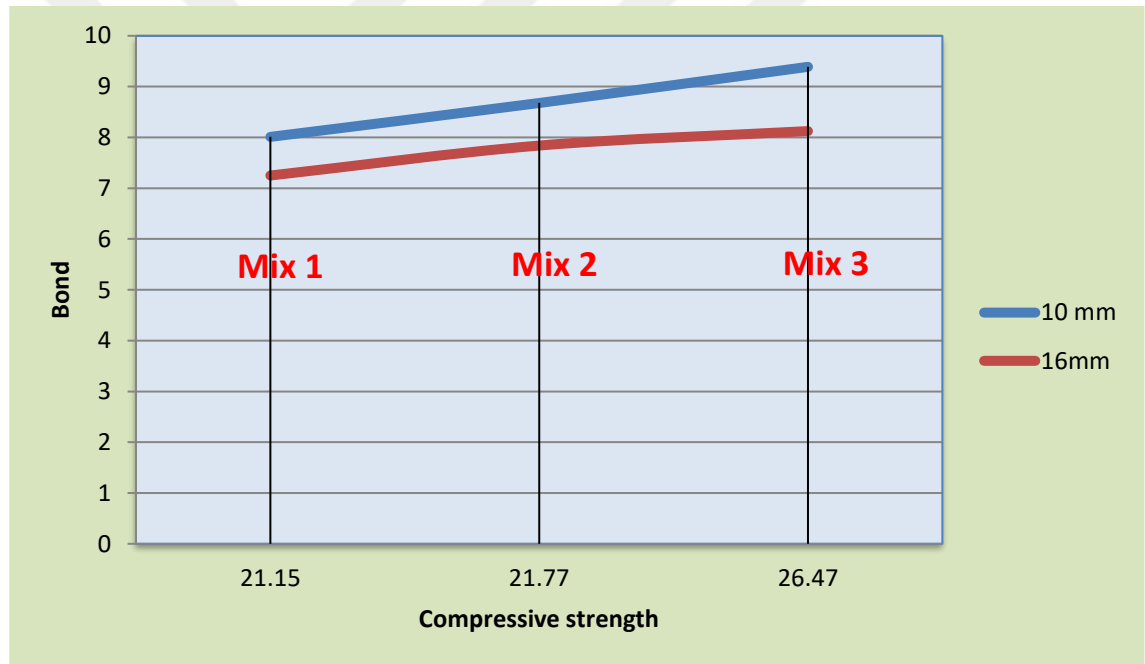
Fig 4.10 Relationship between Bond and compressive strength at age (3) days
