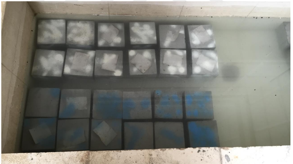
Fig (3.8) photographic all specimens dipped in water
