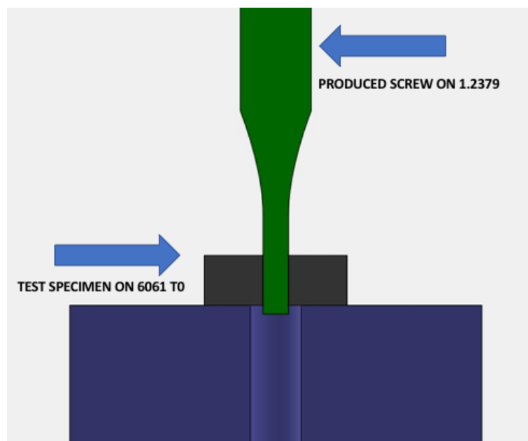
Figure 16 Test Setup Design for Tensile Test
