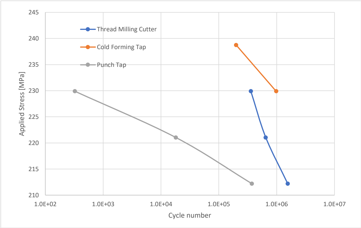
Figure 21 S-N Curve of Three Different Thread Type
