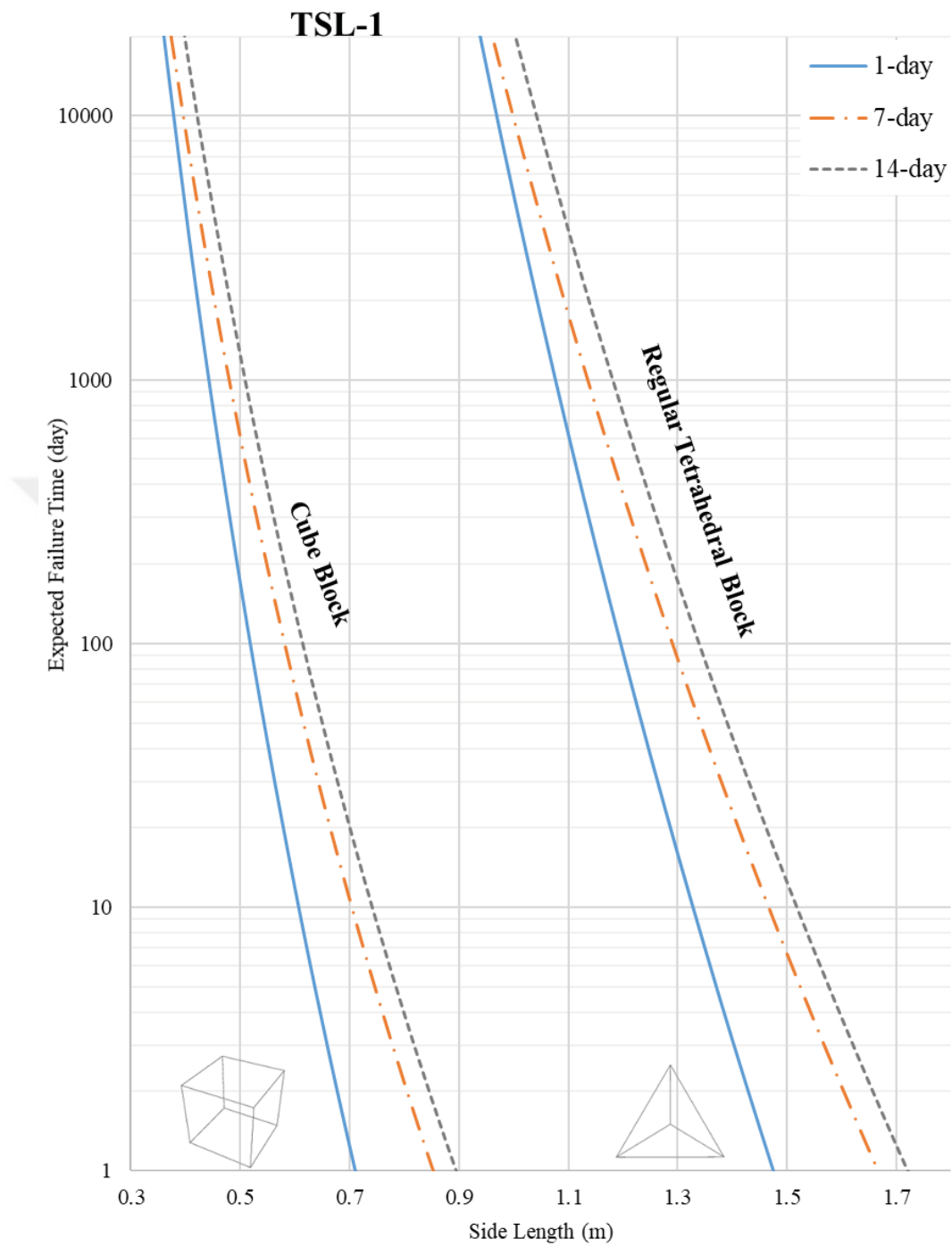
Figure 4.10 Holding time estimation of various wedge block dimensions for TSL-1 (Guner and Ozturk, 2018)
