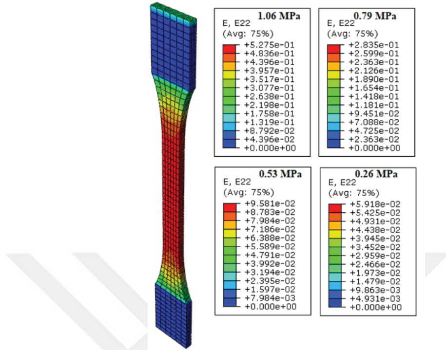
Figure 6.5 Strain distributions at the moment of rupture for TSL-1 (1-day)
