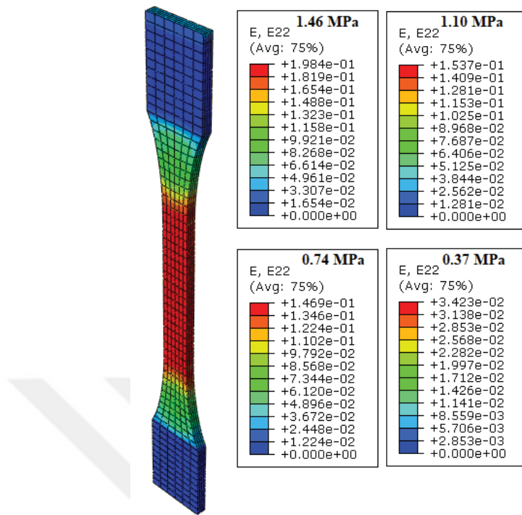
Figure 6.7 Strain distributions at the moment of rupture for TSL-2 (2-day)
