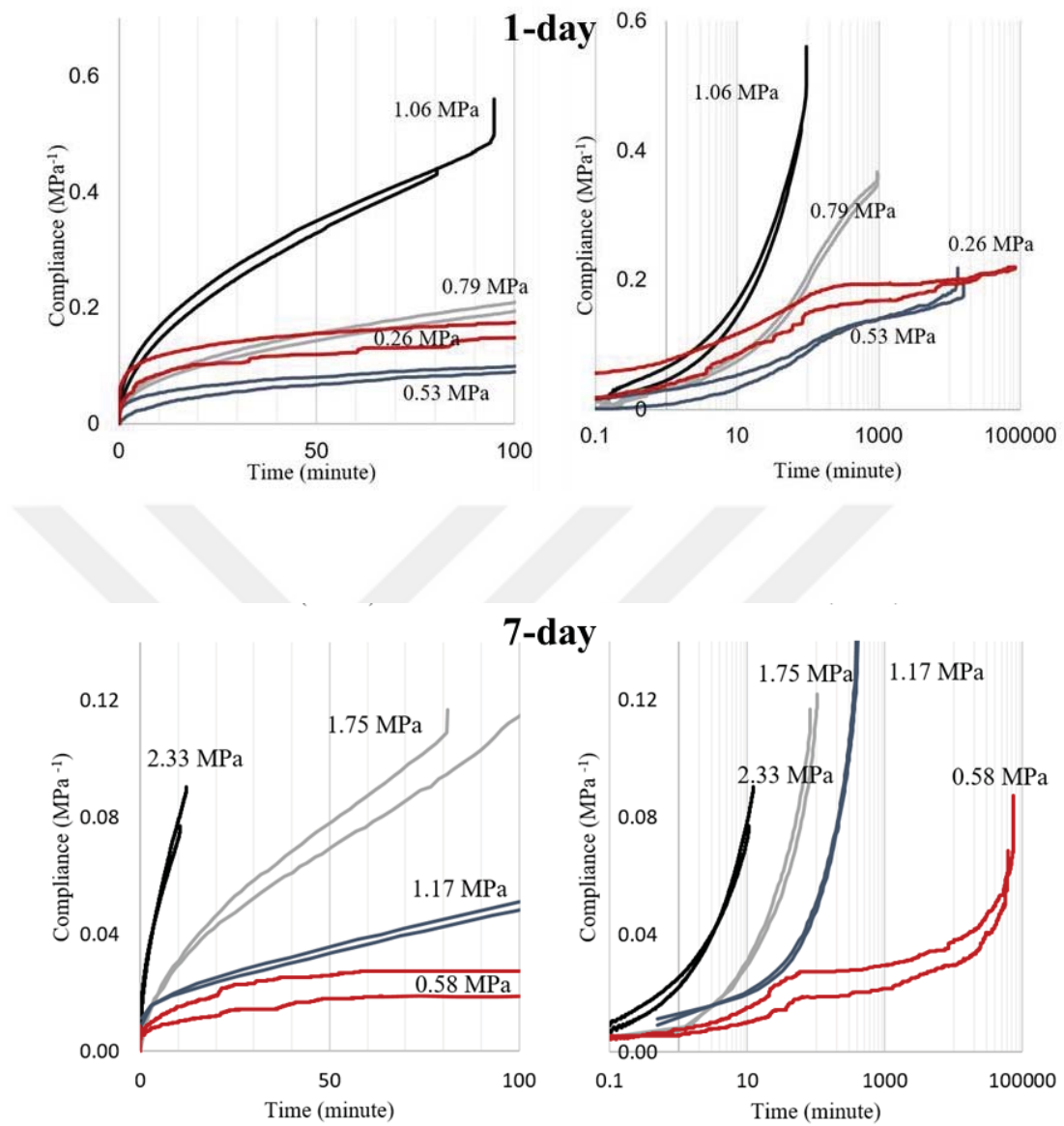
Figure 3.11 Experimental Compliance response of the TSL-1 for 1 and 7 days
