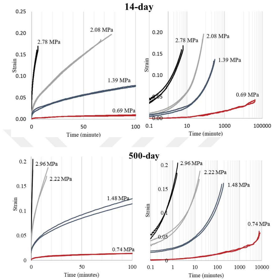
Figure 3.14 Experimental creep response of the TSL-1 for different curing times
