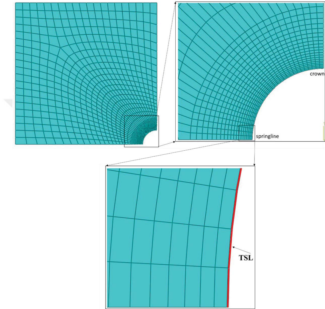
Figure 7.3 Meshing of the model
