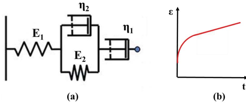
Figure 2.17 Mechanical analogue and strain-time behaviour of the Burger's model
