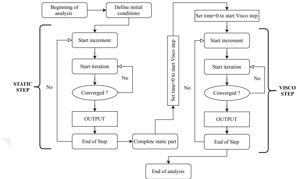
Figure 6.3 Typical workflow for creep analysis in ABAQUS
