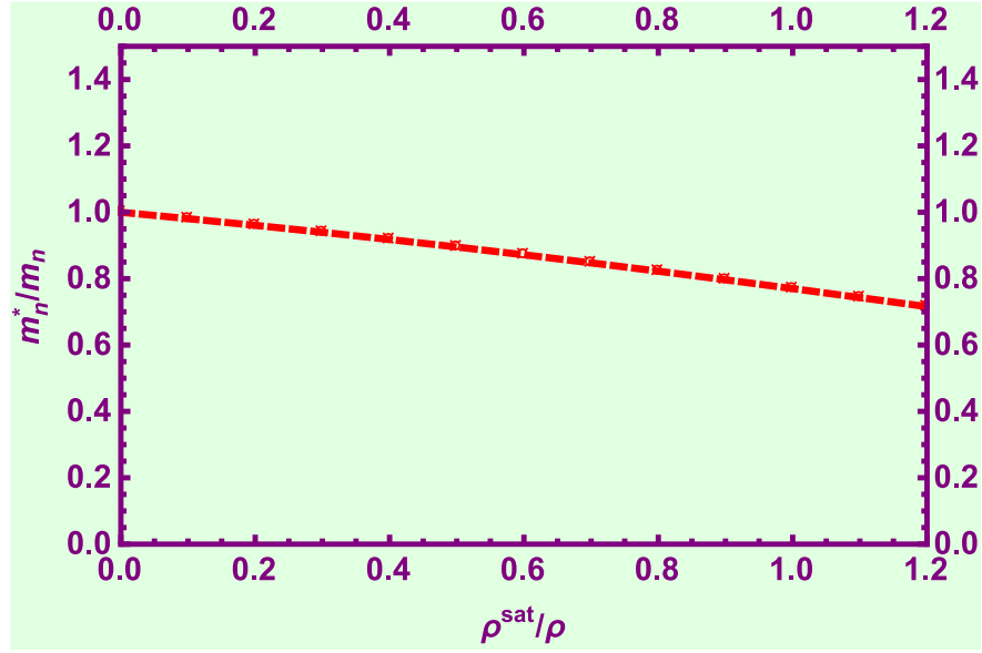
Figure 4.10: Same as Fig. 9 for m_n^*/m_m .
