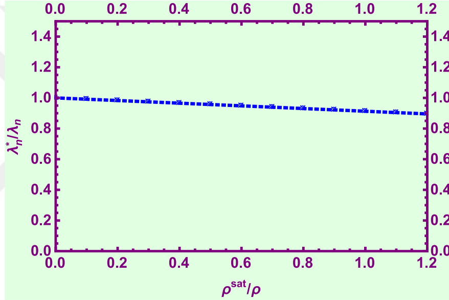
Figure 4.9: \lambda_n^* / \lambda_n as a function of \rho^{\text{sat}} / \rho at s_0^* = 1 \text{ GeV}^2 , M^2 = 1 \text{ GeV}^2 and x = -0.65 .
