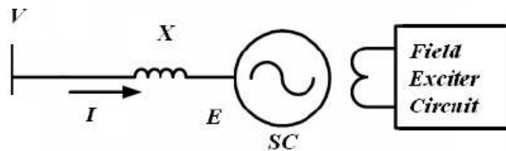
Figure 2.8 Synchronous Compensator
