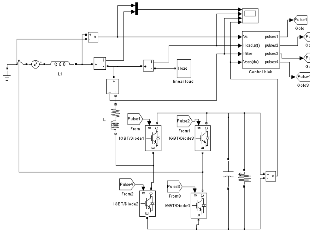
Figure 4.6 Voltage source converter with controller
