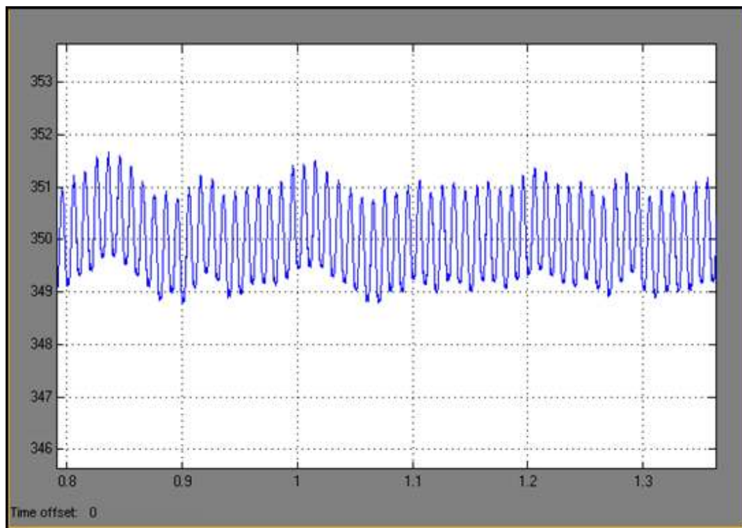
Figure 4.31 DC link voltage ripple ( V_{DC,ripple} )
