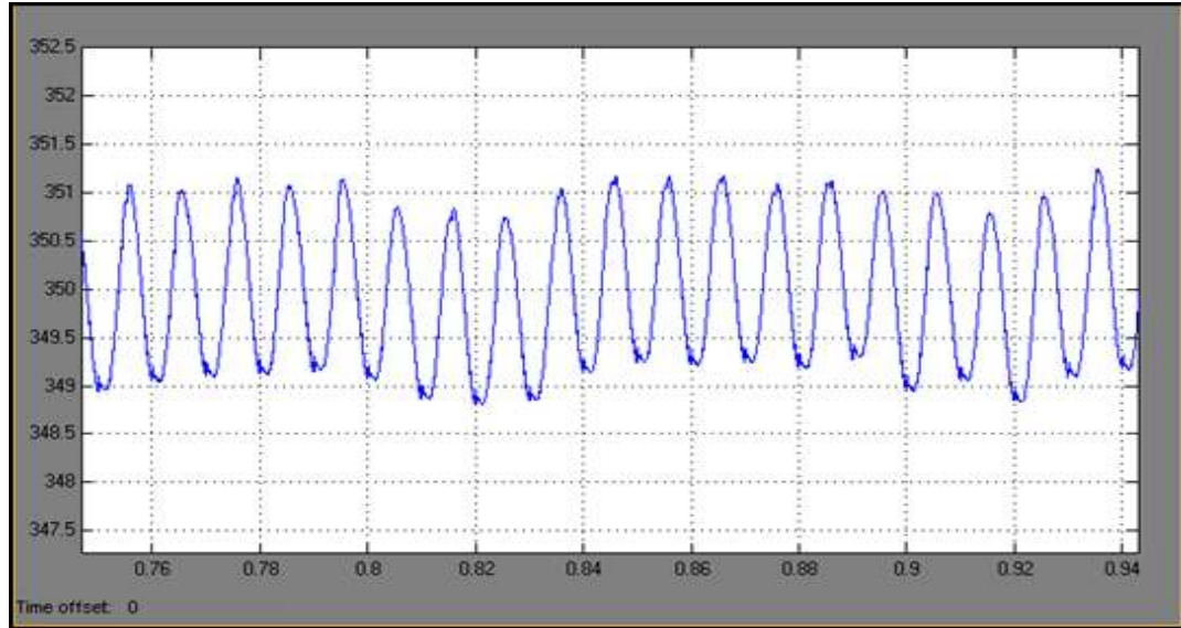
Figure 4.19 DC link voltage ripple ( V_{DC,ripple} )
