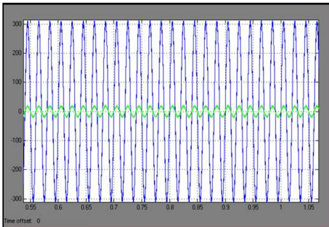
Figure 4.27 Supply current ( i_s ) and supply voltage ( v_s ) (After compensation)
