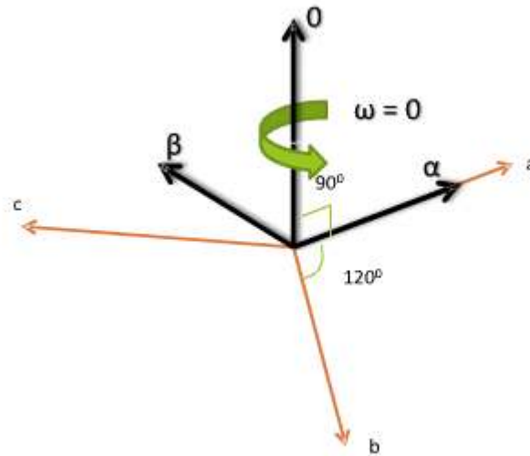
Figure 3.3 The abc to \alpha\beta 0 transformation
