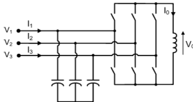
Figure 2.9 CSC topology
