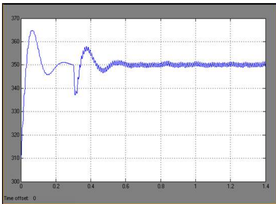
Figure 4.30 DC link voltage ( V_{DC} )
