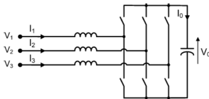
Figure 2.10 VSC topology
