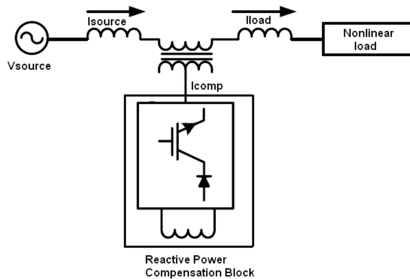
Figure 2.2 Series connection
