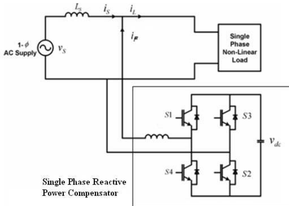
Figure 4.1 Single phase voltage source inverter
