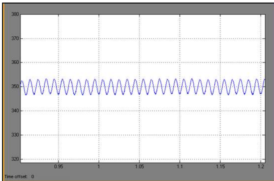
Figure 4.11 DC link voltage ripple ( V_{DC,ripple} )
