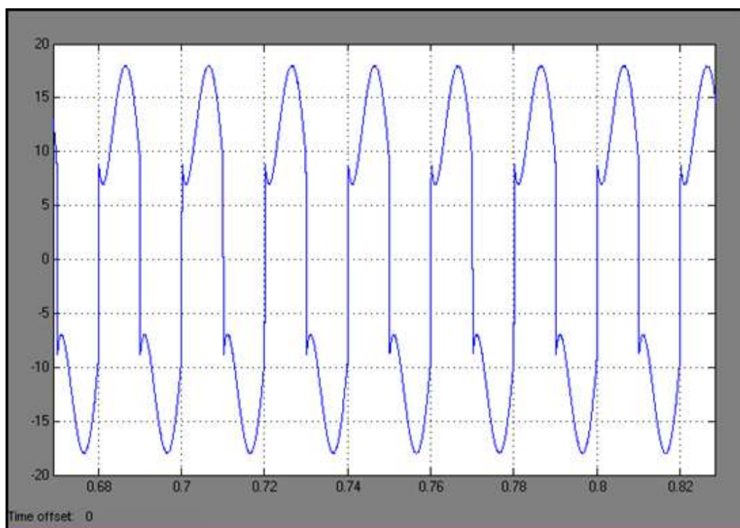
Figure 4.28 Load current ( i_L )
