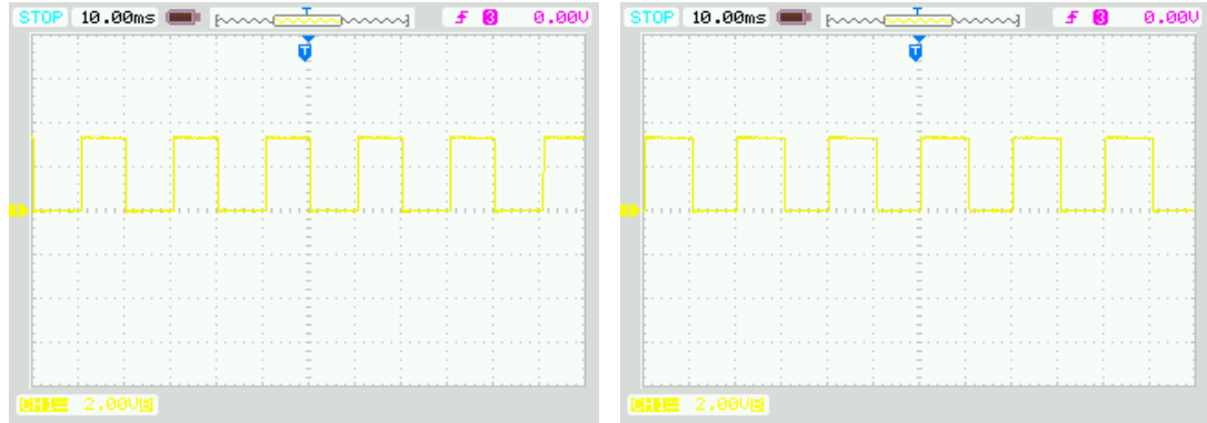
Figure 5.14 Gate signals at DSP output ports
