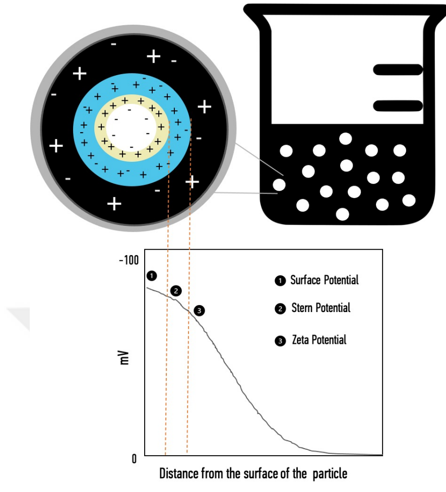
Figure 1 Illustration of the electric double layer, Stern potential, diffuse potential, and Zeta potential
