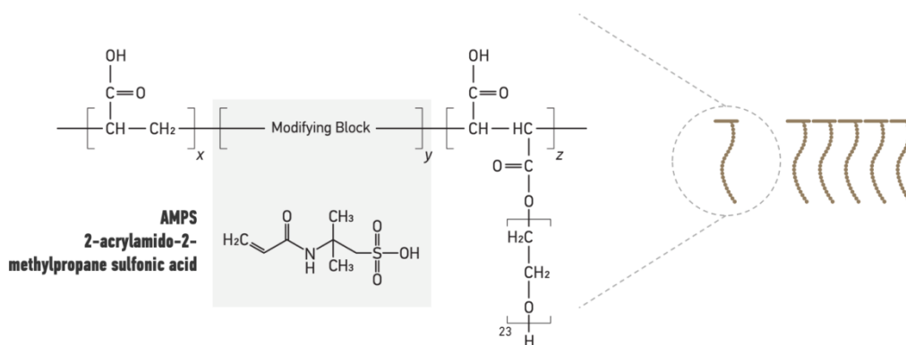
Figure 2 Chemical structure of the grafted copolymers
