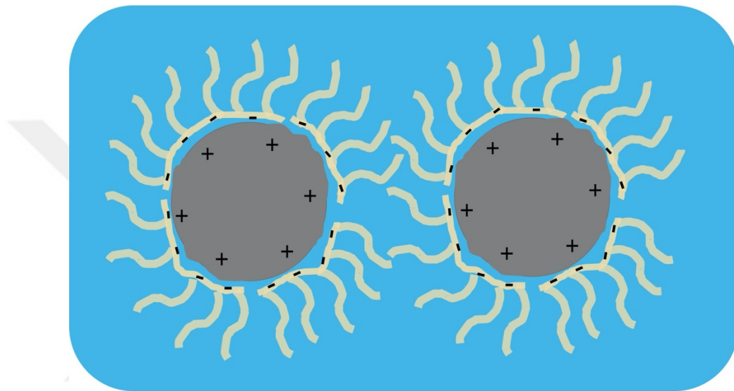
Figure 3 Electrostatic repulsion and steric hindrance mechanism of the grafted copolymer with the cement particles below 1.5 wt. %
