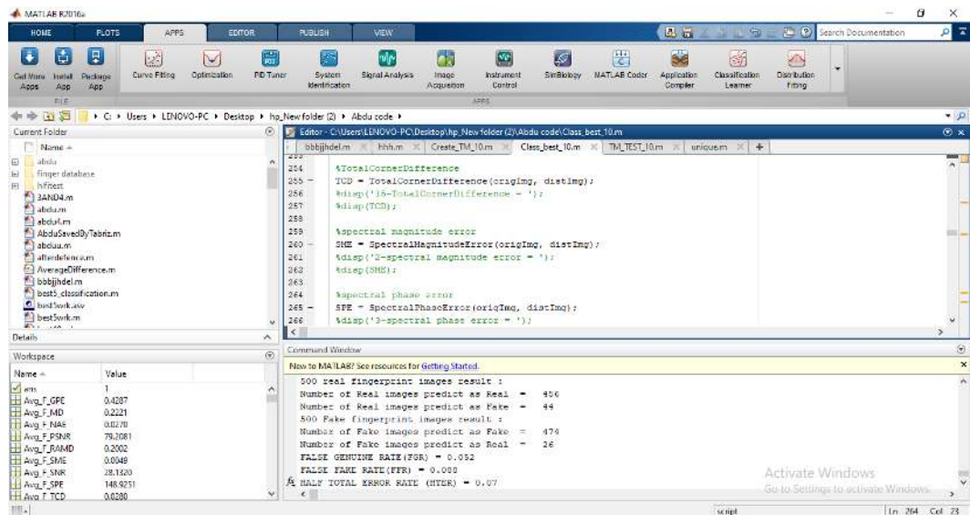
Figure 62: Logistic Regression classification result of 1000 fingerprint images using 10 IQMs.
