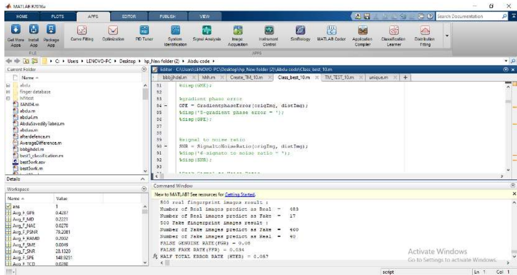
Figure 61: Fine KNN classification result of 1000 fingerprint images using 10 IQMs.
