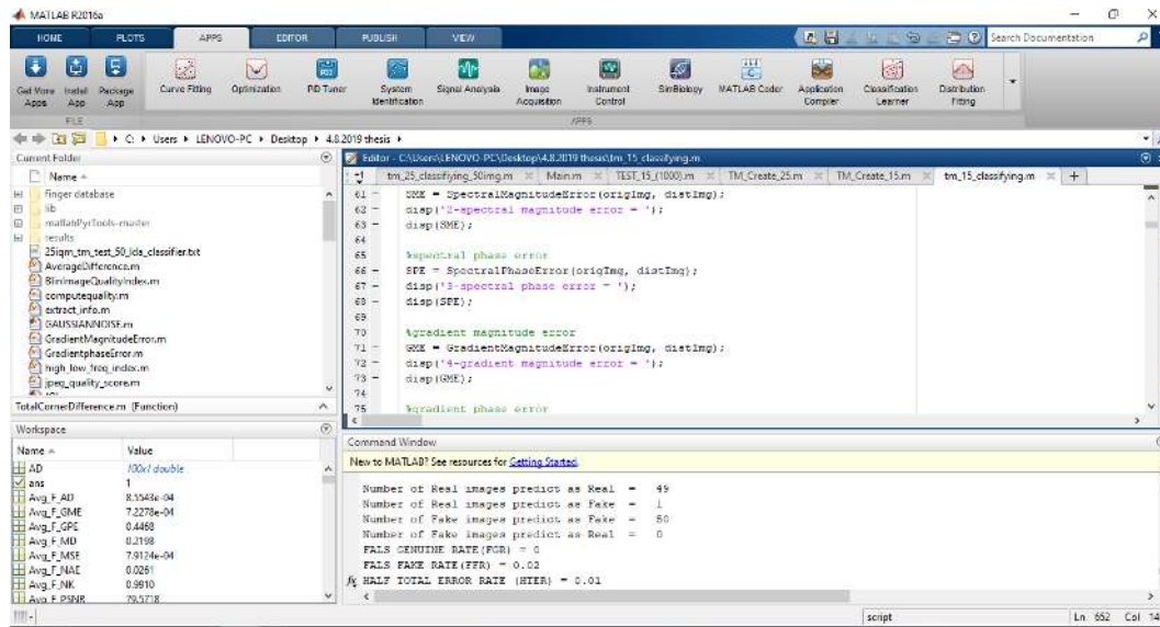
Figure 40: QDA training result of 100 fingerprint images using 15 IQMs.
