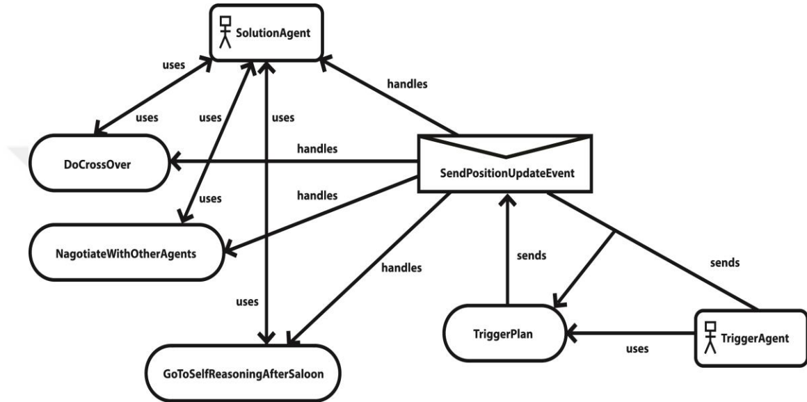
Figure 4.21 General overview of negotiation and next move mechanism
