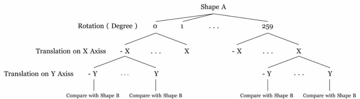
Figure 2.2 State space search for the transformation determination between Shape-A and Shape-B is given. “X” and “Y” are the number of columns and rows of the matrix presenting the shapes respectively.
