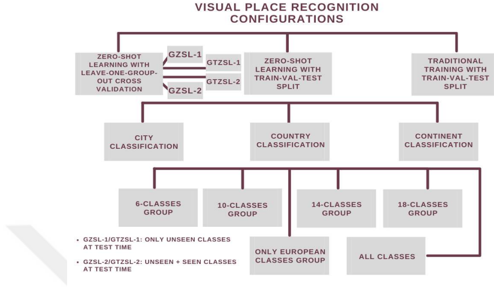
Figure 3.15. Summary of the experimented different techniques throughout the study
