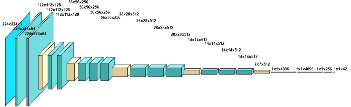
Figure 3.6. Main layers of the model architecture used for traditional training configuration
