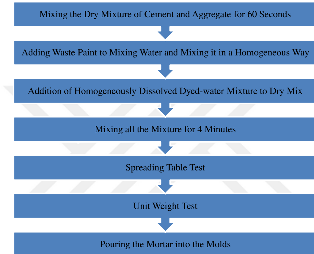
Figure 3.1: Sequence followed in production
