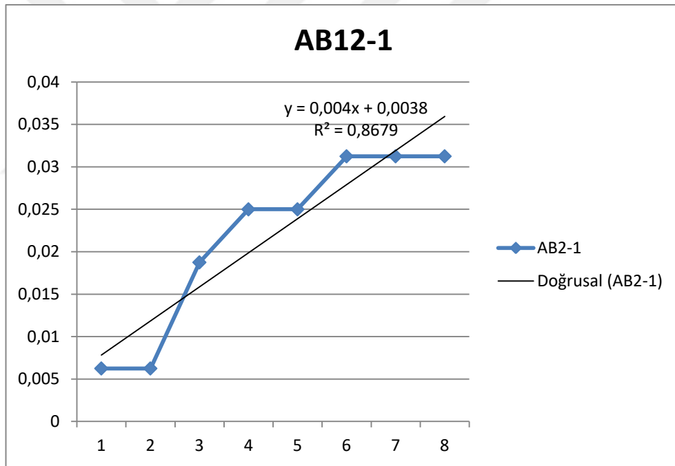
Figure B.5: Capillary Water Absorption-Time Graph in AB12-1 Latex Paint Additive Sample
