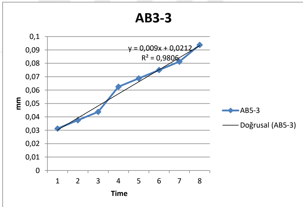
Figure B.15: Capillary Water Absorption-Time Graph in AB3-3 Solvent Dye Additive Sample
