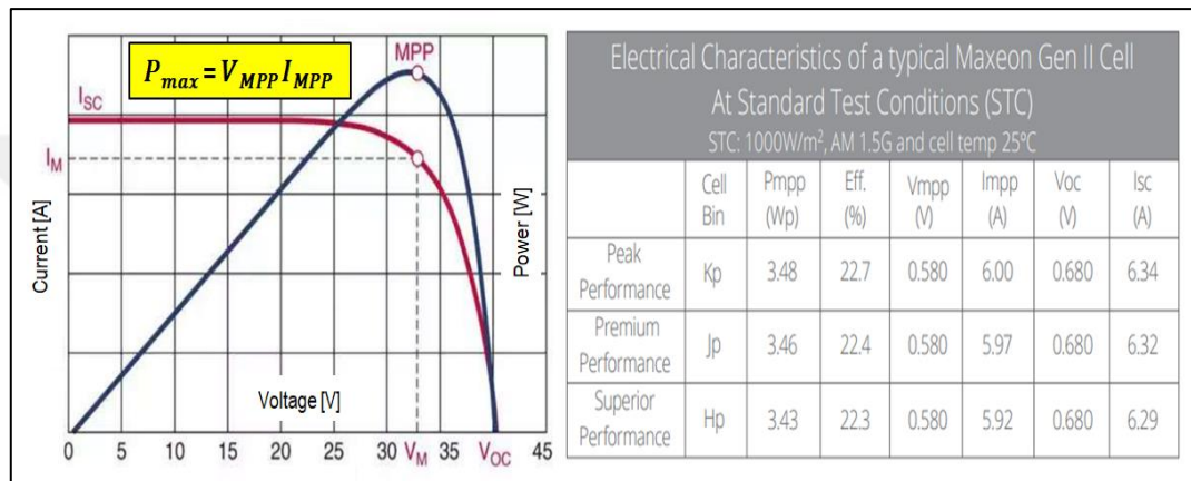
Figure 3.3 Characteristic Graphic of Current to Voltage Curve
