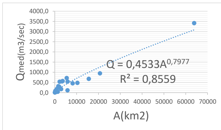
Figure 10.6. Relationship between area and flow for first region of Fırat basin
