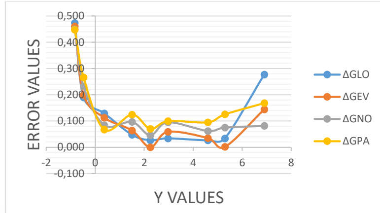
Figure 10.8. Relationship between y and the error values for each of the distributions
