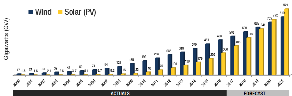
Figure 1.6 Solar and Wind Installed Capacity (fi-powerweb.com, 2019)
