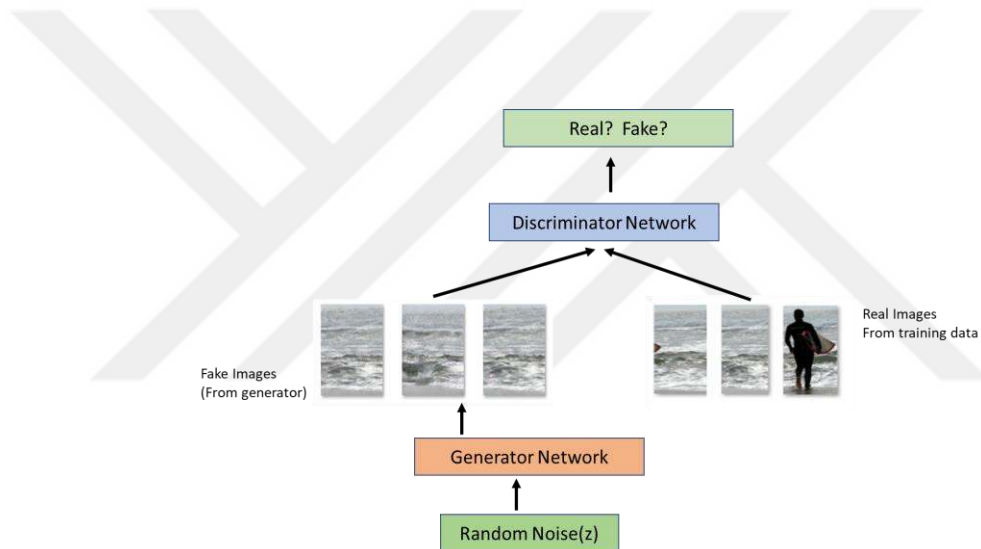
Figure 4.8: Discriminator and generator produce new images that are like the images in the model training set. (Image from COCO dataset)
