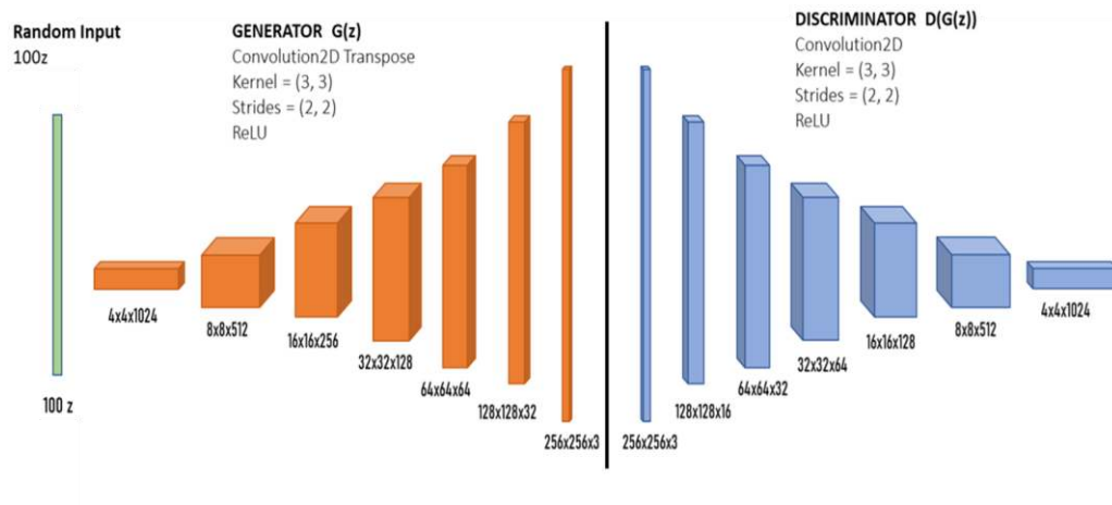
Figure 4.7: GAN model used, the illustration of up-sampling (Convolution2D Transpose) and down-sampling (Convolution2D).
