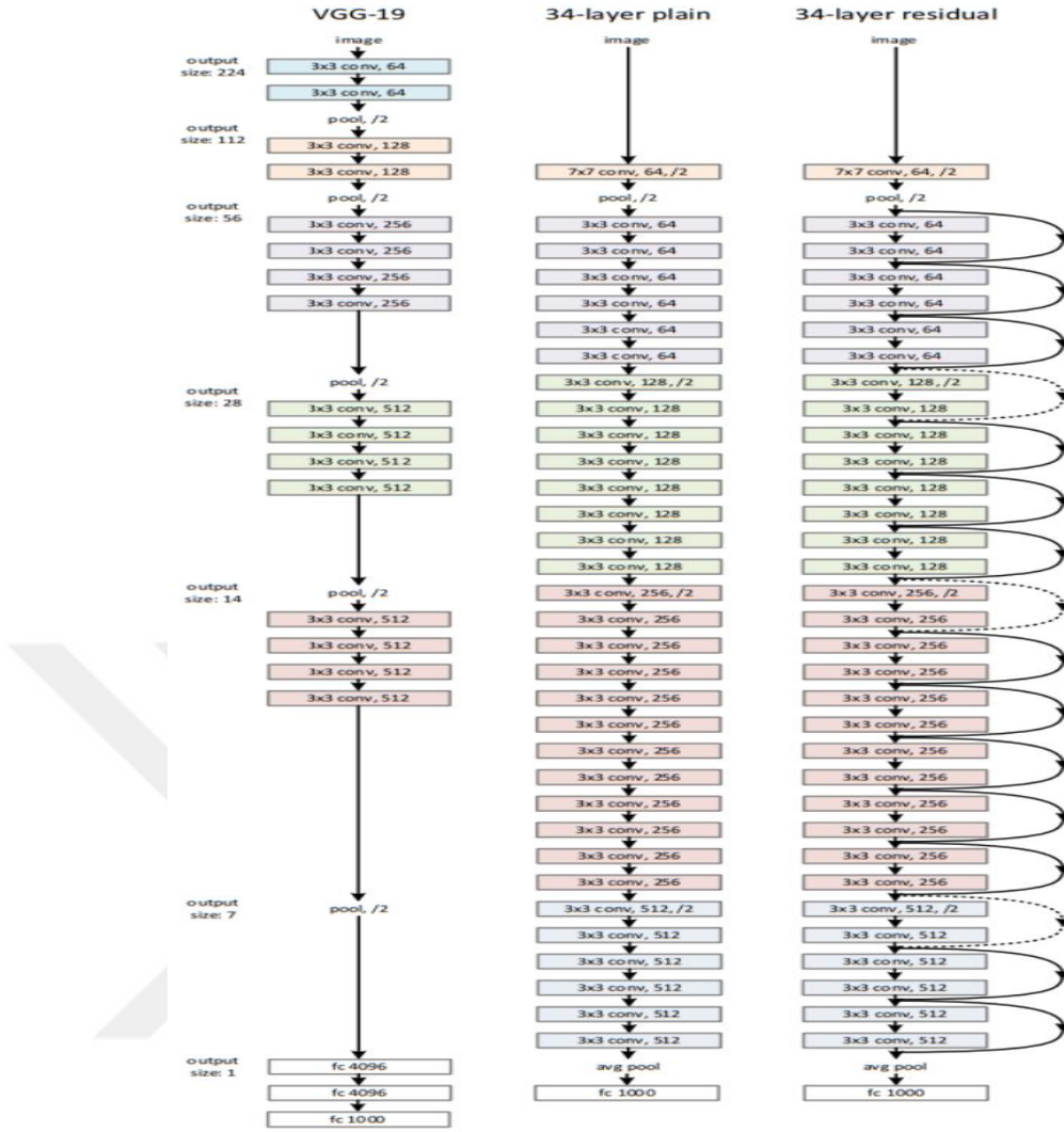
Figure 4.3: Resnet architecture with 34-layer residual [80].
