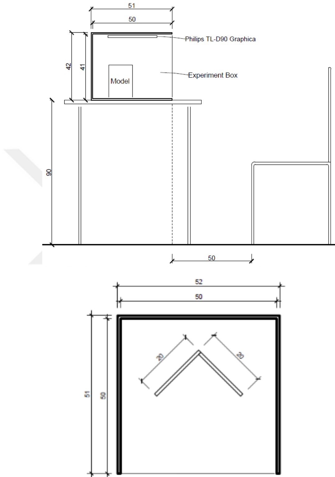
Figure 23. Drawings of the experiment box (side view and top view)
