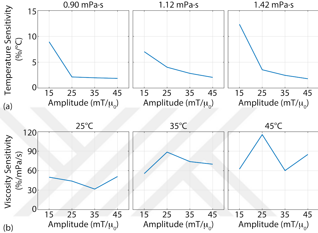
Figure 6.6: The estimated sensitivities for temperature and viscosity at four different drive field amplitudes at 9.8 kHz. (a) The temperature sensitivity is highest at 15 mT/μ₀ with a value of approximately 10%/°C and decreases as the amplitude increases. (b) The viscosity sensitivities are very similar between different amplitudes, and increase with temperature. The viscosity sensitivity at 25°C is around 40%/mPa/s on average, and almost doubles at 45°C to values around 85%/mPa/s on average.
