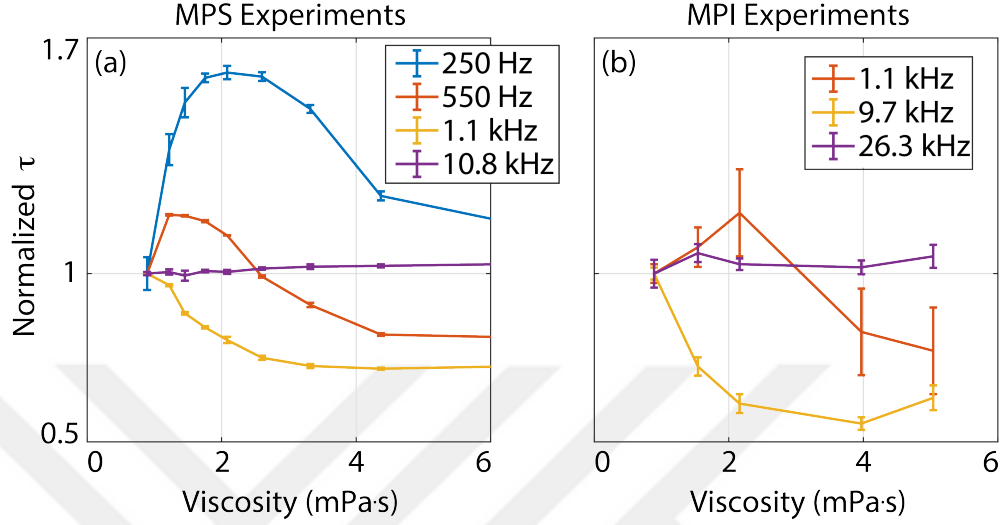
Figure 4.3: Comparison of \tau vs. viscosity curves for (a) MPS experiments (re-plotted from Ref. [60]) and (b) color MPI experiments, performed at different drive field frequencies at a 15 mT/ \mu_0 amplitude. The results are color matched to highlight similar trends. A monotonic \tau vs. viscosity curve is observed at 1.1 kHz in MPS experiments, whereas a similar trend is achieved at 9.7 kHz with the additional selection field of the MPI scanner.
