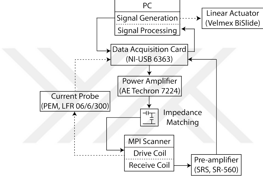
Figure 3.5: The overall signal flow for the MPI scanner. The straight lines show the main signal flow, and the dashed lines show the control of equipment used for the field calibration and the motion of the object. Copyright © 2017, IEEE.
