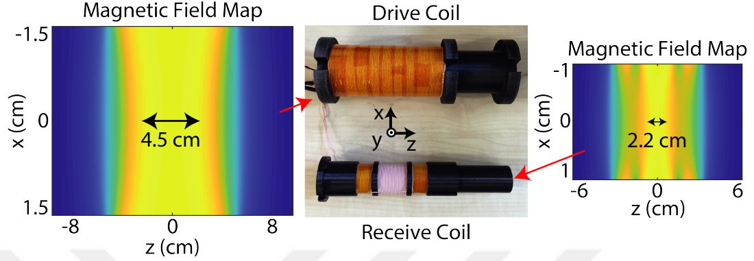
Figure 3.2: The drive and receive coils, and their simulated magnetic field maps in x-z planes. The homogeneous length of the drive field is 4.5 cm within 95% of its maximum value, and the sensitive region of the receive coil drops to its 75% within 2.2 cm. Copyright © 2017, IEEE.
