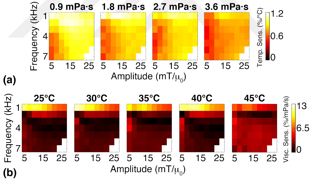
Figure 5.7: The estimated temperature and viscosity sensitivities at all operating points displayed as color maps. (a) The temperature sensitivities (in \%/^{\circ}\text{C} ) at 4 different viscosity levels change relatively slowly across different operating points, reaching the highest values of >1 \%/^{\circ}\text{C} at high-amplitude operating points. (b) The viscosity sensitivities (in \%/m\text{Pa/s} ) at 5 different temperatures show a drastic change as a function of drive field frequency, reaching the highest values of >10 \%/m\text{Pa/s} at low frequencies around 1 kHz.
