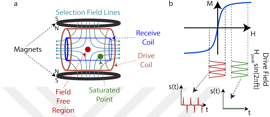
Figure 2.2: (a) An MPI scanner schematic is shown with the static selection field created by magnets with north poles facing each other. The selection field distribution creates a field free region in the middle, and other points in this configuration have a DC magnetic field that typically exceeds H_{sat} . (b) Once a sinusoidal drive field is applied on top of this configuration, only the SPIONs in the field free region will induce signal in the receive coil, and the SPIONs in the saturated regions can not further increase their magnetic moments, and hence, do not have any contribution to the received signal.
