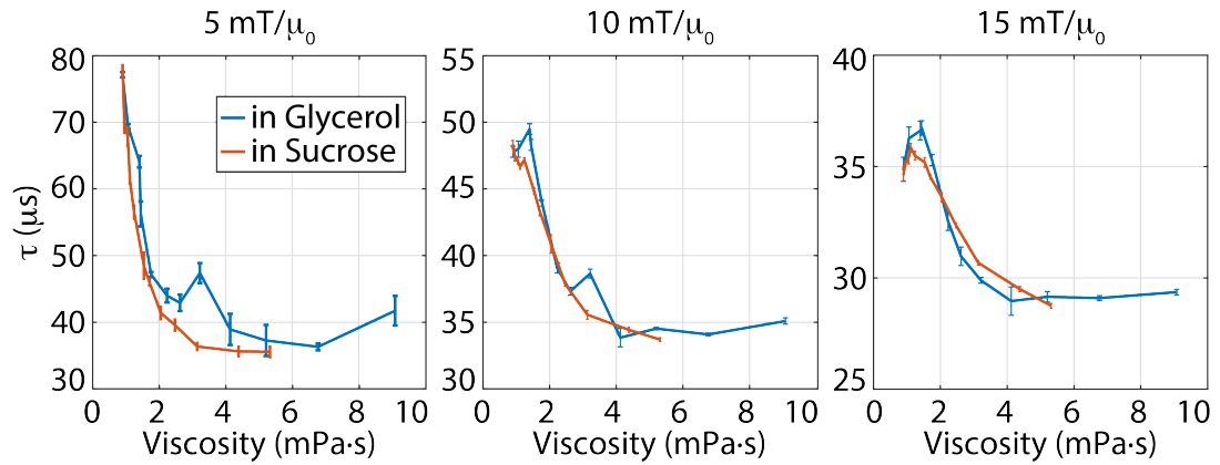
Figure 2.8: The estimated time constant vs. viscosity curves for 11 different glycerol/water mixtures and sucrose/water solutions measured at 1.1 kHz and three different drive field amplitudes: 5 \text{ mT}/\mu_0 , 10 \text{ mT}/\mu_0 , and 15 \text{ mT}/\mu_0 .
