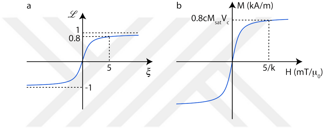
Figure 2.1: (a) The Langevin function given in Equation 2.1 is plotted. Here, the saturation is defined as reaching to 80% of the maximum value [118]. (b) The nonlinear magnetization characteristics of SPIONs are described by the Langevin function, which is weighted with the concentration, c , saturation magnetic moment, M_{sat} , and core volume, V_c , of the SPION. The magnetic moments of SPIONs are fully driven by the applied field when the applied magnetic energy exceeds the internal thermal energy of SPIONs.
