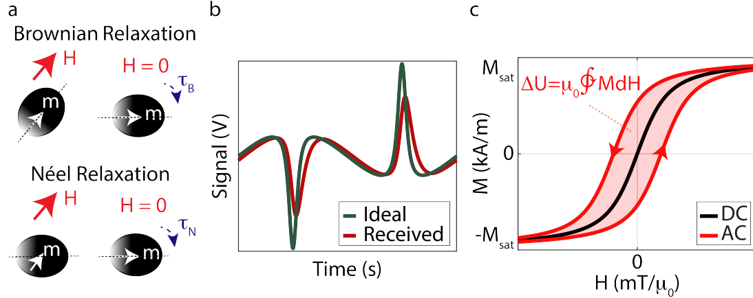
Figure 2.3: (a) Brownian relaxation (i.e., physical rotation) and Néel relaxation (i.e., internal rotation) describes the zero-field relaxation behaviors of the SPIONs. (b) The time-domain SPION response to an AC magnetic field is shown for two cases: The ideal signal with an adiabatic approximation that does not have any relaxation effects, and the actual received signal with the relaxation effects. (c) The magnetization curves of the SPIONs under DC and AC magnetic fields are shown. A hysteresis loop is observed in the AC case where the red shaded area corresponds to the magnetic work done on the SPIONs ( \Delta U ) that result in heat dissipation.
