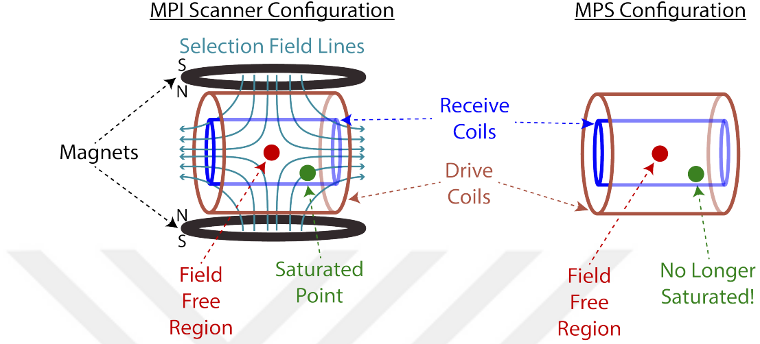
Figure 2.5: The schematic comparison of an MPI scanner (left) and an MPS setup (right) is shown. Here, the only difference between the two setups is the permanent magnets that generate the selection field for spatial encoding. In the MPS case, the SPION samples in the whole measurement chamber induce response in the receive coil, enabling the characterization of the SPION response.
