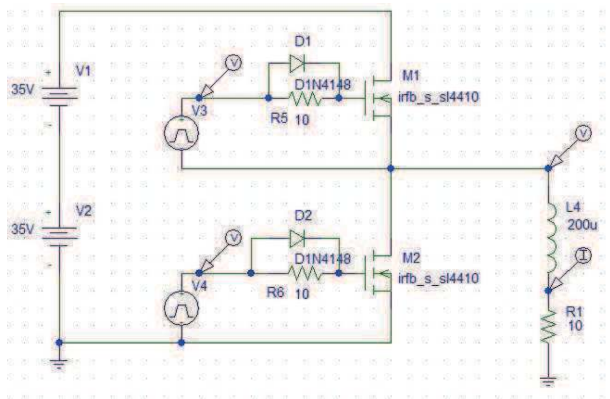
Figure 3.1 Basic half - bridge inverter circuit with MOSFETs IRFS4410
