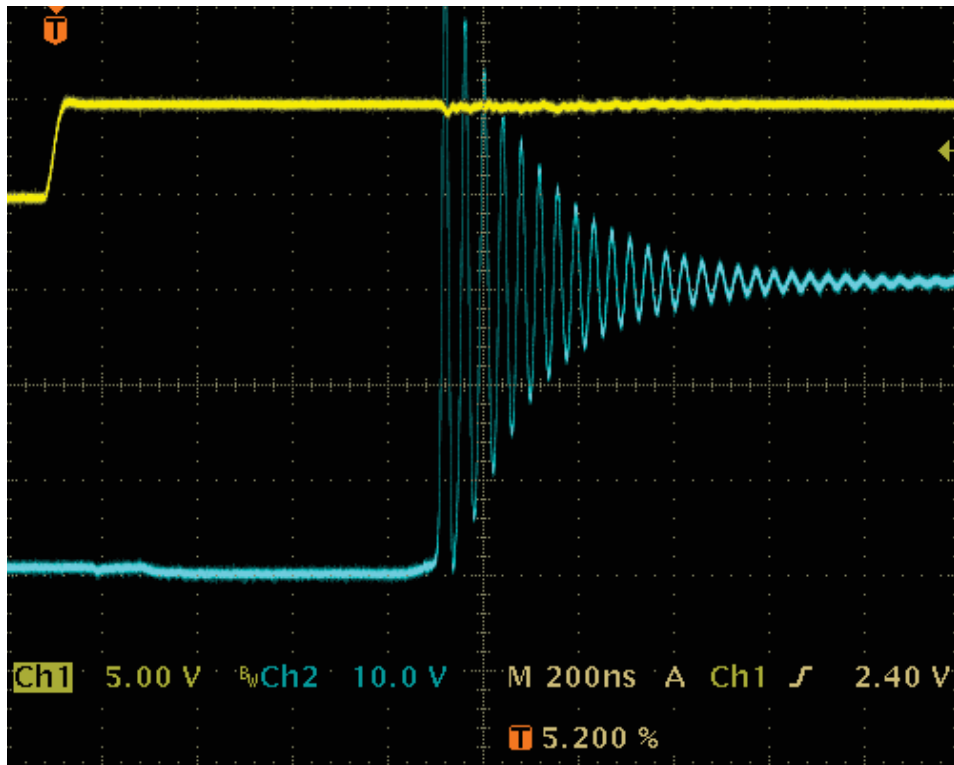
Figure 5.8 Switch - Off MOSFET drain voltage waveform
