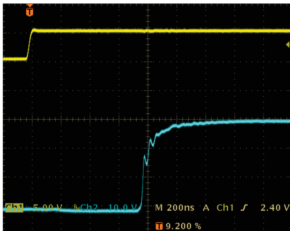
Figure 5.10 Switch - Off MOSFET drain voltage waveform after addition of RC snubber
